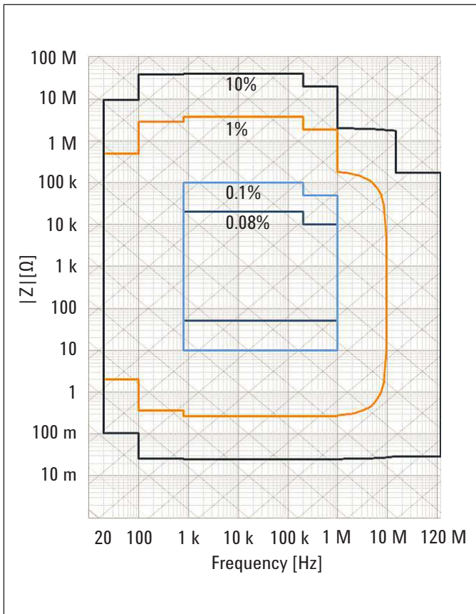
10% impedance measurement accuracy range at Four-terminal-pair of E4990A's Front Panel (Test signal level = 0.5 Vrms, measurement Time = 5)
