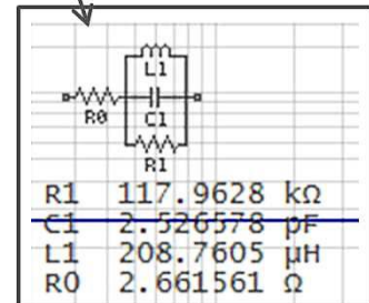
Equivalent parameters for a low inductor (F circuit is used)
