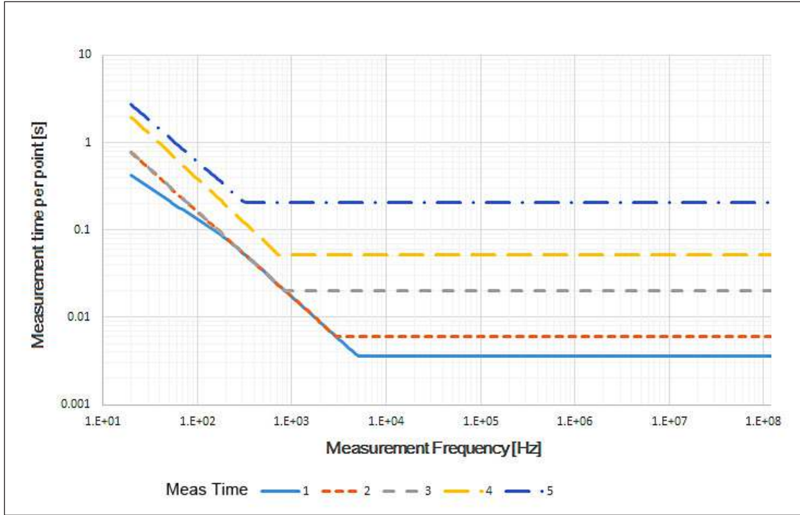
Figure 2. Measurement time (Option 120, adapter: None, 1 m, 2m, Typical)
