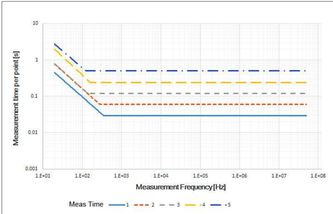
Figure 4. Measurement time (Option 050/030/020/010, Typical)
