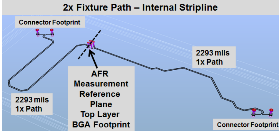
Figure 8: The full 1x fixture path including the cable and the PCB inner layer differential pair stripline routing can be measured using the 2x Fixture Through path with the reference plane located at the top layer BGA via pads. Implementing an additional 2x Fixture path with 1 inch added to each side for a 1x fixture length of 3293 mils enables measurement of material properties and simulated fixture data for the remaining DUT fixture paths.
