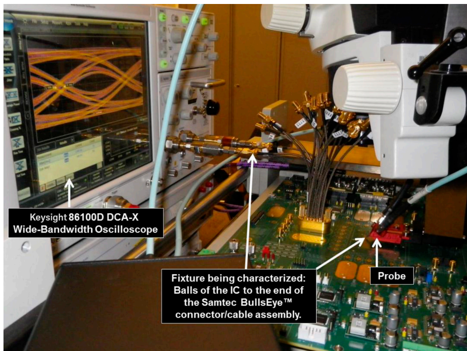
Figure 11: A probe station was used to launch a reference signal onto the high speed channel fixture using a probe, and the signal at the output of the fixture was then analyzed using a wide-bandwidth oscilloscope.
