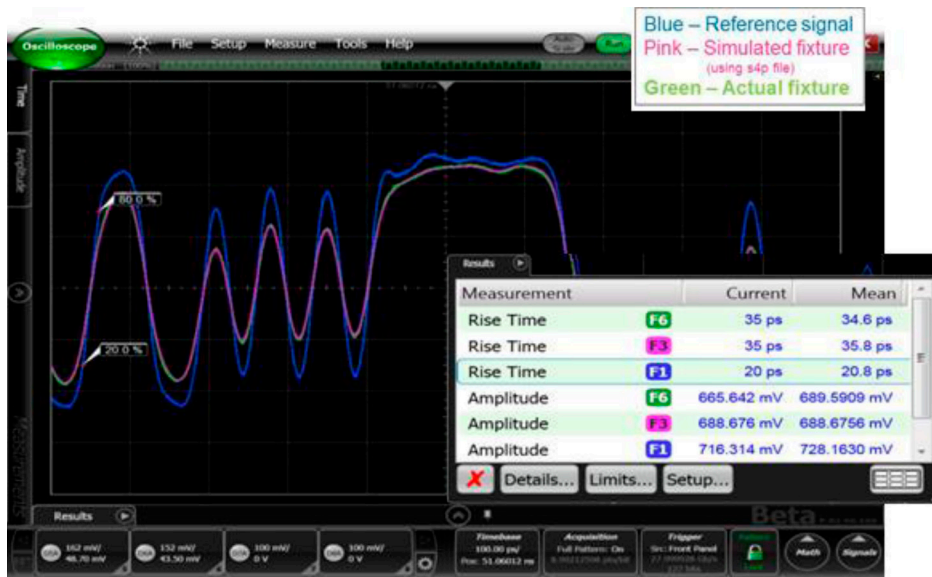
Figure 20: Comparison of waveforms from simulated fixture (F3 pink) and actual fixture (F6 green) showing excellent correlation.
