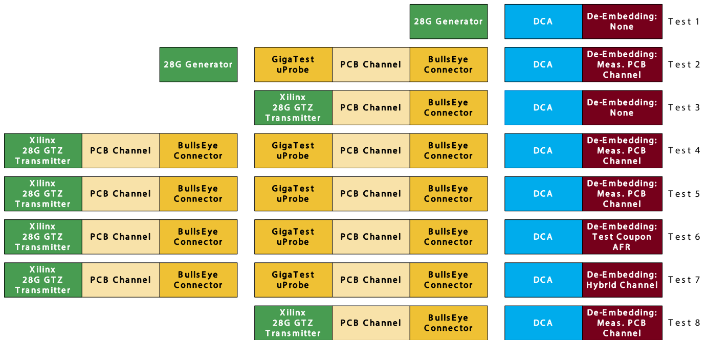
Figure 5: Planned measurements for verification of fixture de-embedding methodology.
