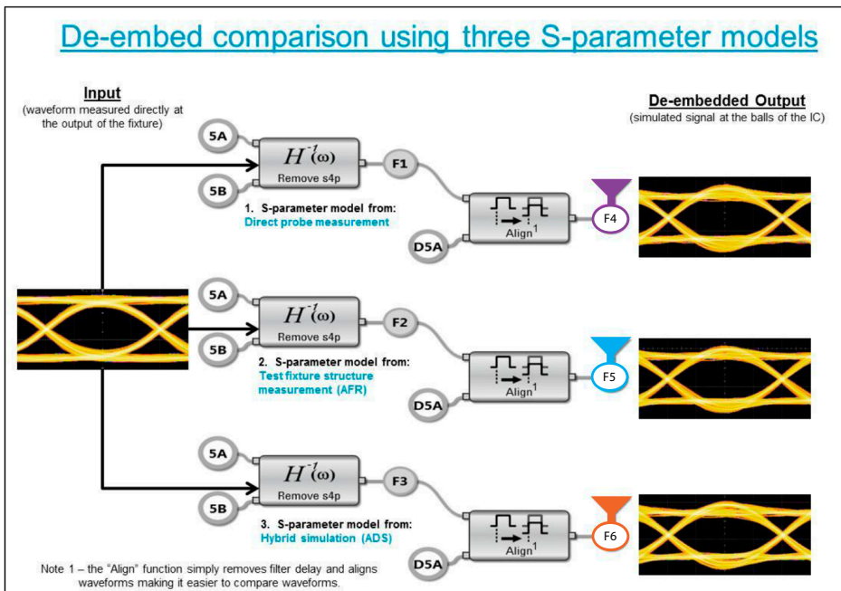
Figure 31 – Graphical representation of the signal processing setup used to compare the de-embedded signals (the same input signal is processed by three different S-parameter models)
