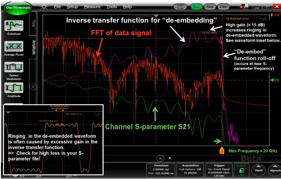
Figure 15: Frequency plot showing S21(green), inverse S21 function(purple), overlaid with the FFT of the data signal (orange). Attempting to de-embed too much loss often results in ringing in the de-embedded waveform (lower left).
