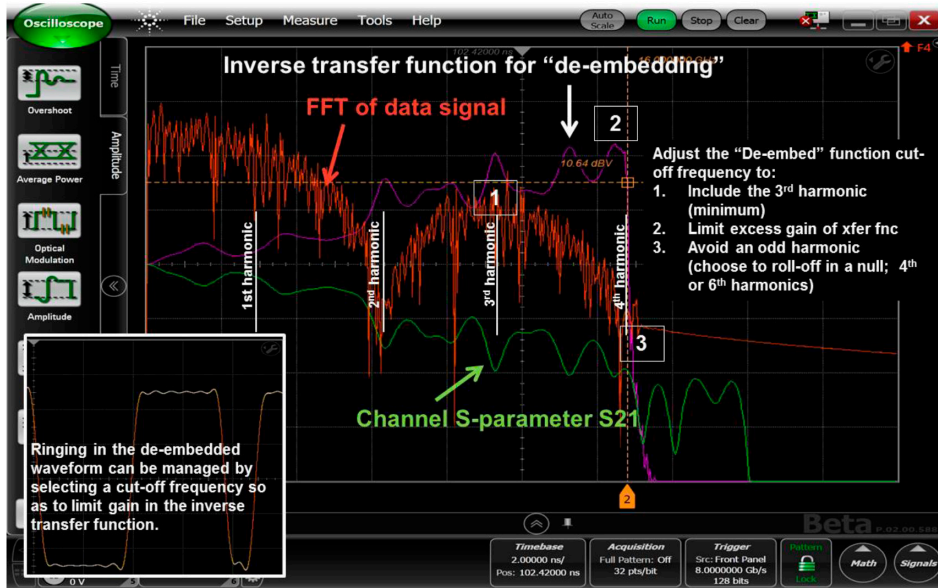
Figure 16: Frequency plot showing the cut-off frequency for a de-embed function (top trace) which has been optimized to minimize ringing in de-embedded waveform.
