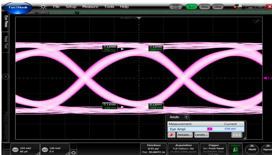
Figure 18: Predicted eye diagram at the output of the fixture (F3 pink).
