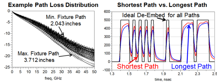
Figure 10: The measurement based hybrid model of the fixture path quickly simulates all of the possible paths on a given PCB layer as shown in the plot on the left. The plot on the right shows the variation in bit shape between the longest path and the shortest path and the ideal source input bit pattern that is desired after fixture de-embedding
