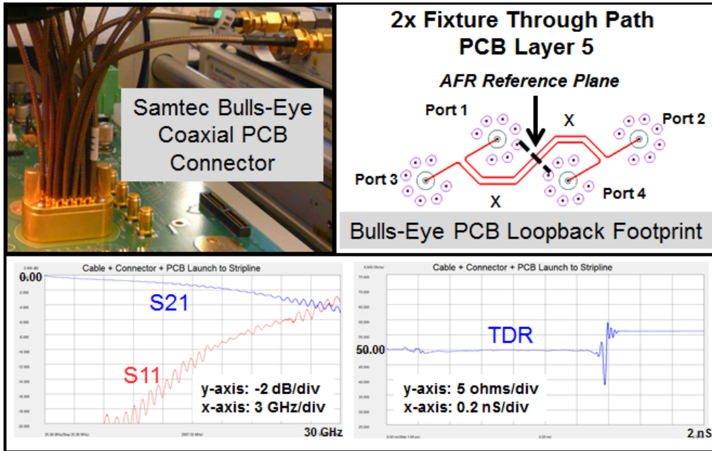
Figure 7: The 1x path length fixture data for the coaxial cable connection to the PCB can be measured using a 2x symmetrical through AFR calibration to split the 2x through path in half and get the S-Parameters for each cable connection to the PCB inner layer. This also provides a quick verification of cable performance in the event a cable is suspected of being damaged through mating and de-mating cycles.
