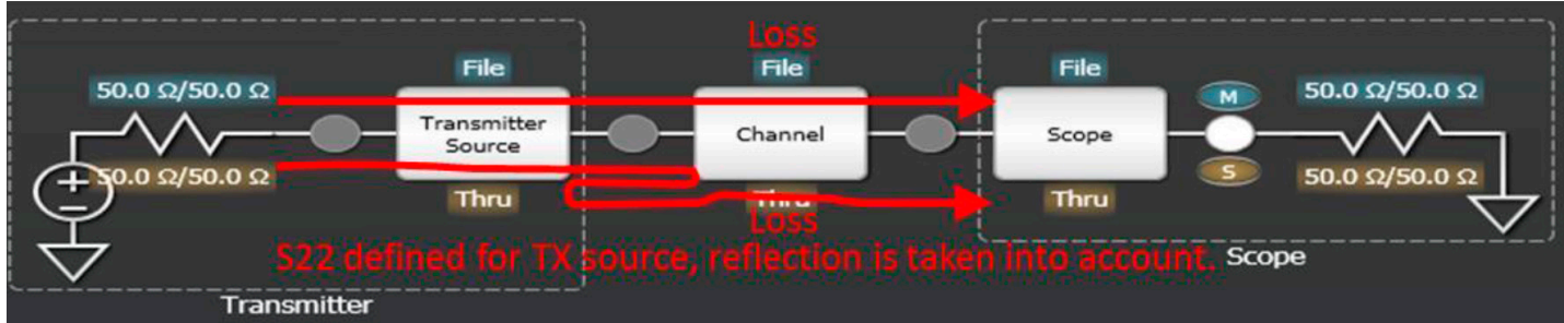
Figure 13: Full de-embedding: If the output impedance of the DUT (left) has been measured and electrical lengths of all circuit elements are accurately known, true de-embedding techniques can yield more accurate results.
