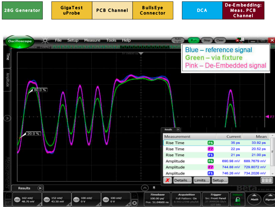
Figure 22: De-embedded signal (F7 pink) compared to reference trace (F1 blue) showing good correlation and provides further model validation.
