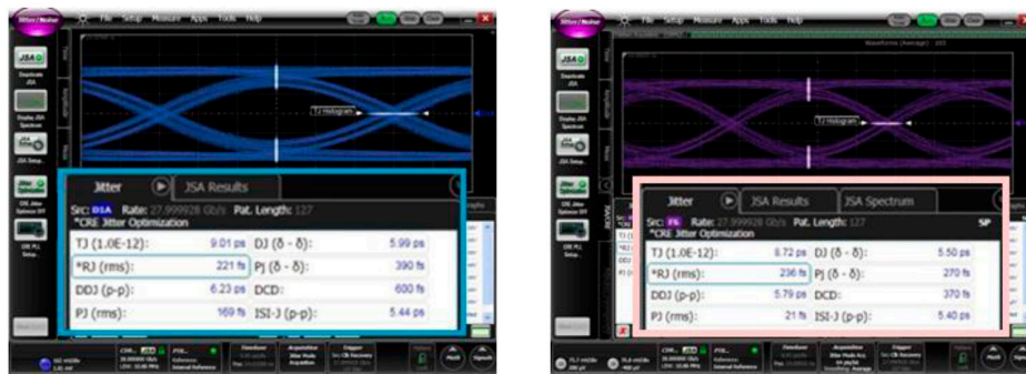
Figure 23: Jitter measurement comparison of de-embedded signal and reference signal; good ISI correlation (both measured and de-embedded signals are 5.4ps) which further validates the model.
