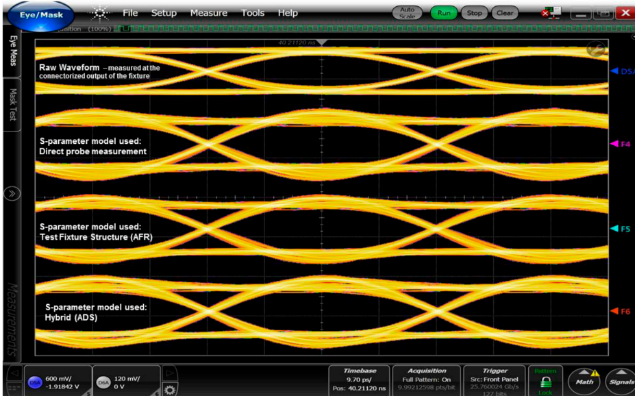
Figure 32: Direct DUT measurement at the output of the fixture (top) vs. de-embedded signals showing what the 25.78 Gb/s signal would look like at the balls of the device (three lower waveforms).
