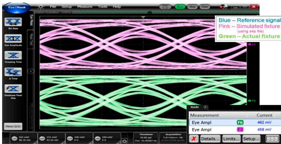
Figure 21: Eye diagram measurements of simulated fixture (F3 pink) and actual fixture (F6 green) showing good eye and amplitude correlation.
