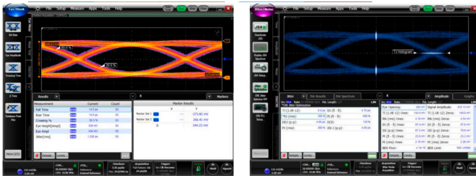
Figure 24: Eye diagram and jitter measurements of the reference signal establish a baseline for subsequent analysis (Rise/Fall times 14.5ps, Eye amplitude 434 mV, ISI 4.8 ps, TJ (@1E-12 8.8 ps).
