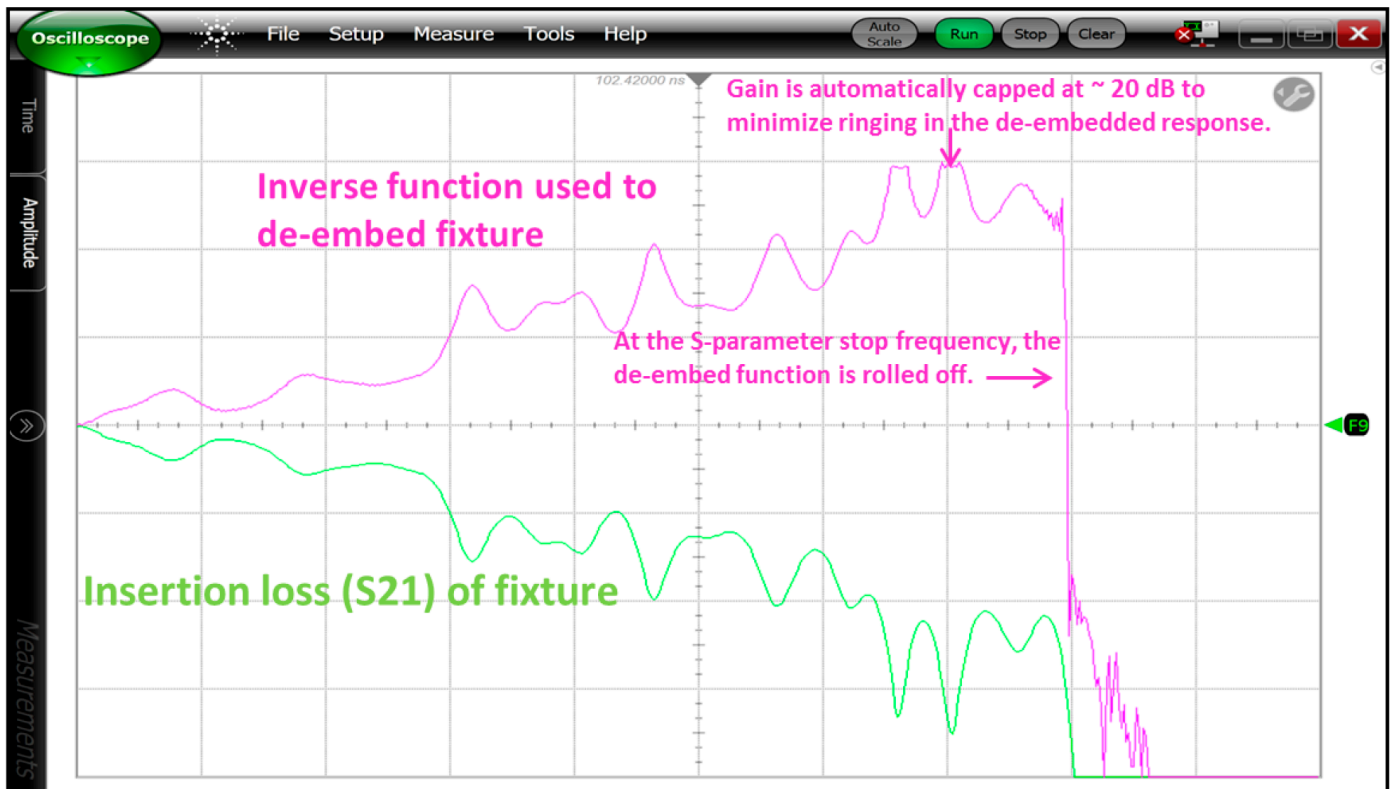
Figure 14: Frequency vs amplitude plot of a fixture's insertion loss profile (bottom trace S21) and the corresponding inverse function (top trace) used by de-embedding software to compensate for fixture effects.
