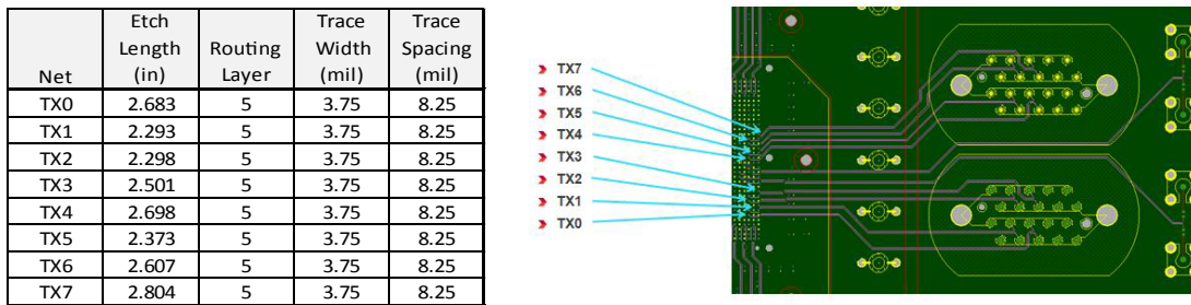
Figure 2: VC7222 28Gbps internal stripline routing design parameters and the resulting Detail 'A' PCB layout with the location shown in Figure 3.
