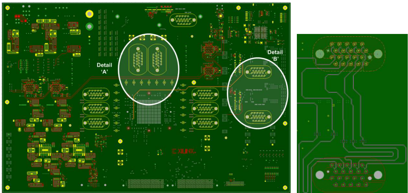
Figure 3: Top view of the VC7222 PCB with the 28Gbps Channels in Detail 'A' and the test fixture calibration structures in Detail 'B', which are expanded on the right to show the inner layer routing.
