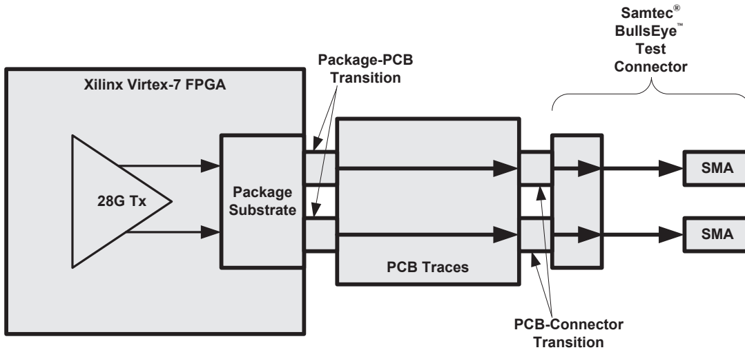
Figure 1: 28G Signal path
