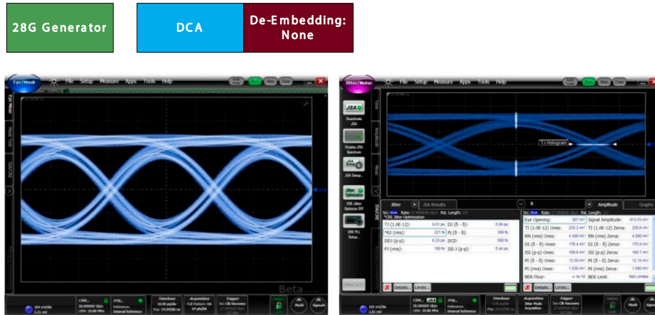
Figure 19: Eye diagram and jitter measurements of the reference signal.
