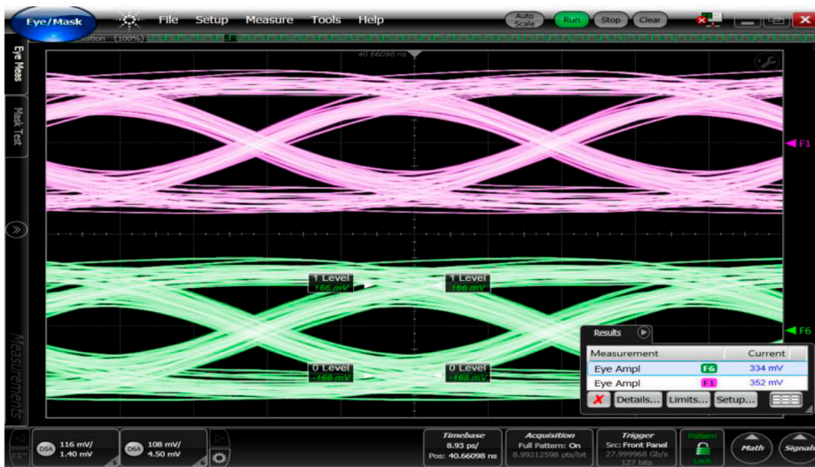
Figure 26: Good correlation between simulated and measured signals.
