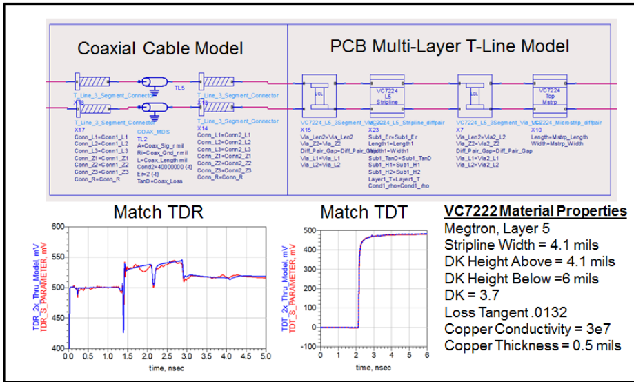
Figure 9: Creating a measurement based model by matching transmission line impedances with that of 2x fixture test structures enables the extraction of material properties and the ability to quickly simulate all the fixture paths for a given routing layer.
