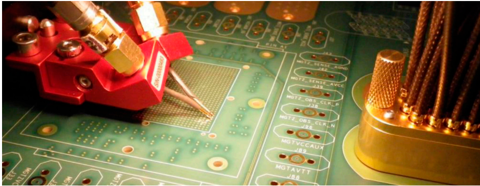
Figure 6: High performance Ground-Signal-Ground probes for direct measurement of the channel fixture path for de-embedding from the active measurement of the DUT to accurately predict the performance at the package. (Probes courtesy of Gigatest Labs)
