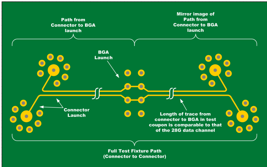
Figure 4: Calibration test fixture design
