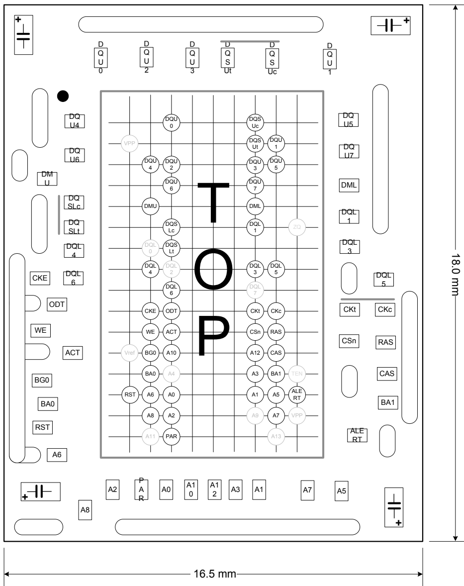
Figure 4. N2115A dimension drawing of interposer.
