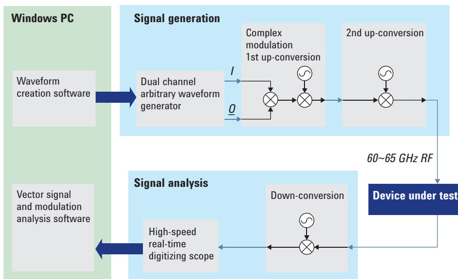
Block diagram of the complete test setup
