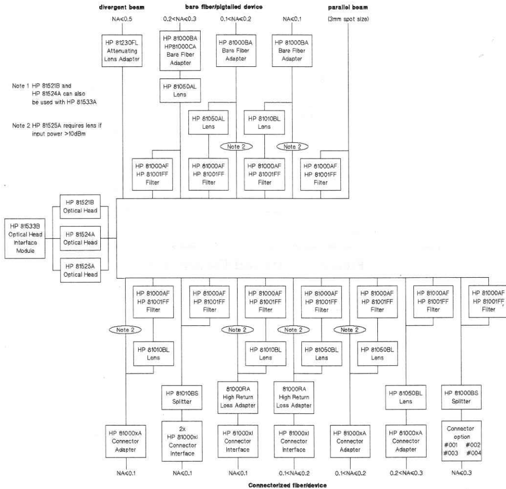
Figure C-2. Optical Connections
