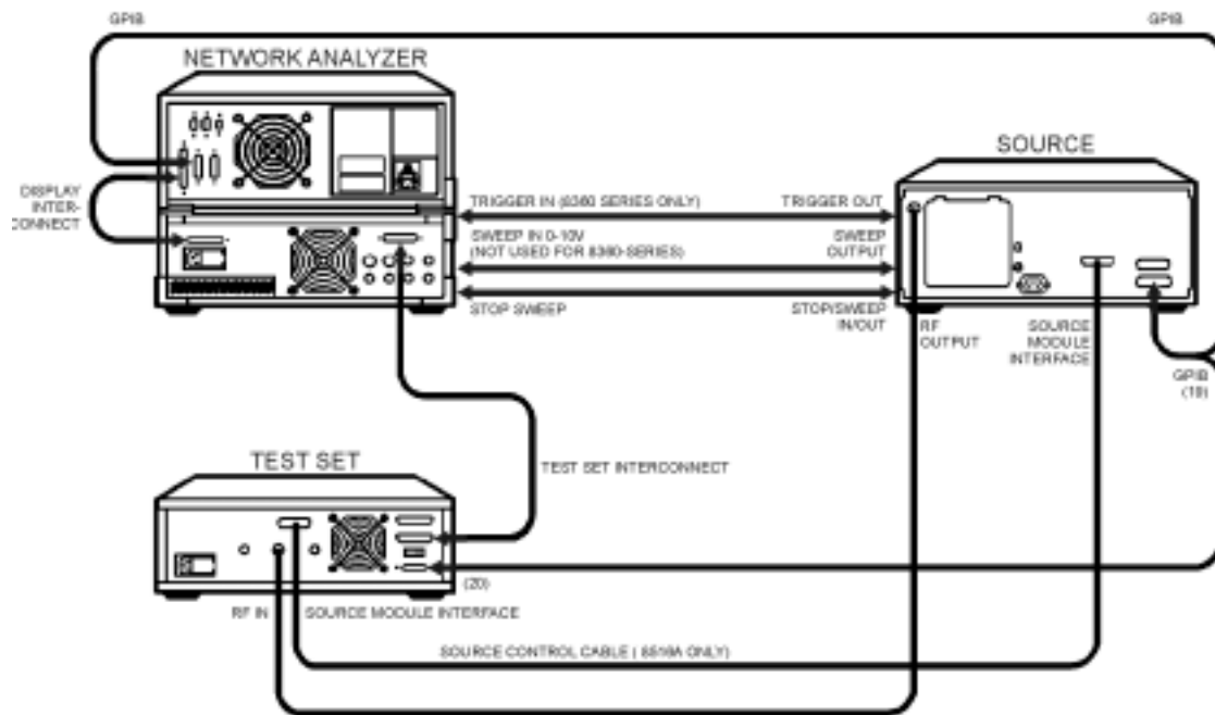
Figure 6 Typical 8510 System Connections
