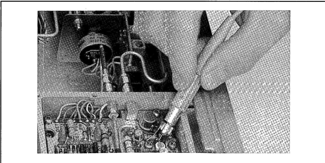
Figure 8B-3. Troubleshooting Probe for use within Doubler Amplifier (Option 002)
