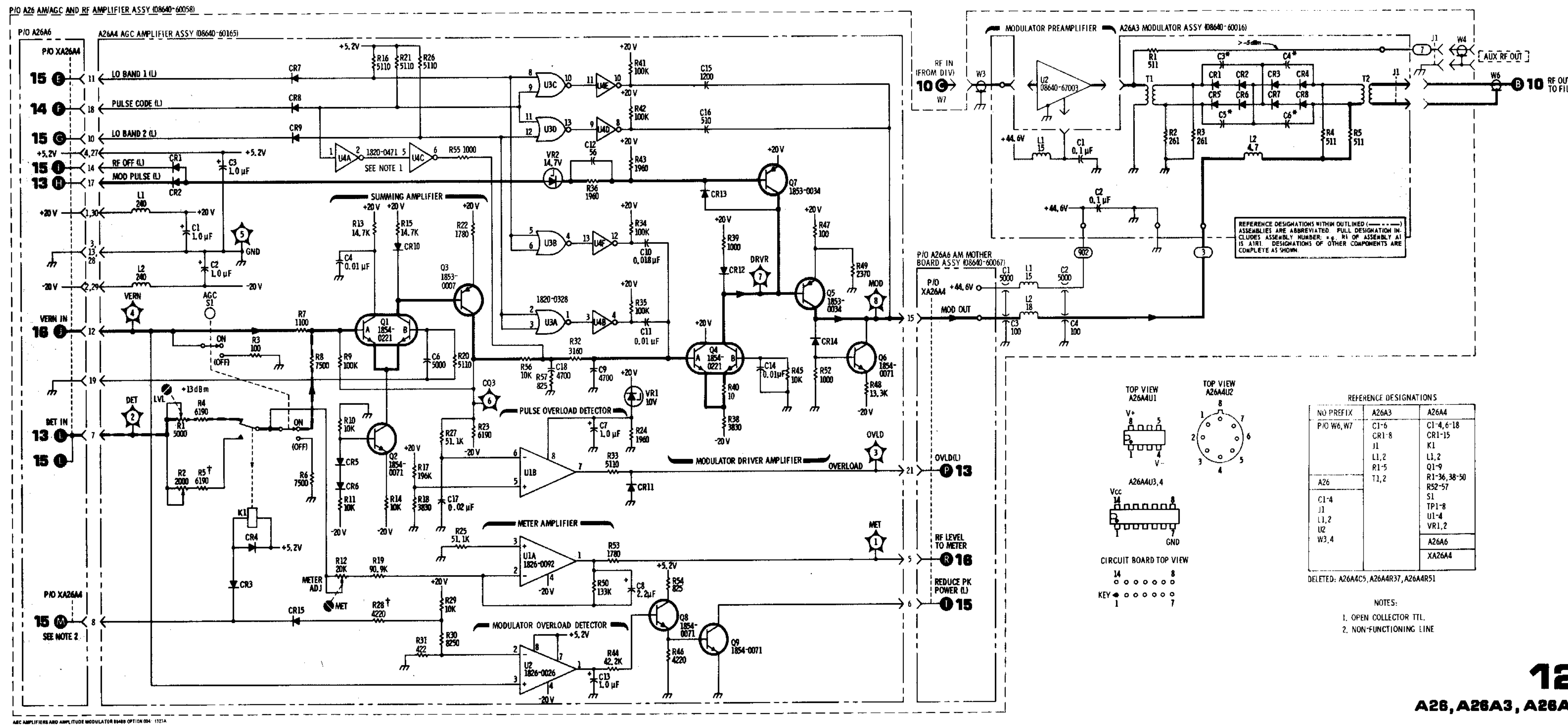
Figure 8-46. AGC Amplifiers and Amplitude Modulator Schematic Diagram
