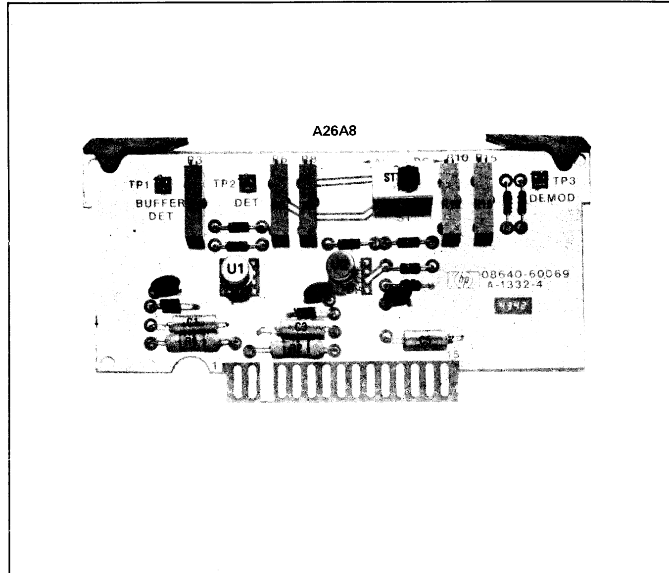
Figure 8-52. A26A8 Demodulation Amplifier Assembly Component Locations
