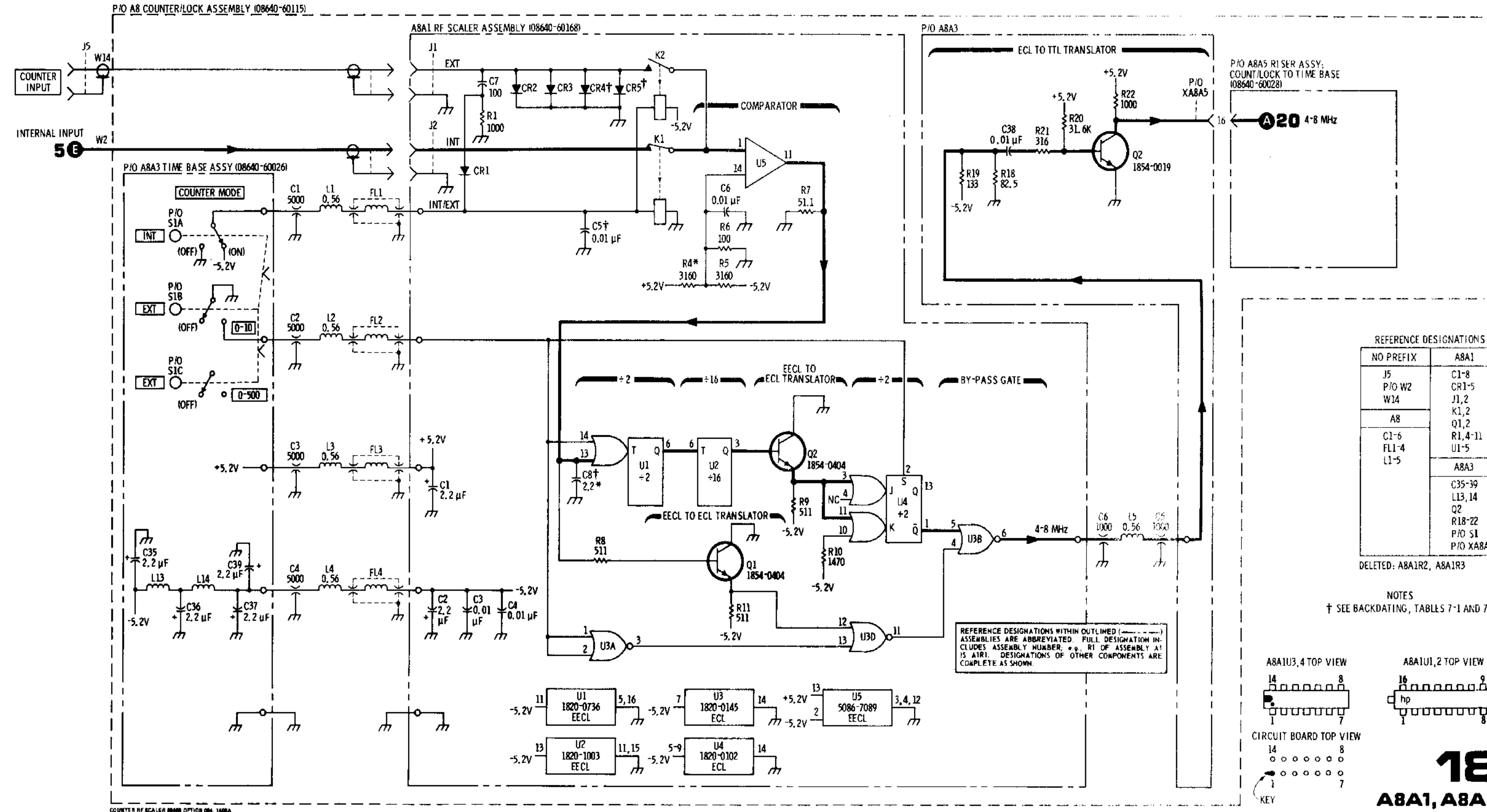
Figure 8-62. Counter RF Scaler Schematic Diagram
