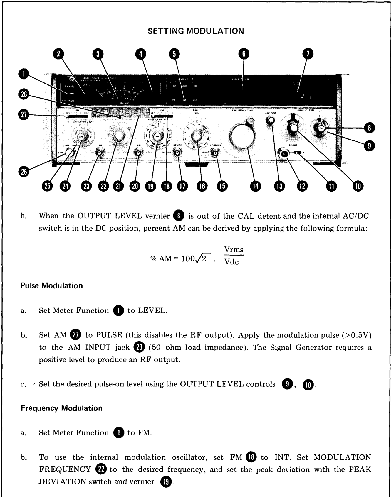
Figure 3-7. Setting the Modulation Controls (3 of 5)
