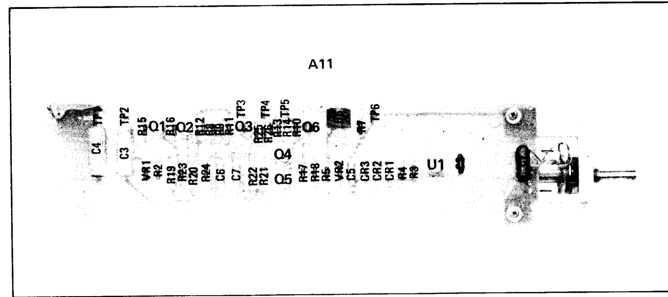
Figure 8-34. A11 Fixed-Frequency Modulation Oscillator Component Locations
