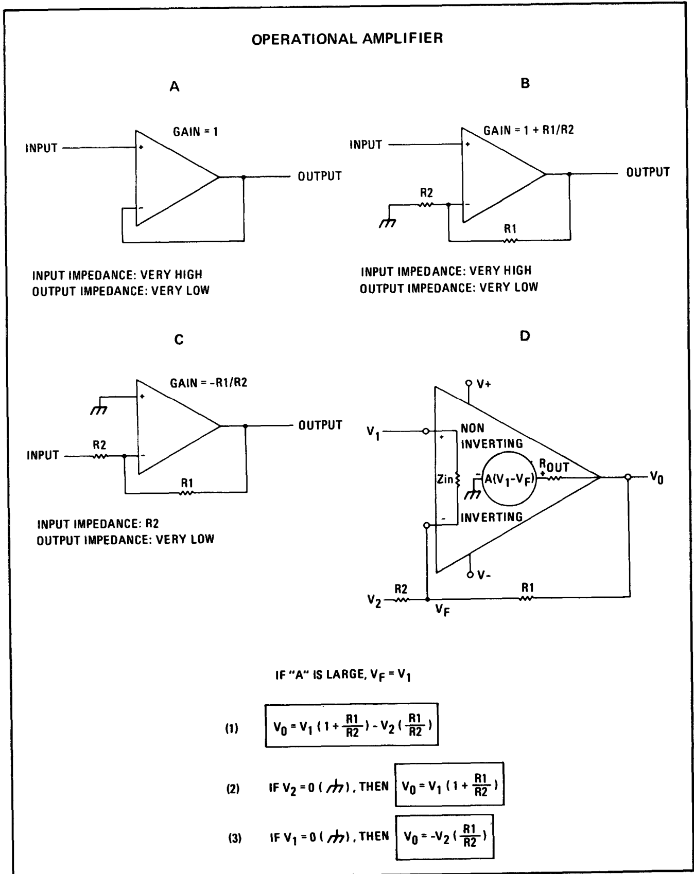
Figure 8-15. Operational Amplifier
