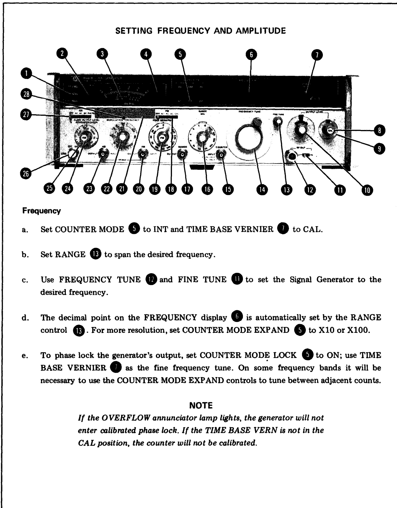
Figure 3-6. Setting the Frequency and Amplitude Controls (1 of 3)
