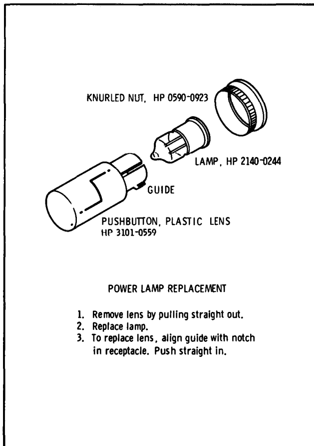
Figure 3-1. Lamp Replacement
