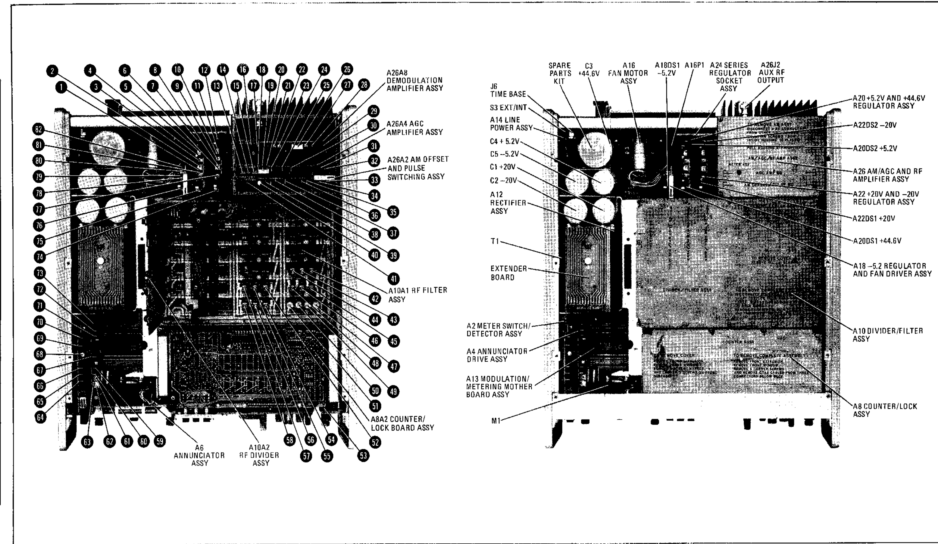
Figure 8-90. Top Internal Views (Option 001 Shown)
