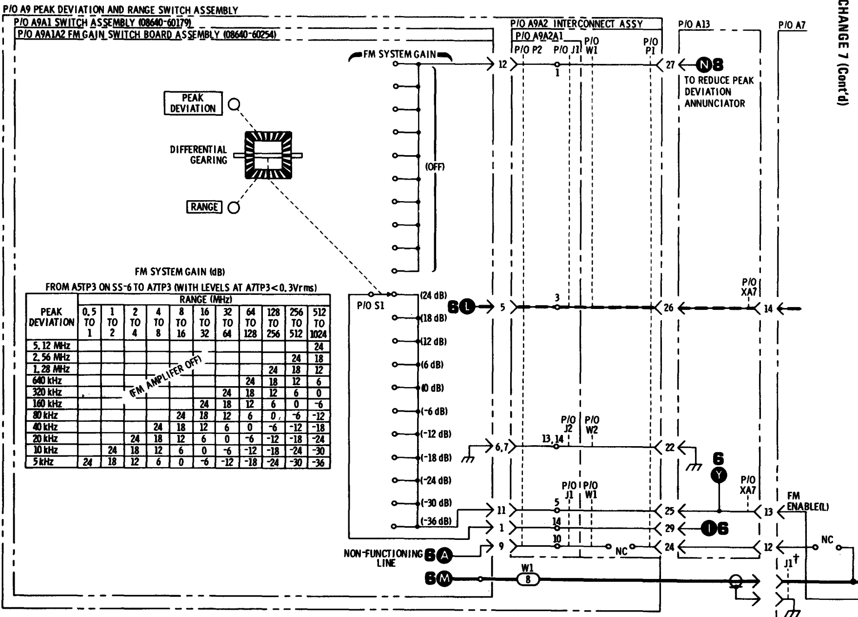
P/O Figure 8-29. FM Shaping Circuits and Phase Lock Loop Filter Schematic Diagram (P/O Change 7)
