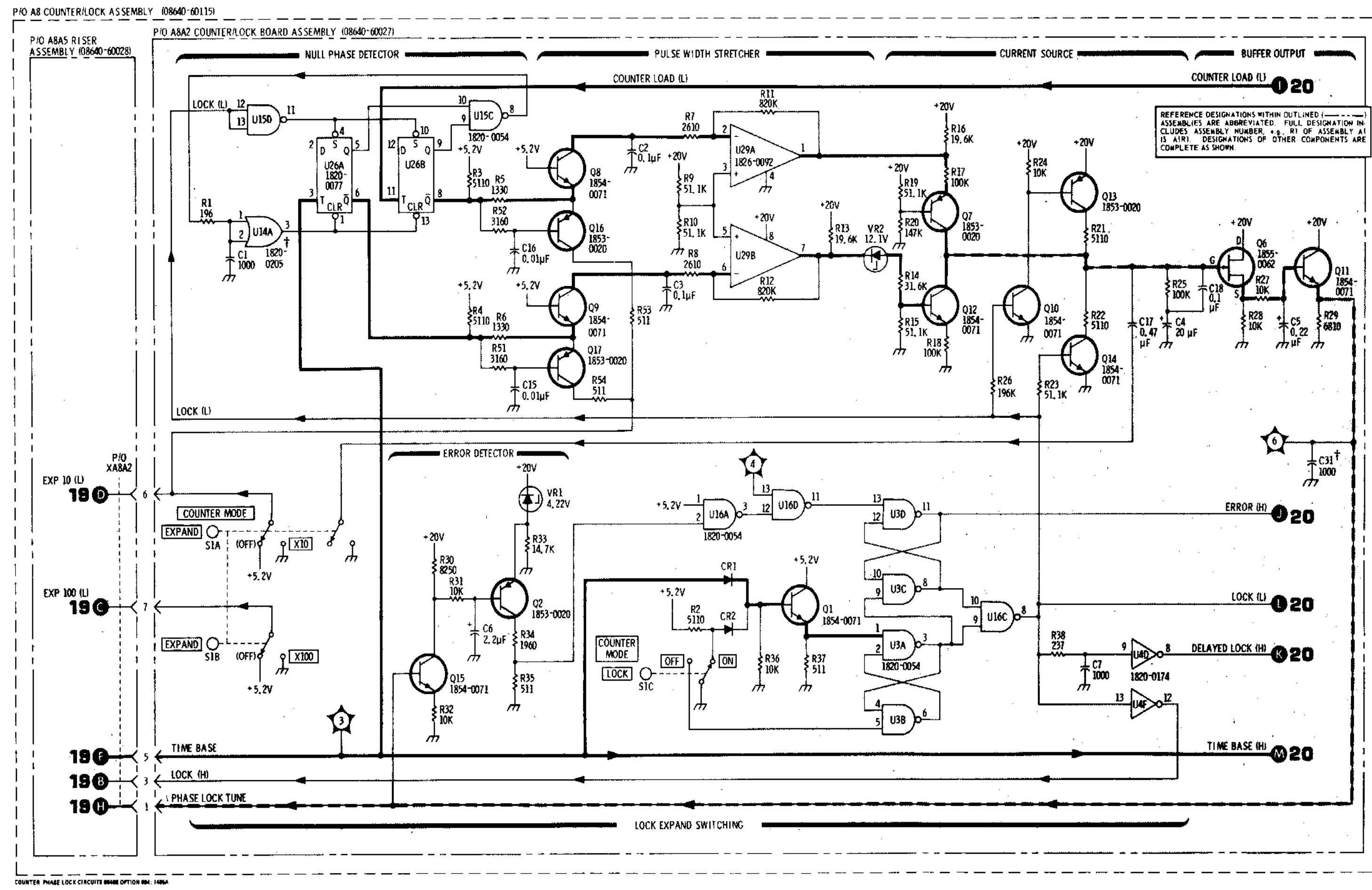
Figure 8-69. Counter Phase Lock Circuits Schematic Diagram
