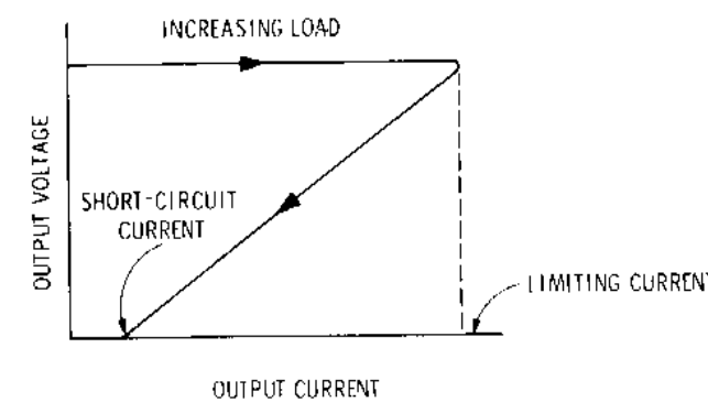
Figure 8-70. Current Foldback
