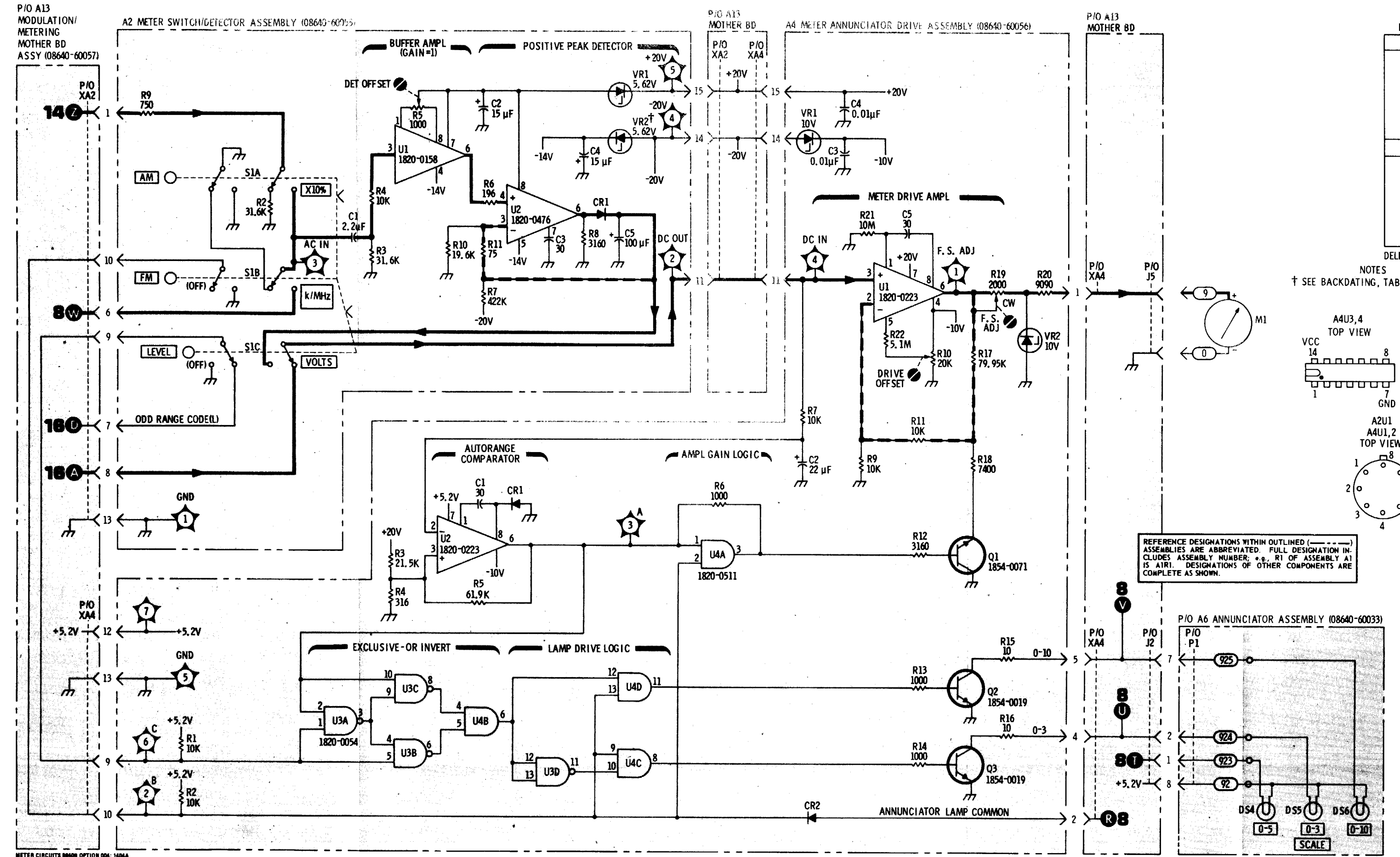
Figure 8-59. Meter Circuits Schematic Diagram
