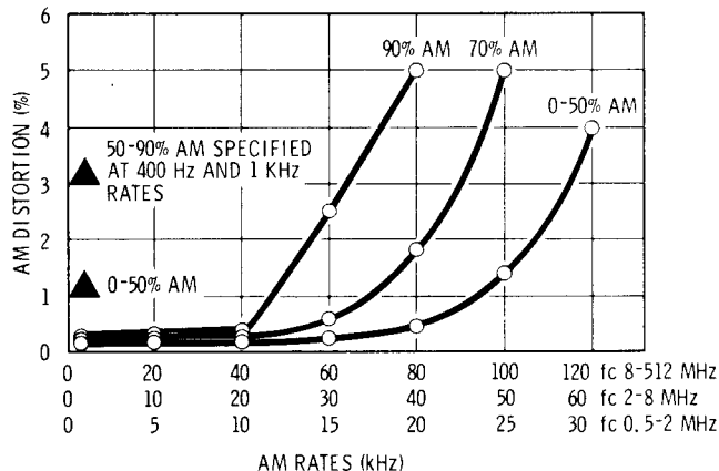
Figure 1-4. AM distortion us AM rate measured at 200 MHz and +10 dBm, but applies to all bands. (Supplemental information only.)
