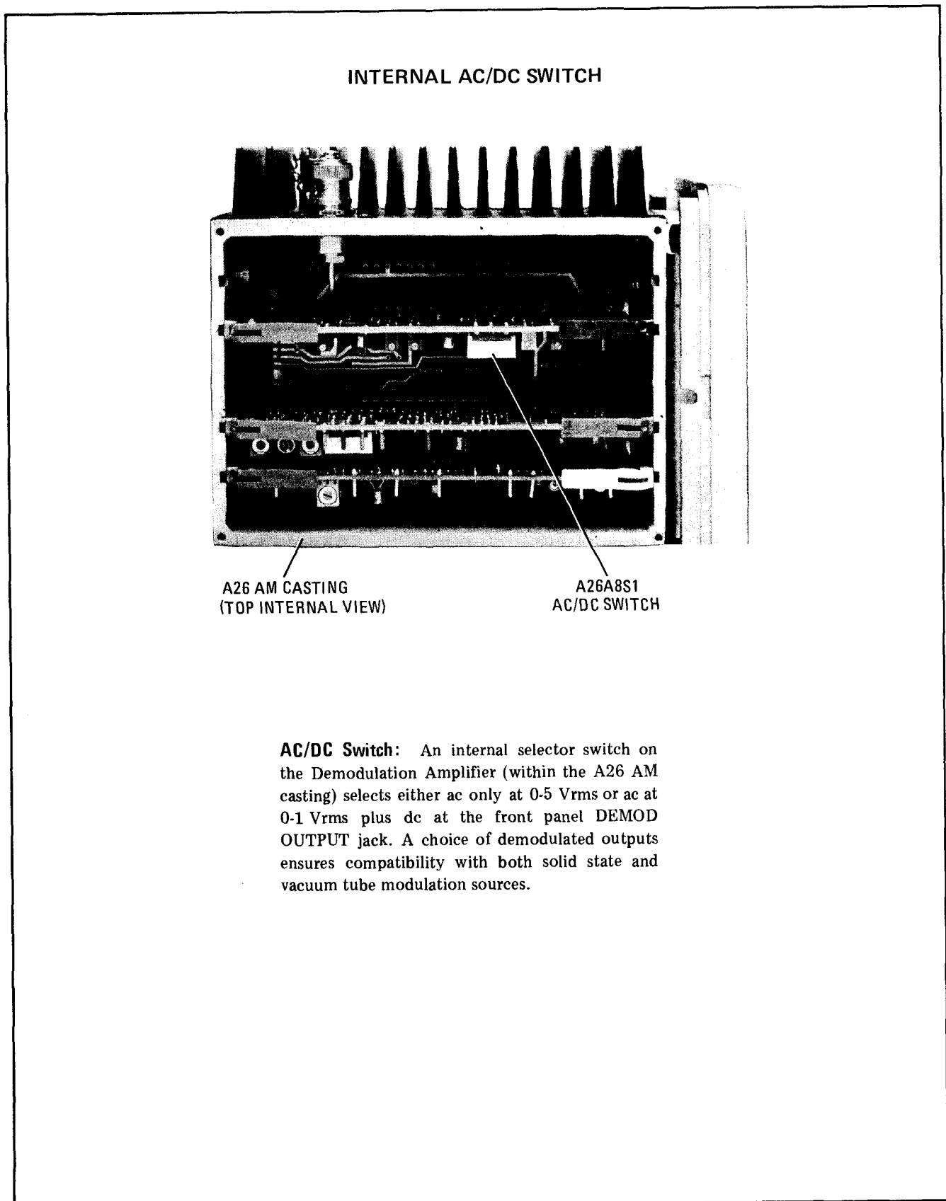
Figure 3-3. Internal AC/DC Switch
