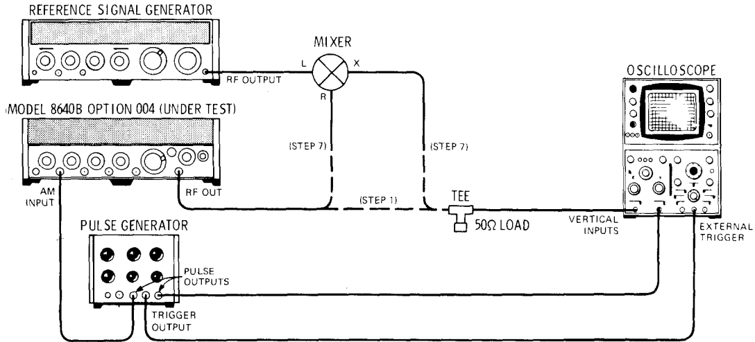
Figure 4-26, Pulse Modulation Test Setup
