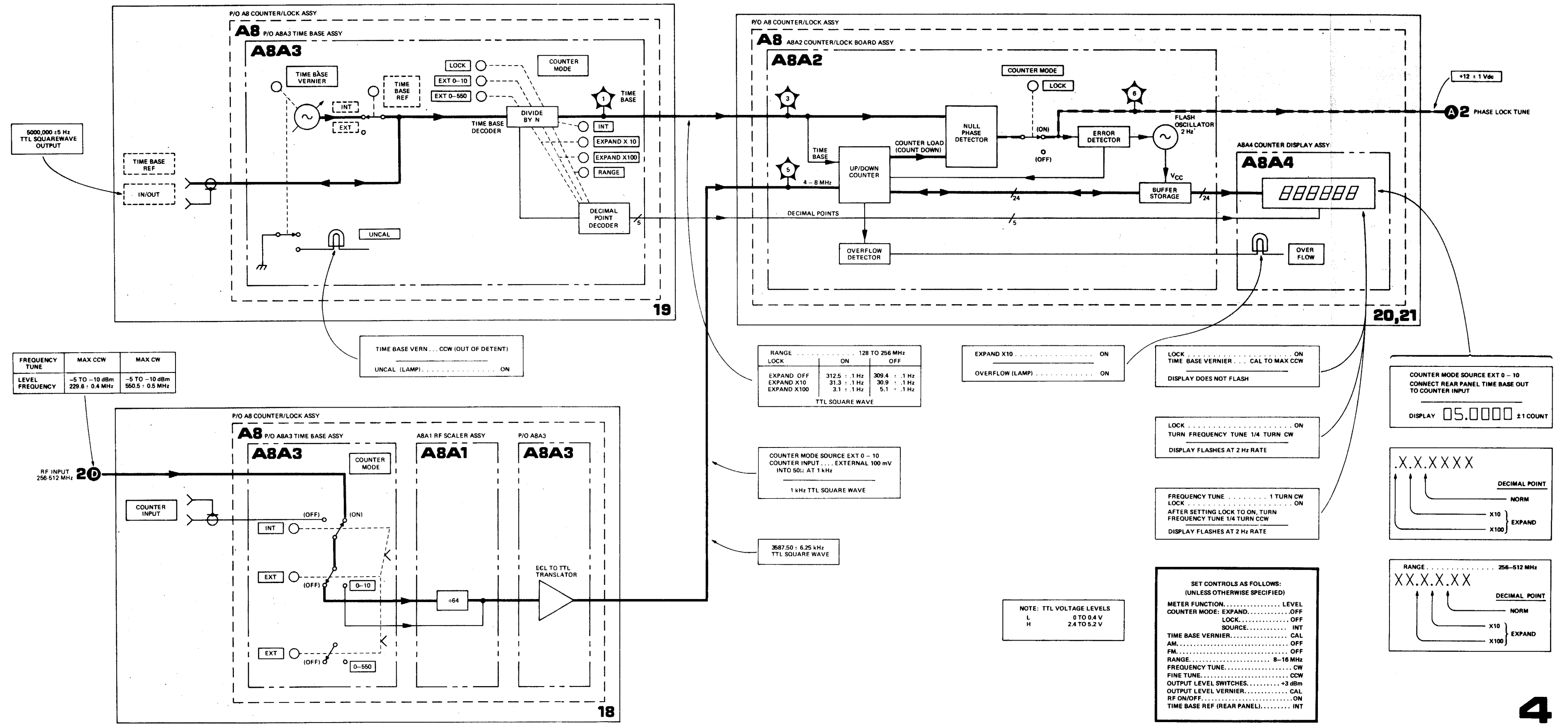
Figure 8-21. Counter/Lock Circuits Block Diagram
