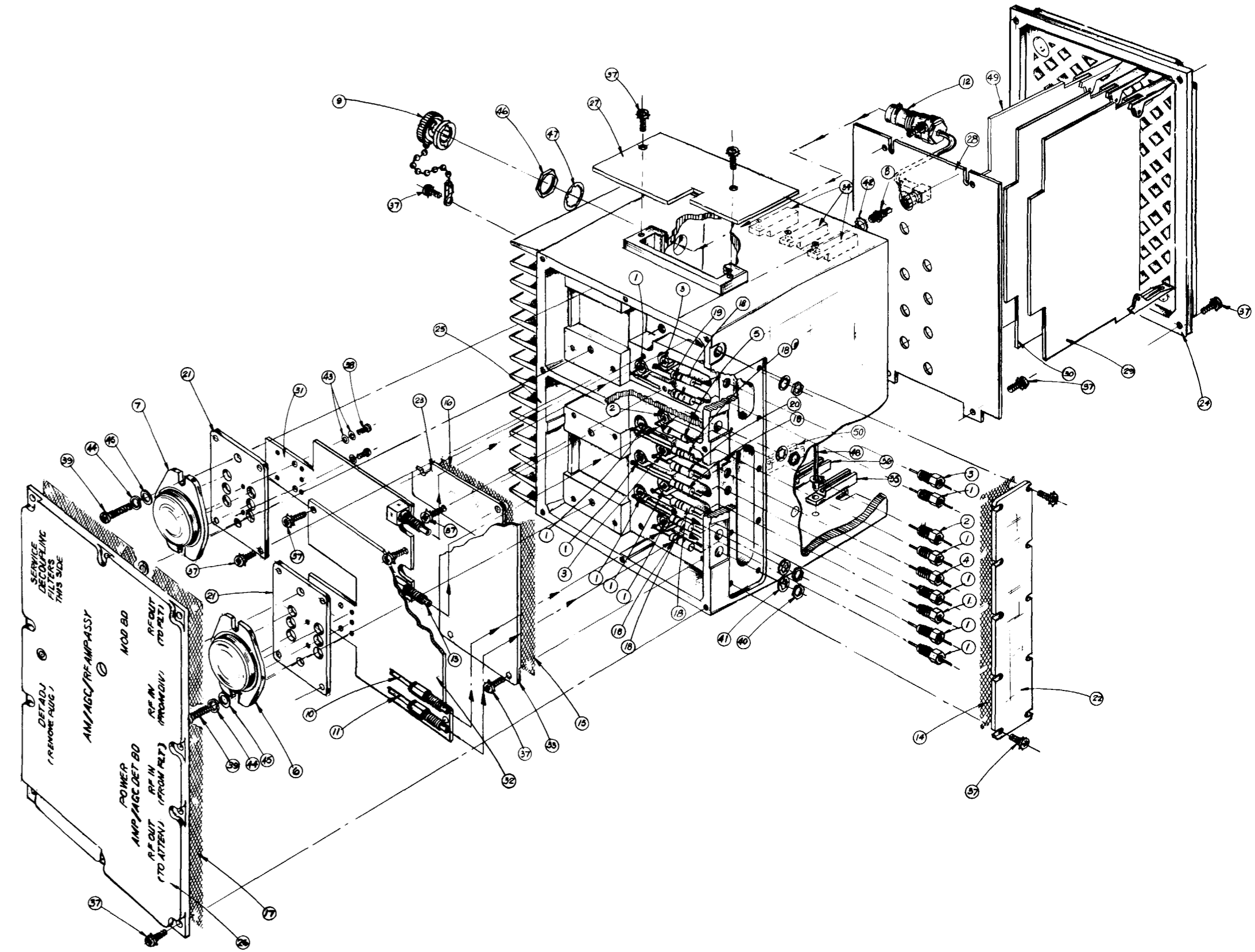
Figure 8-89. A26 AM/AGC and RF Amplifier Illustrated Parts Breakdown
