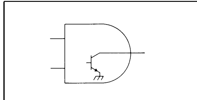
Figure 8-3. Open Collector Output Stage (AND Gate)
