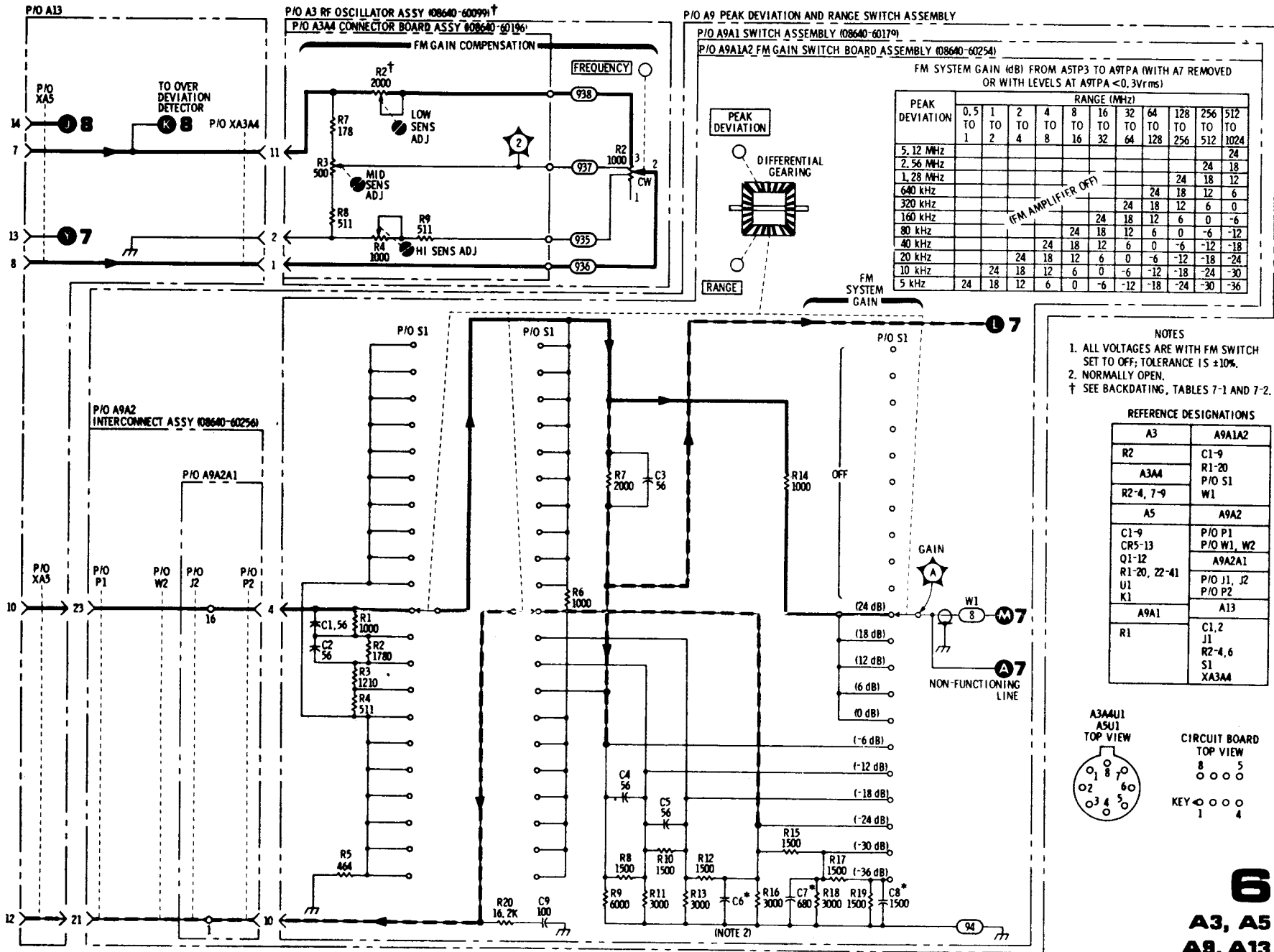
P/O Figure 8-27. FM Amplifiers Schematic Diagram (2 of 2, P/O Change 7)
