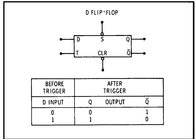
Figure 8-6. D Flip-Flop
