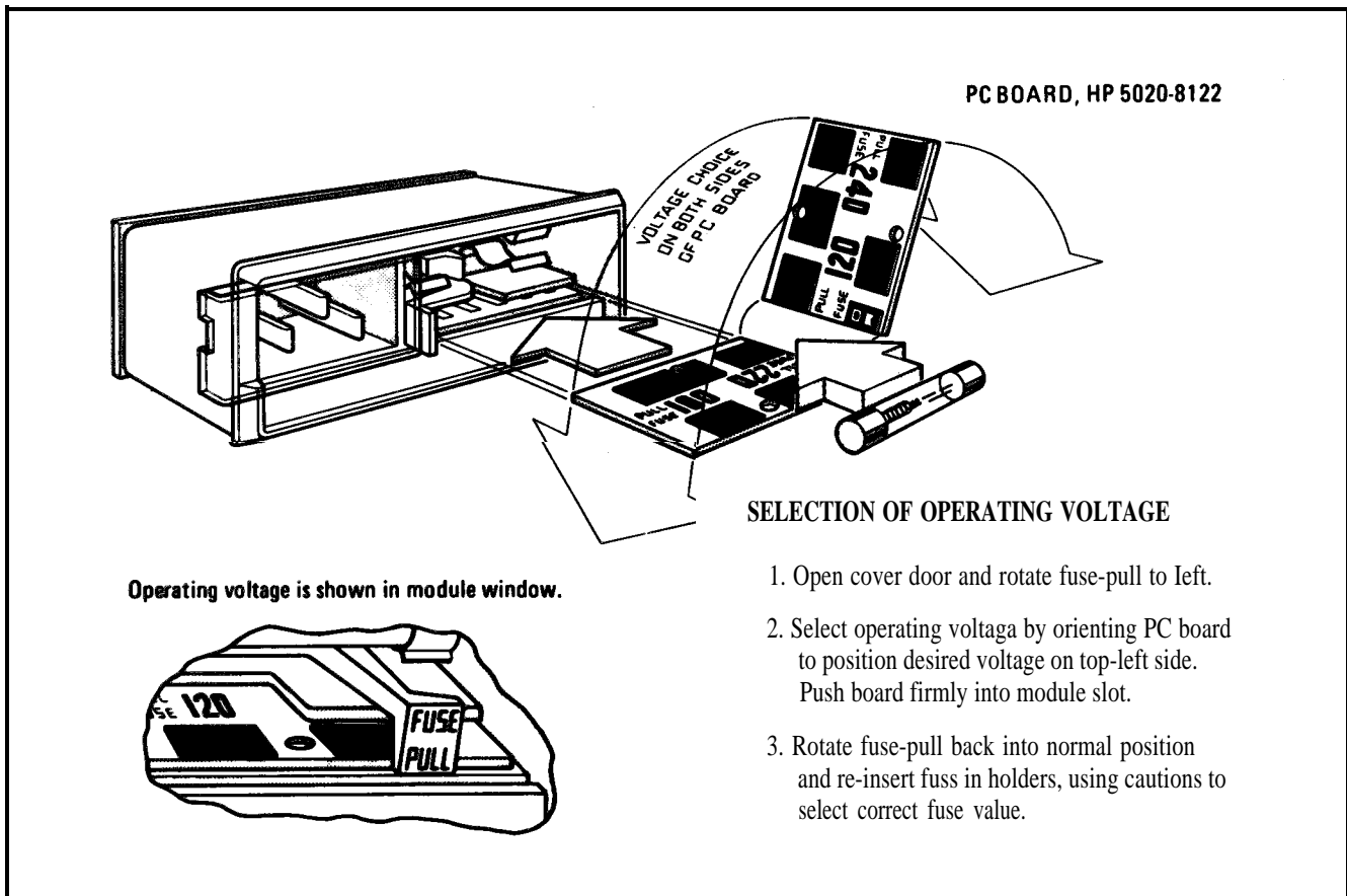
Figure 2-1. Line Selector
