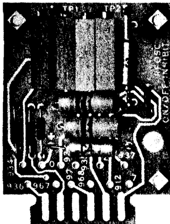
Figure 8-22. P/O A3A4 Connector Board Assembly Component Locations (P/O Change 2)
