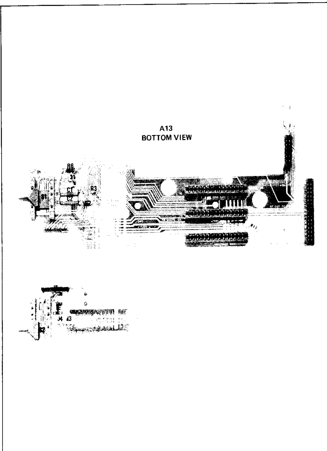
Figure 8-79. A13 Modulation/Metering Mother Board Assembly Component Locations (2 of 2)
