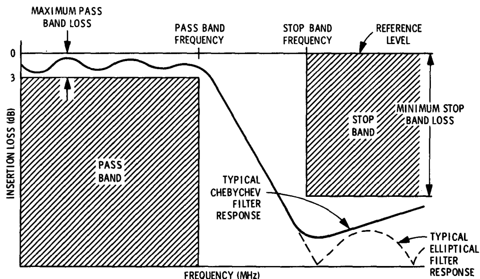
Figure 5-8. Filter Terminology
