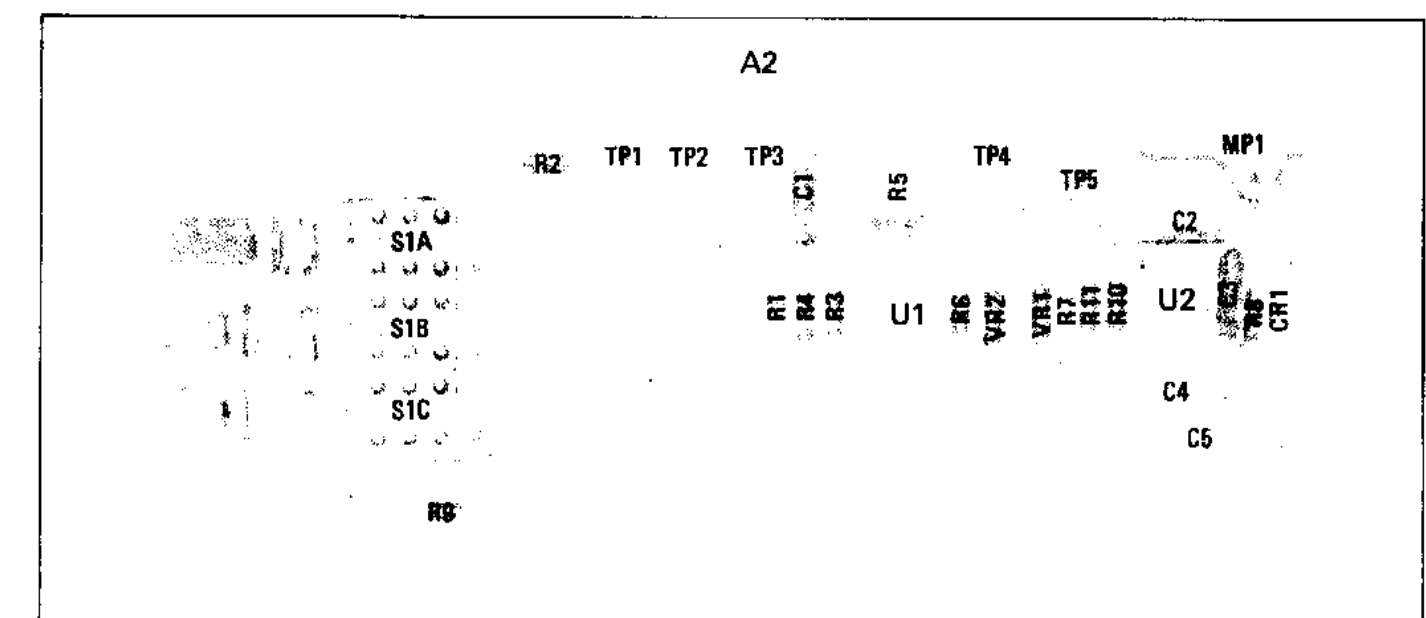
Figure 8-56. A2 Meter Switch/Detector Assembly Component Locations
