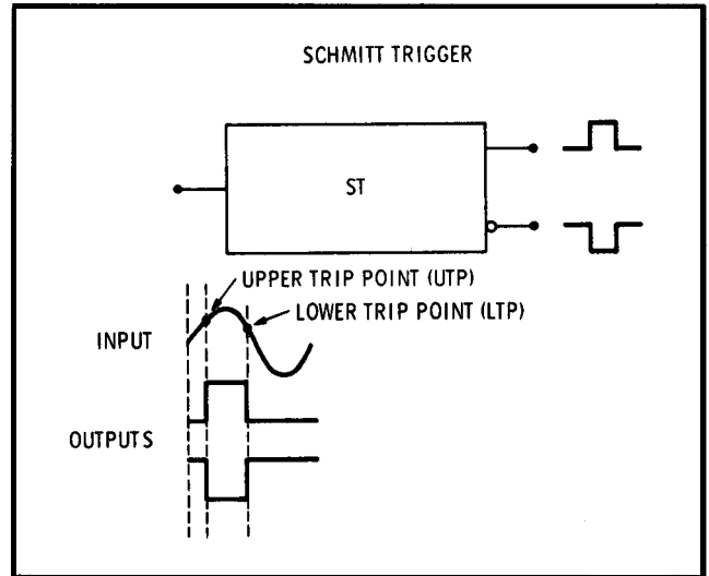
Figure 8-7. Schmitt Trigger
