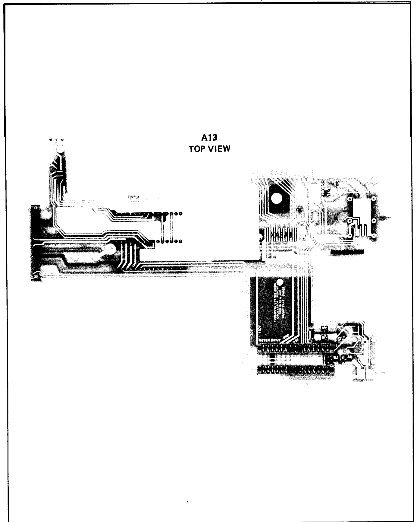
Figure 8-79. A13 Modulation/Metering Mother Board Assembly component Locations (1 of 2)
