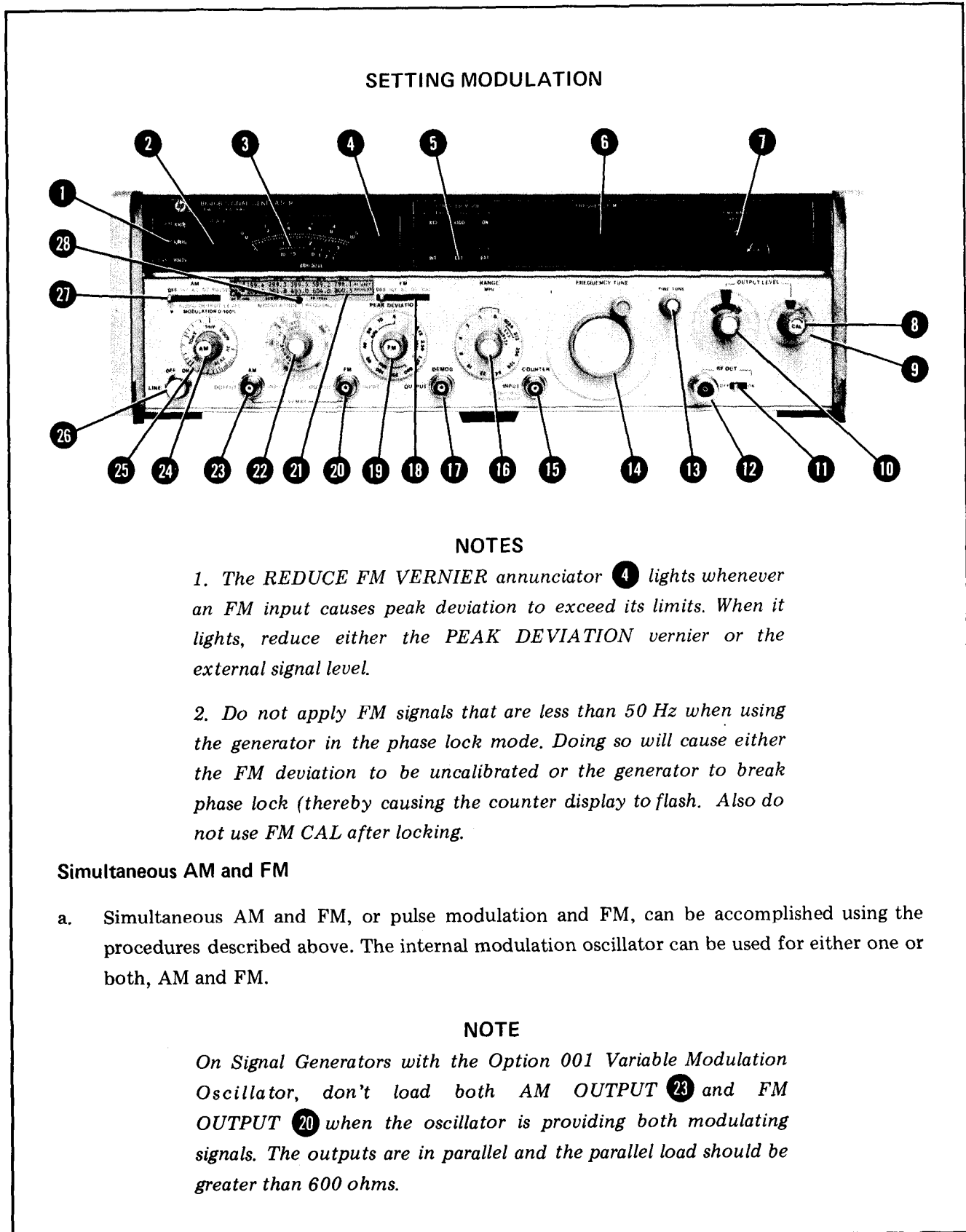
Figure 3-7. Setting the Modulation Controls (5 of 5)
