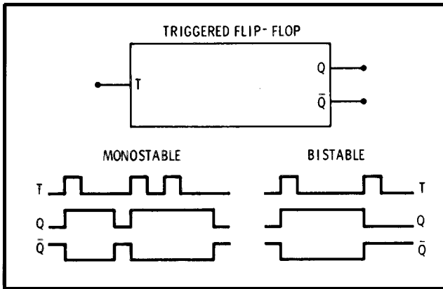
Figure 8-5. Triggered Flip-Flop
