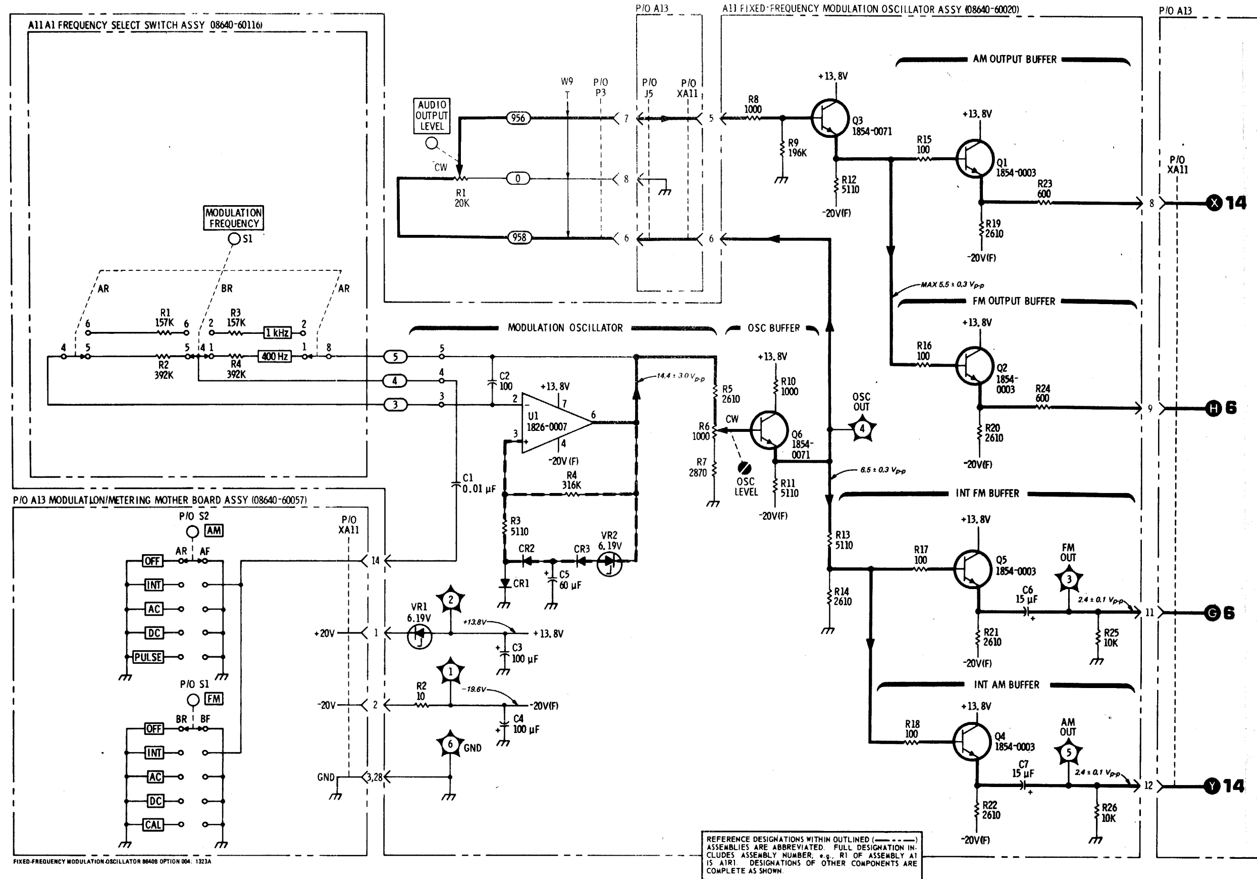
Figure 8-35. Fixed-Frequency Modulation Oscillator Schematic Diagram
