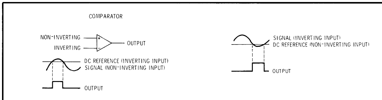
Figure 8-16. Comparator
