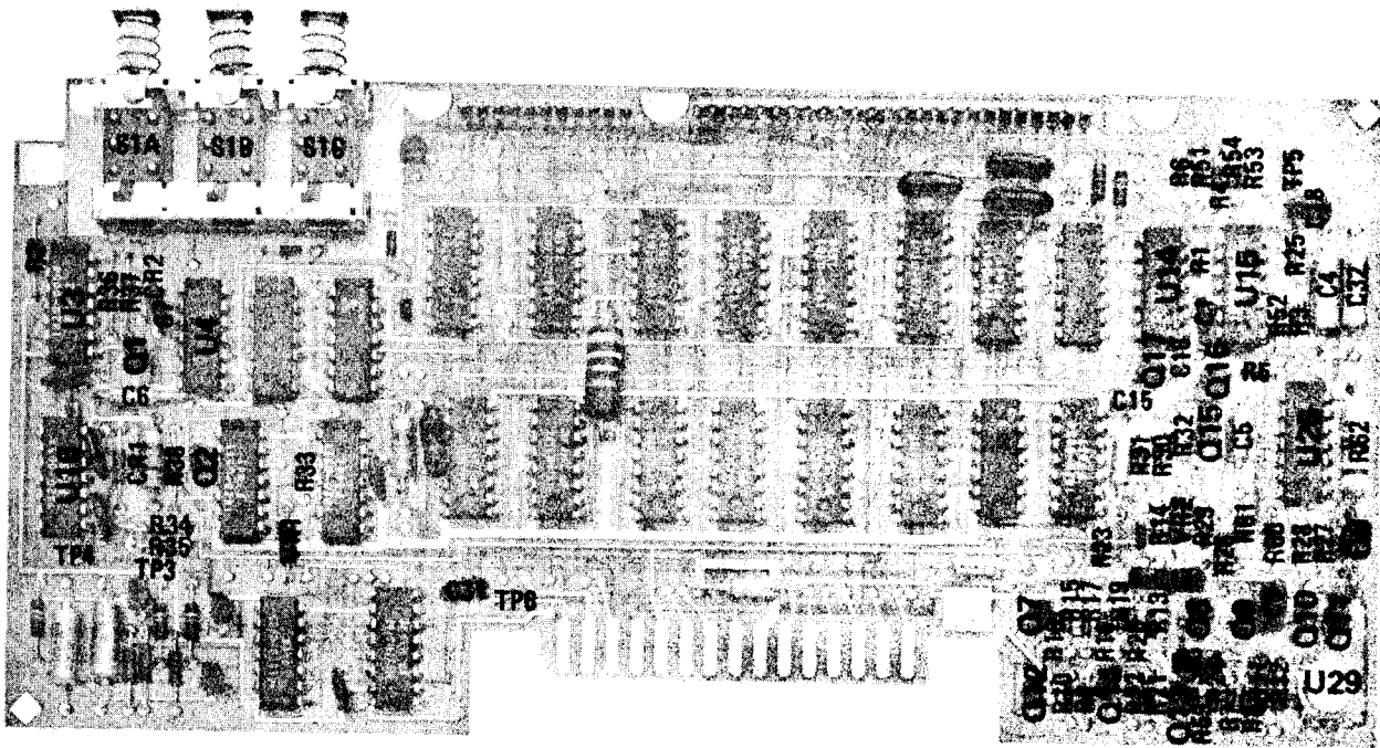
Figure 8-68. P/O A8A2 Counter/Lock Board Assembly, Component Locations {P/O Change 16}
