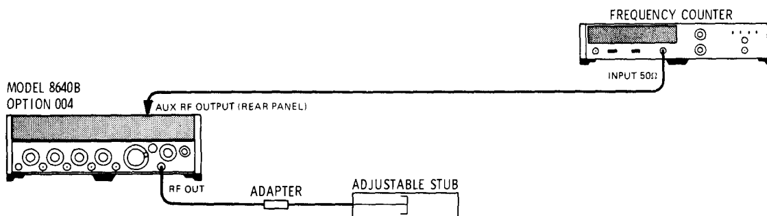
Figure 4-4. Frequency Stability us Load, Level, and Mode Test Setup
