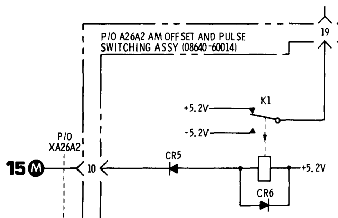
Figure 7-1. A26A 2 AM Offset and Pulse Switching Assembly Backdating (Change C)
