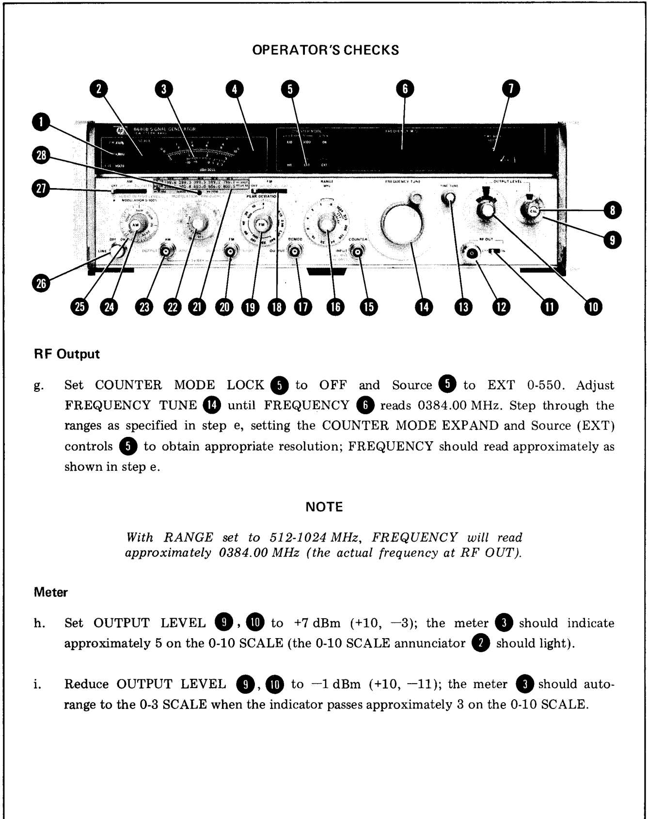
Figure 3-5. Operator's Checks (3 of 5)
