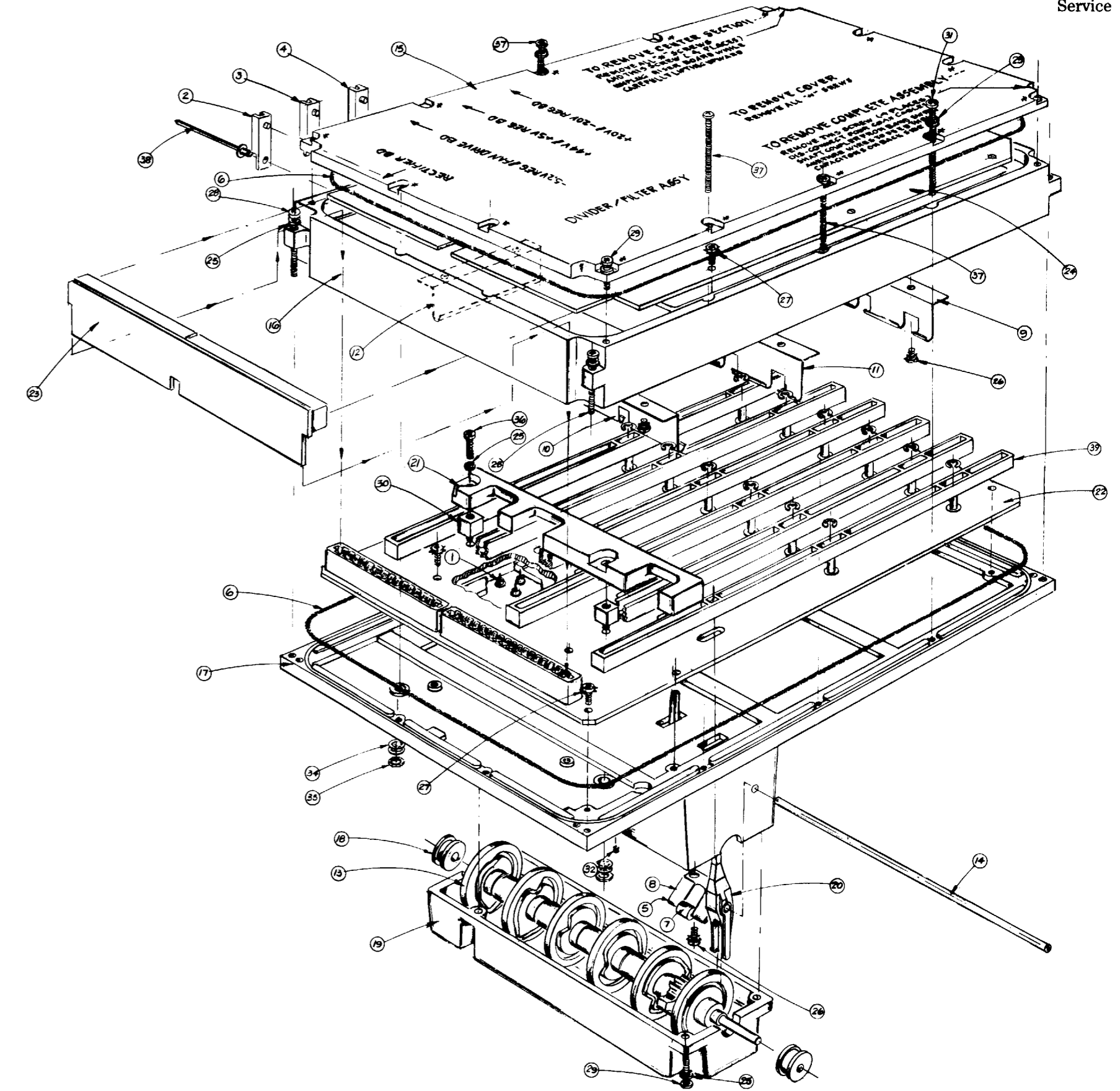
Figure 8-88. A10 Divider/Filter Assembly Illustrated Parts Breakdown
