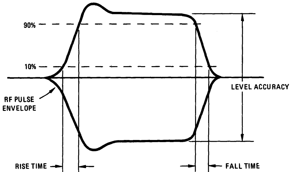
Figure 4-27. Pulse Measurements
