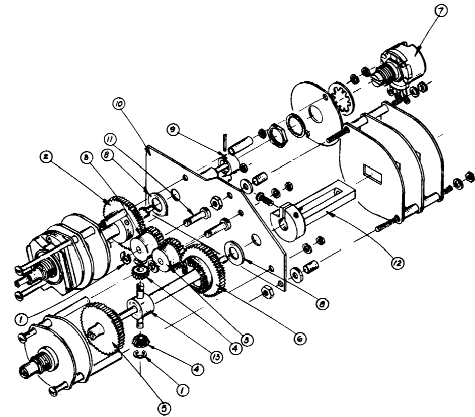
Figure 8-86. A9 Peak Deviation and Range Switch Assembly Illustrated Parts Breakdown
