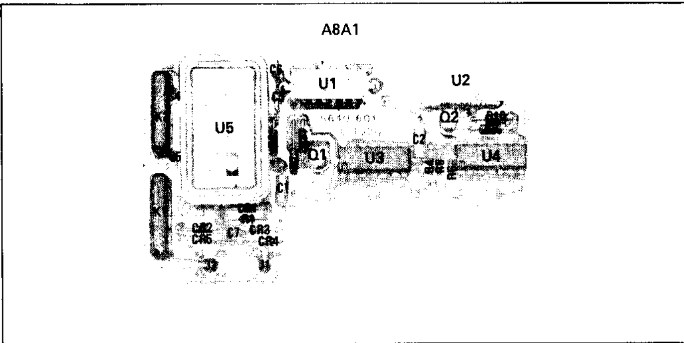
Figure 8-60. A8A1 RF Scaler Assembly Component Locations
