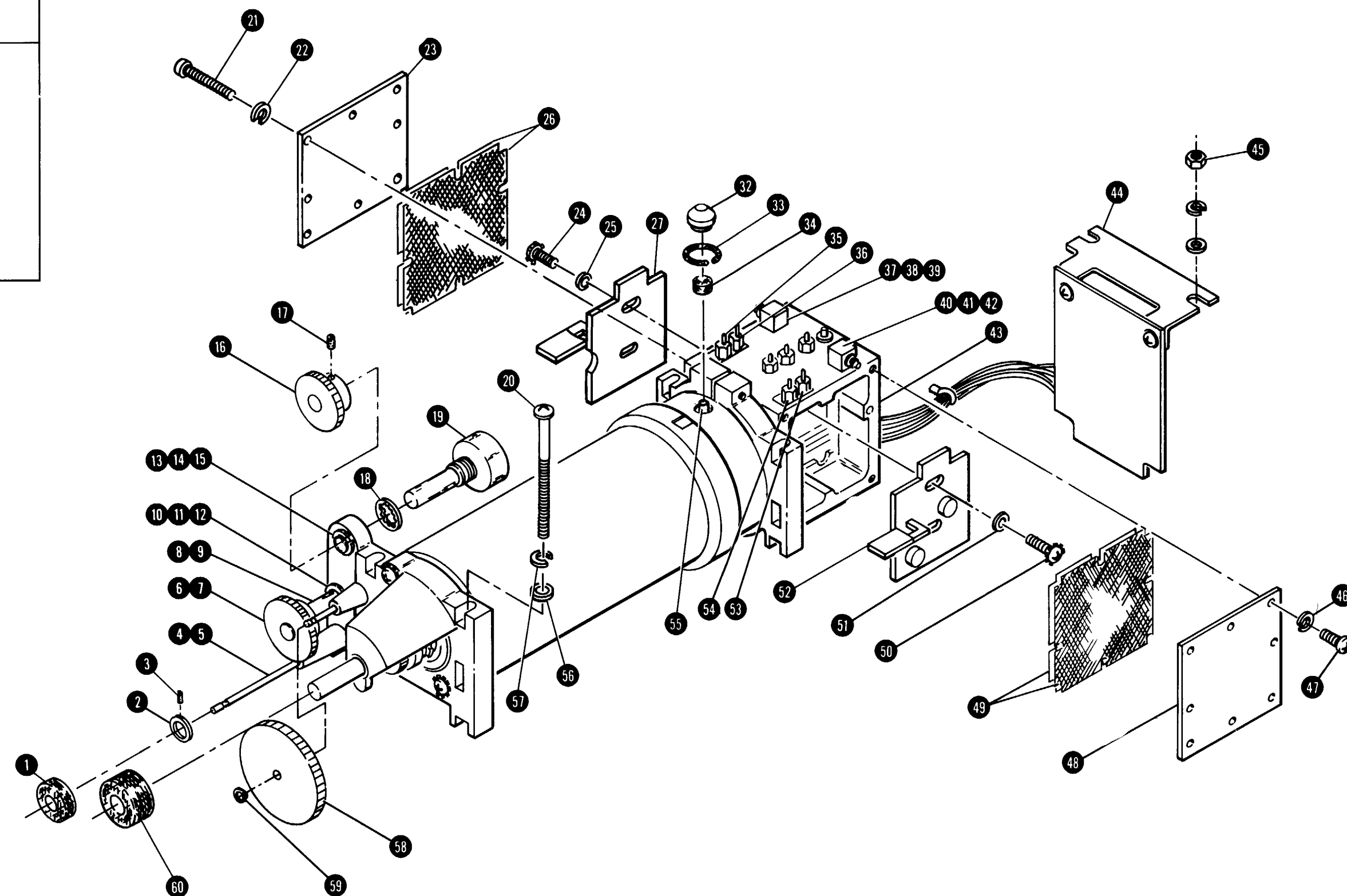
Figure 8-84. A3 RF Oscillator Illustrated Parts Breakdown
