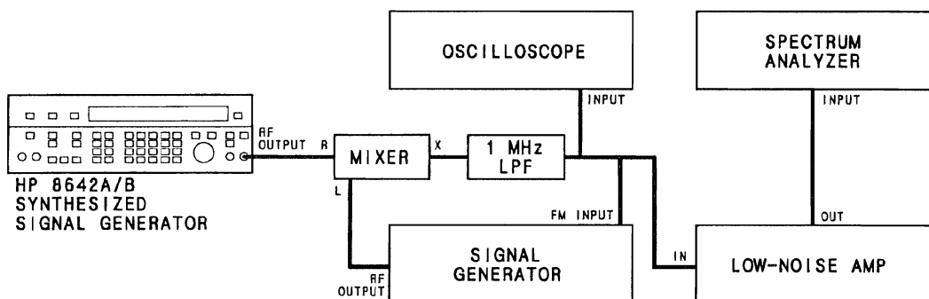
Figure 4-12. SSB Phase Noise Test Setup (Optional)
