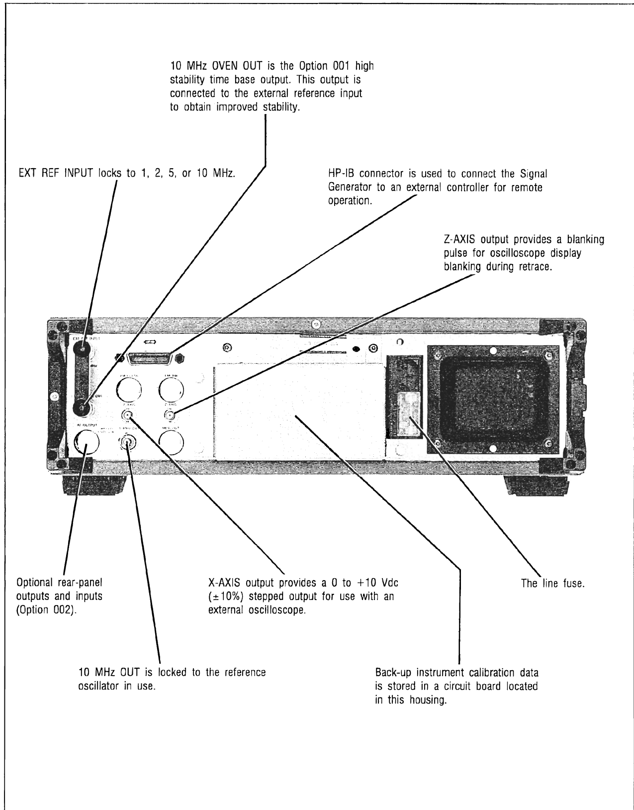
Figure 3-2. Rear-Panel Features
