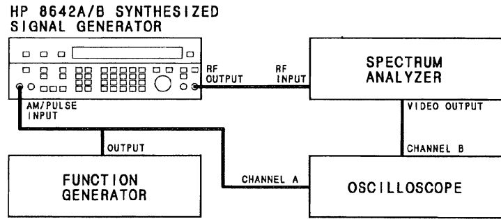
Figure 4-13. Pulse Test Setup
