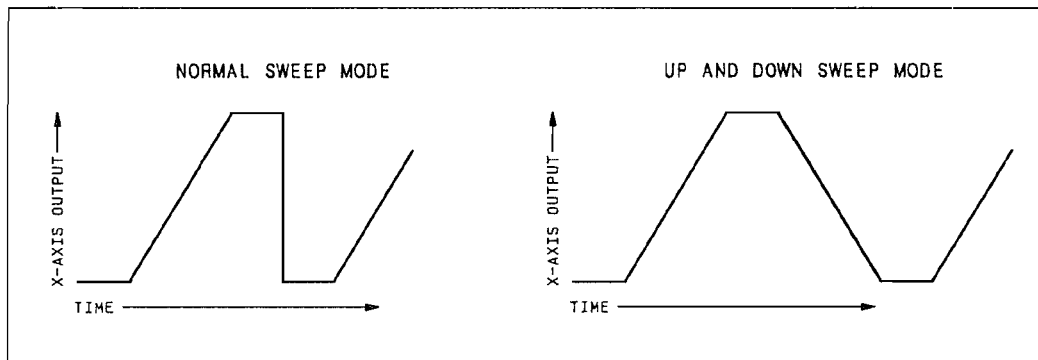
Figure 3-10. Sweep Waveforms
