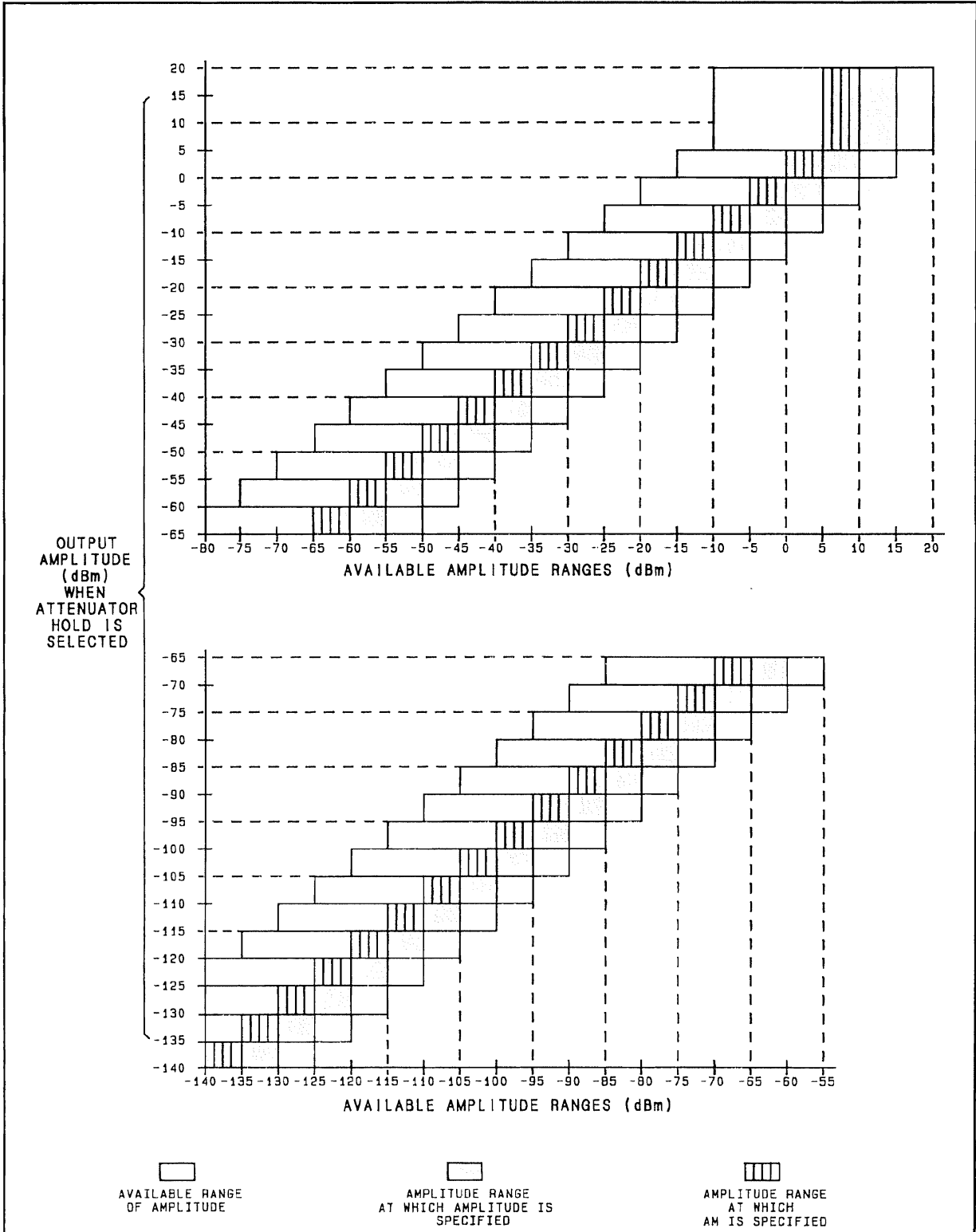
Figure 3-9. Attenuator Range Hold; Amplitude and AM Ranges
