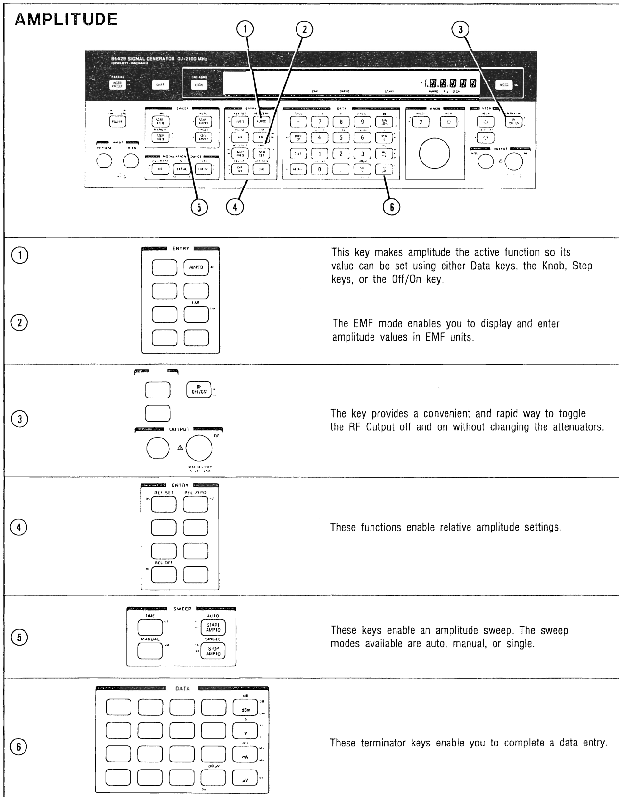
Figure 3-8. Amplitude-Related Functions
