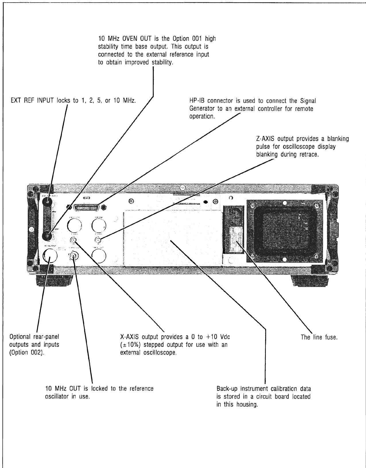
Figure 3-2. Rear-Panel Features
