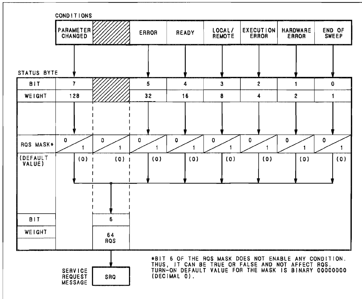
Figure 3-4. The Status Byte and RQS Mask
