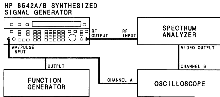
Figure 4-13. Pulse Test Setup
