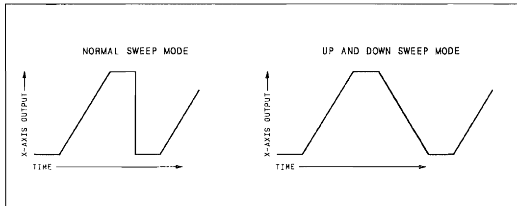
Figure 3-7. Sweep Waveforms
