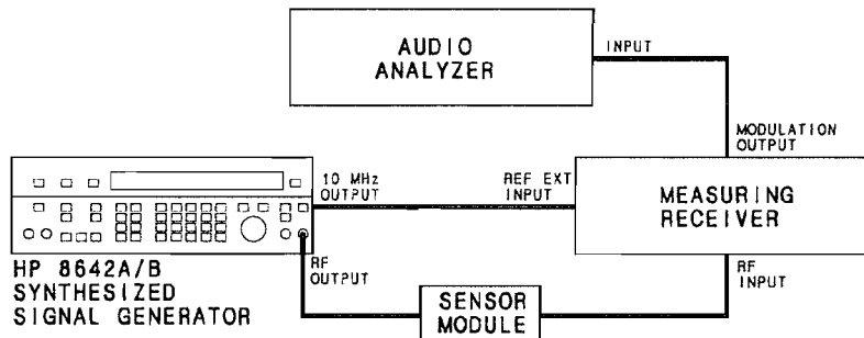
Figure 4-6. FM Distortion Test Setup
