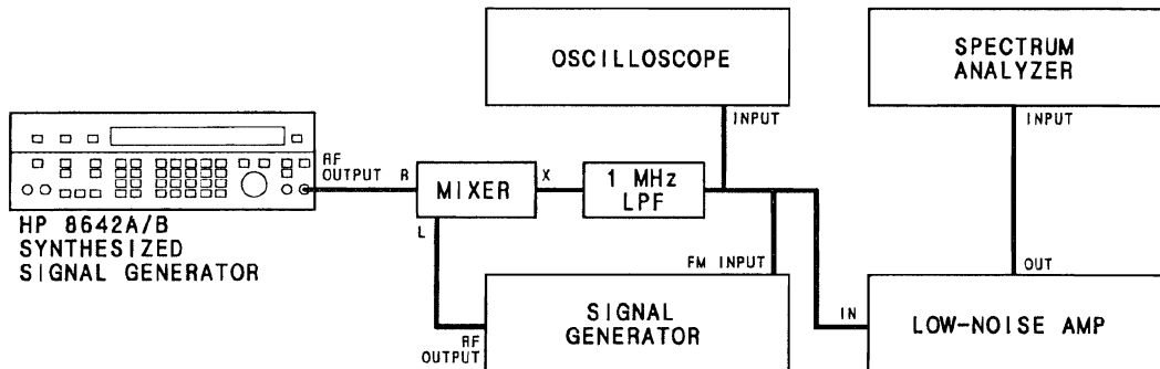
Figure 4-12. SSB Phase Noise Test Setup (Optional)
