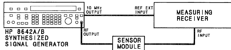
Figure 4-2. Harmonics Test Setup
