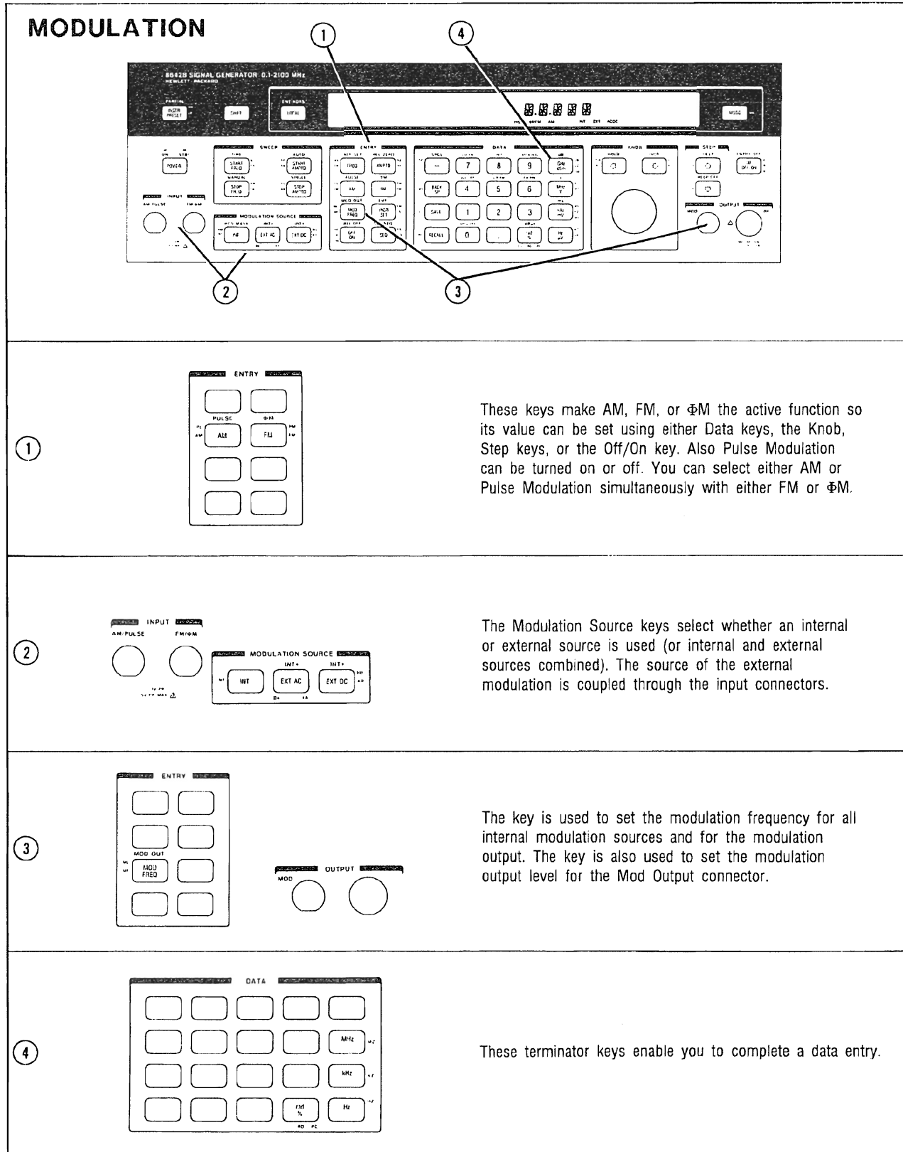
Figure 3-11. Modulation-Related Functions
