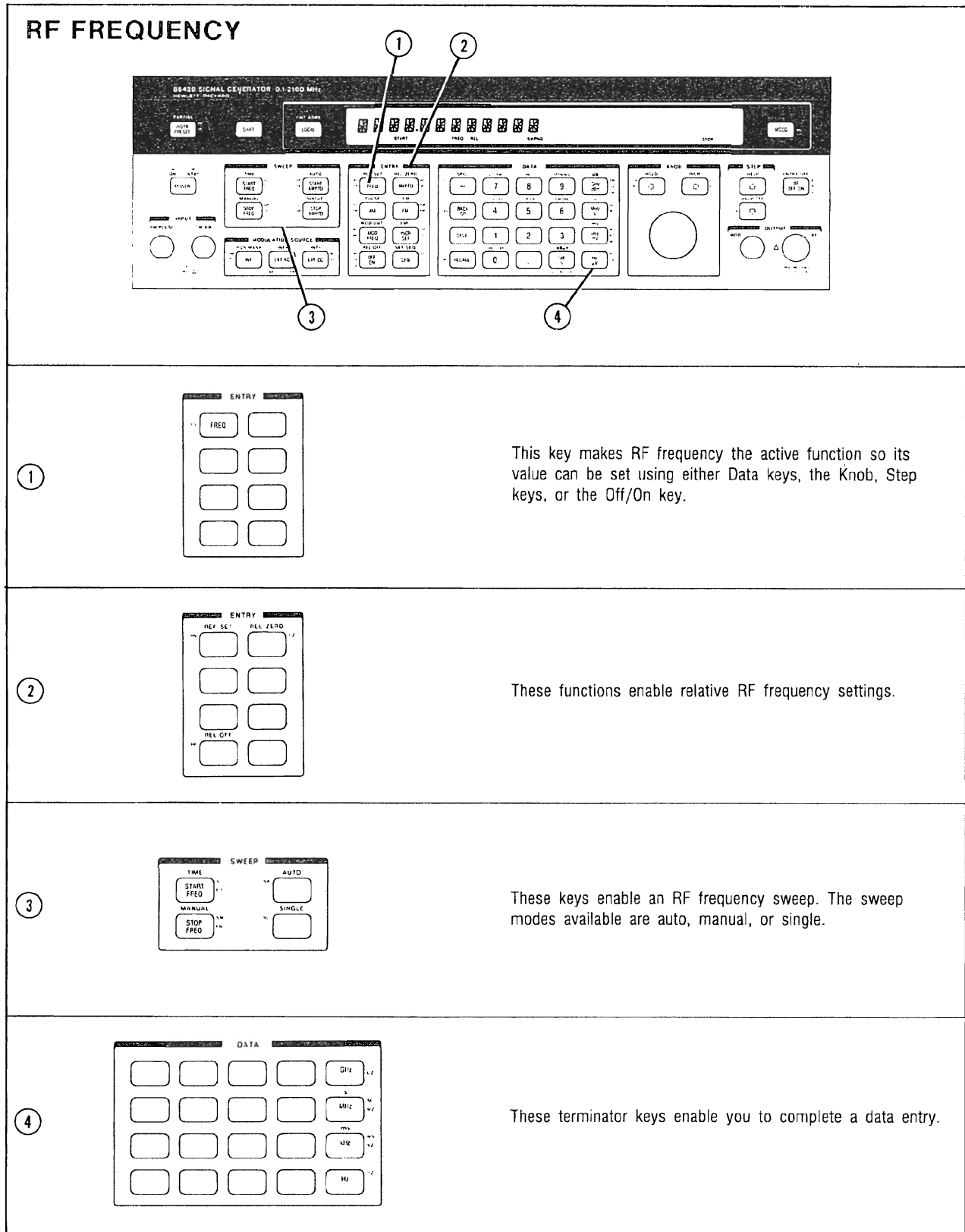
Figure 3-6. RF Frequency-Related Functions
