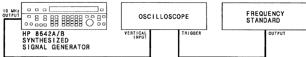
Figure 4-18. Internal Time Base Aging Rate Test Setup
