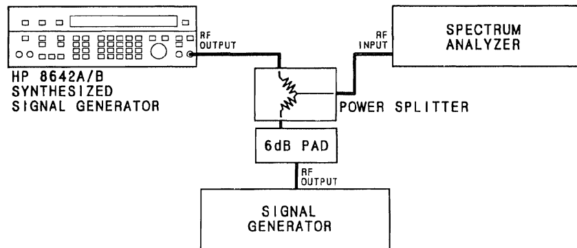
Figure 4-10. Intermodulation Test Setup
