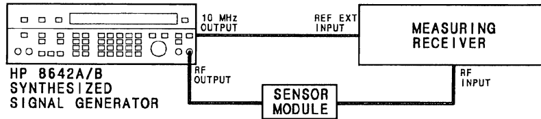
Figure 4-1. Level Accuracy and Flatness Test Setup
