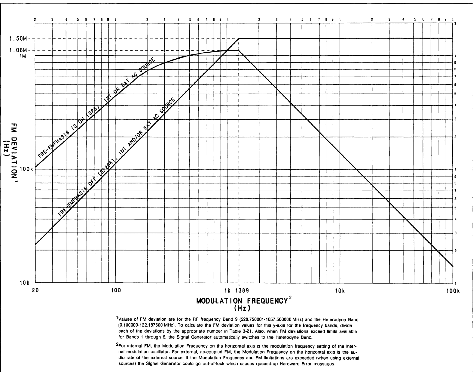
Figure 3-14. FM Deviation Limits with/without FM Pre-emphasis
