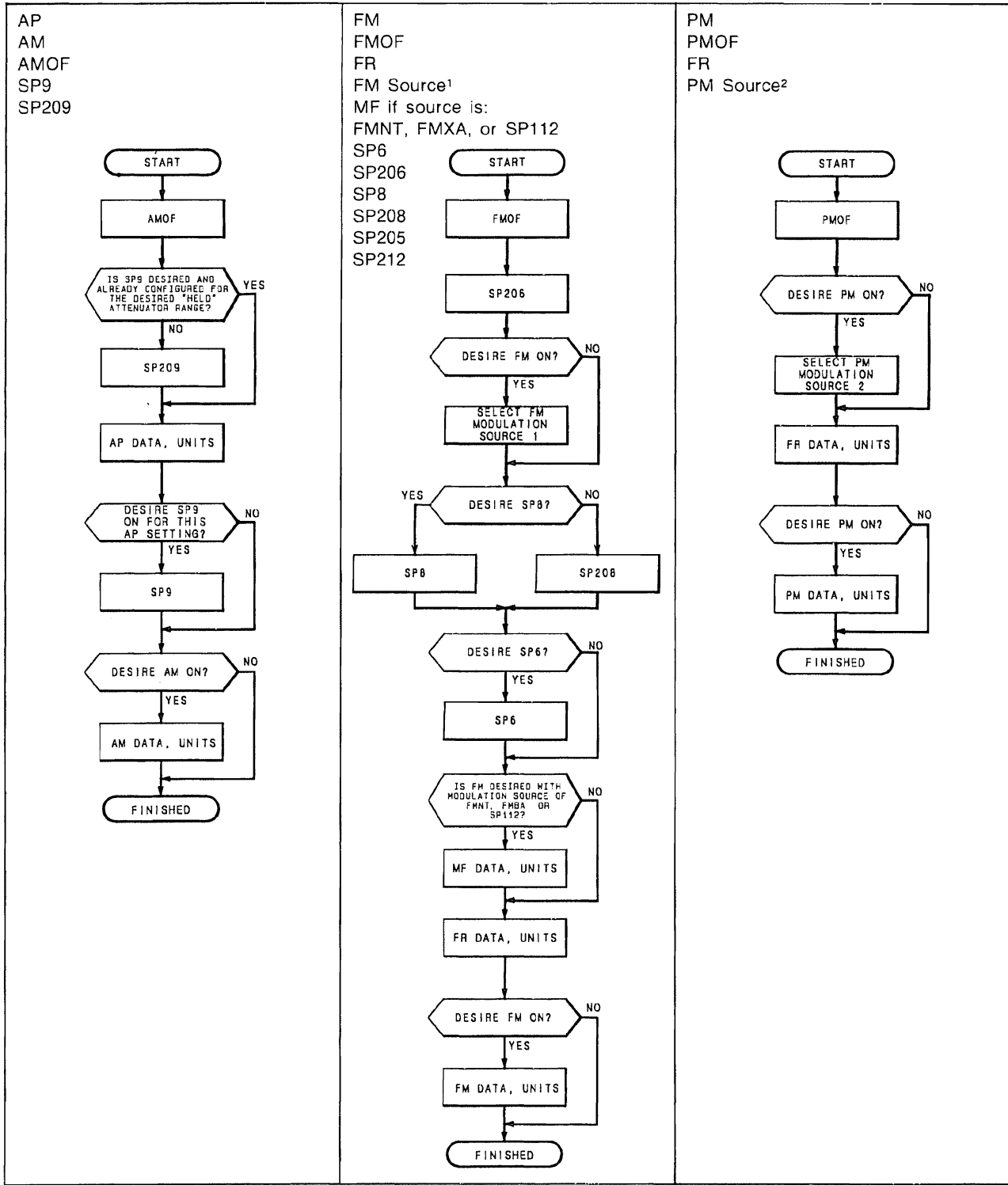
Figure 3-3. Flowcharts for Sequence Dependency
