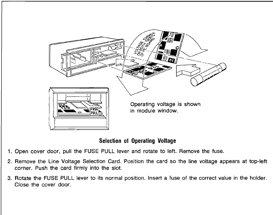
Figure 2-1. Line Voltage and Fuse Selection
