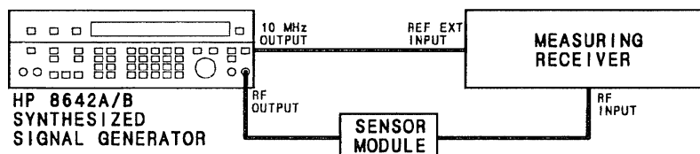
Figure 4-4. Residuals Test Setup
