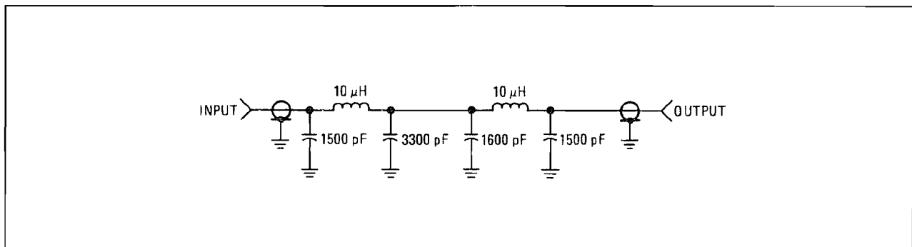
Figure 1-1. 1 MHz Low-Pass Filter
