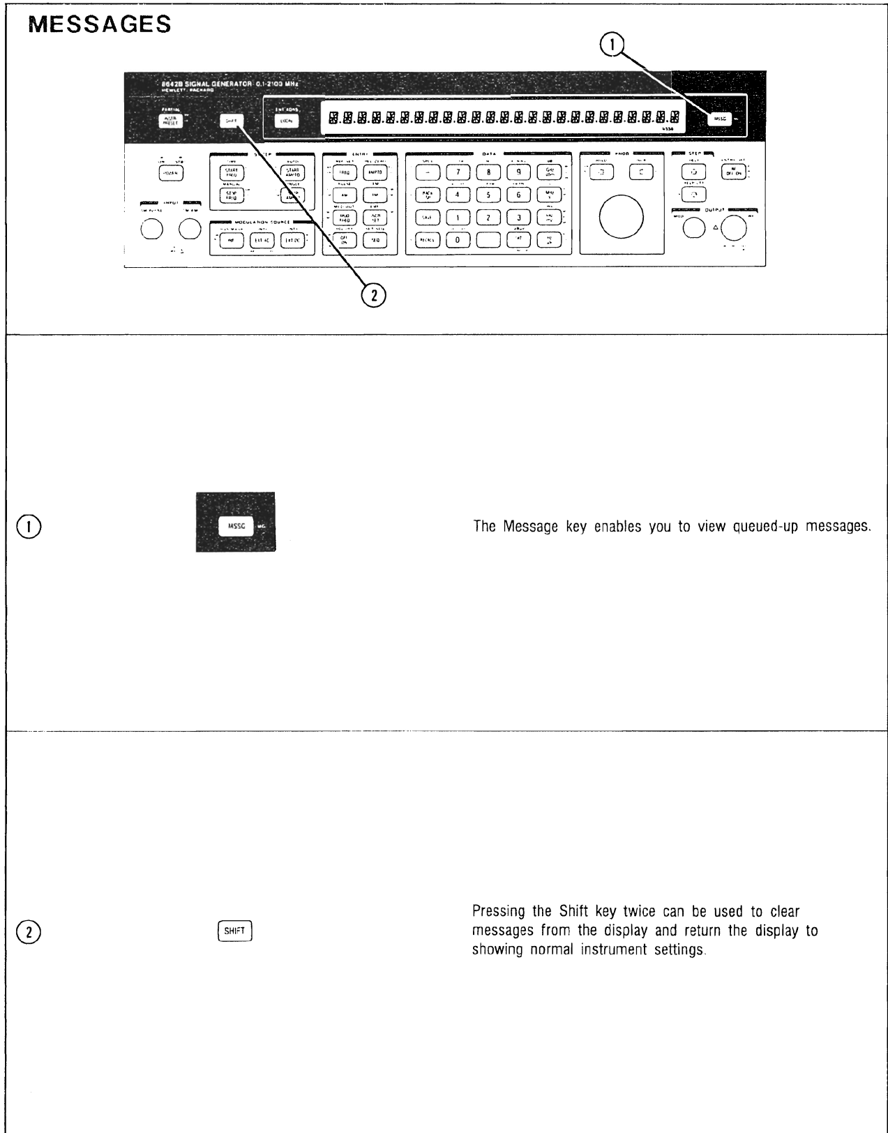
Figure 3-19. Message-Related Keys
