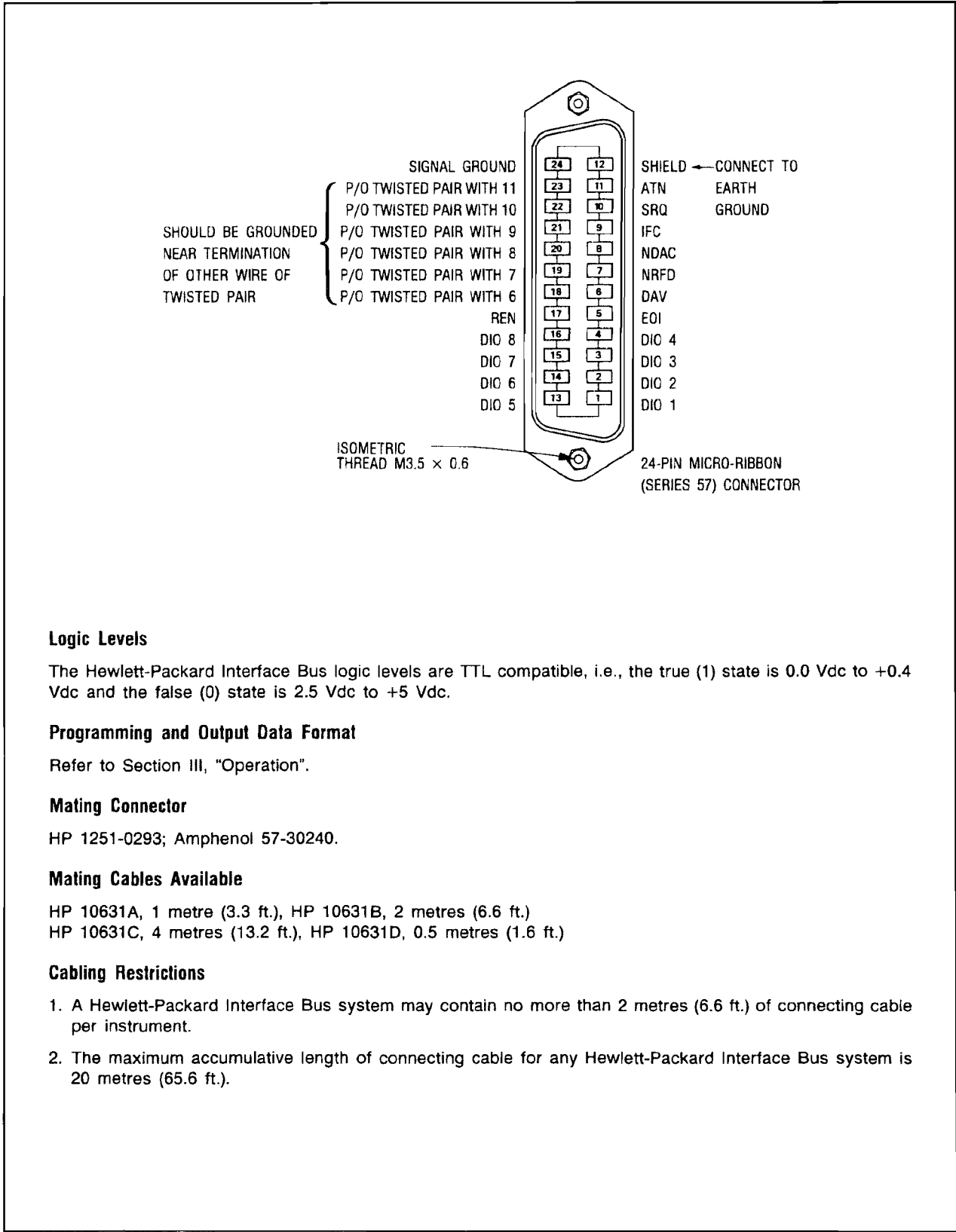
Figure 2-2. Hewlett-Packard Interface Bus Connections
