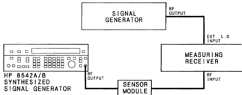
Figure 4-17. Residual Test Setup
