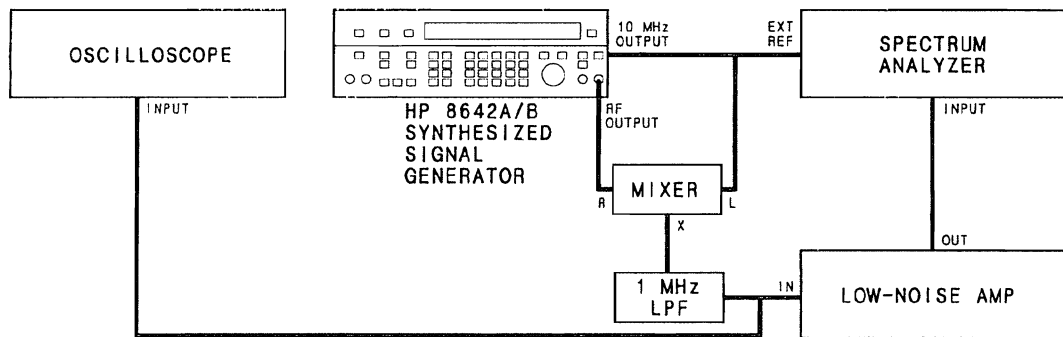
Figure 4-11. SSB Phase Noise Test Setup
