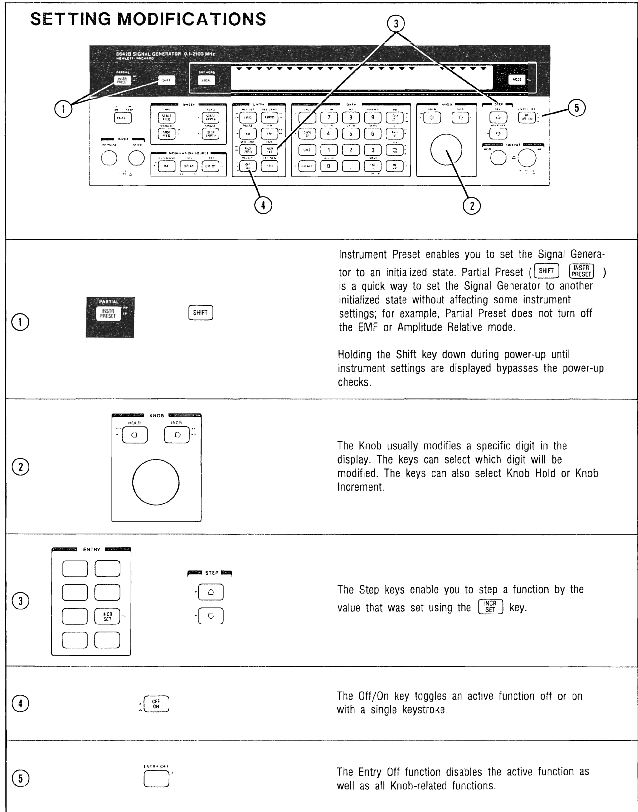
Figure 3-16. Functions Related to Modifying Settings
