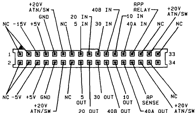
Figure 3M-1. Cable Plug W11P2 Signal Locator
