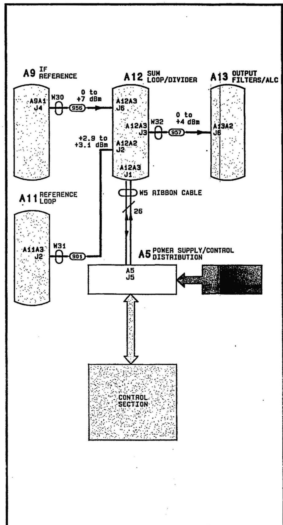
Figure 3J-100. A12 Sum Loop/Divider Module Diagnostics.
