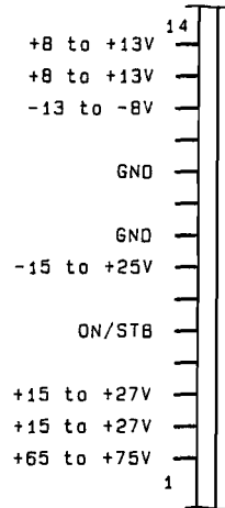
Figure 3B-1. Connector A17J1 Signal Locator (Solder-Side View)
