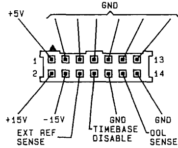
Figure 3F-4. Cable Plug W1P3 Signal Locator
