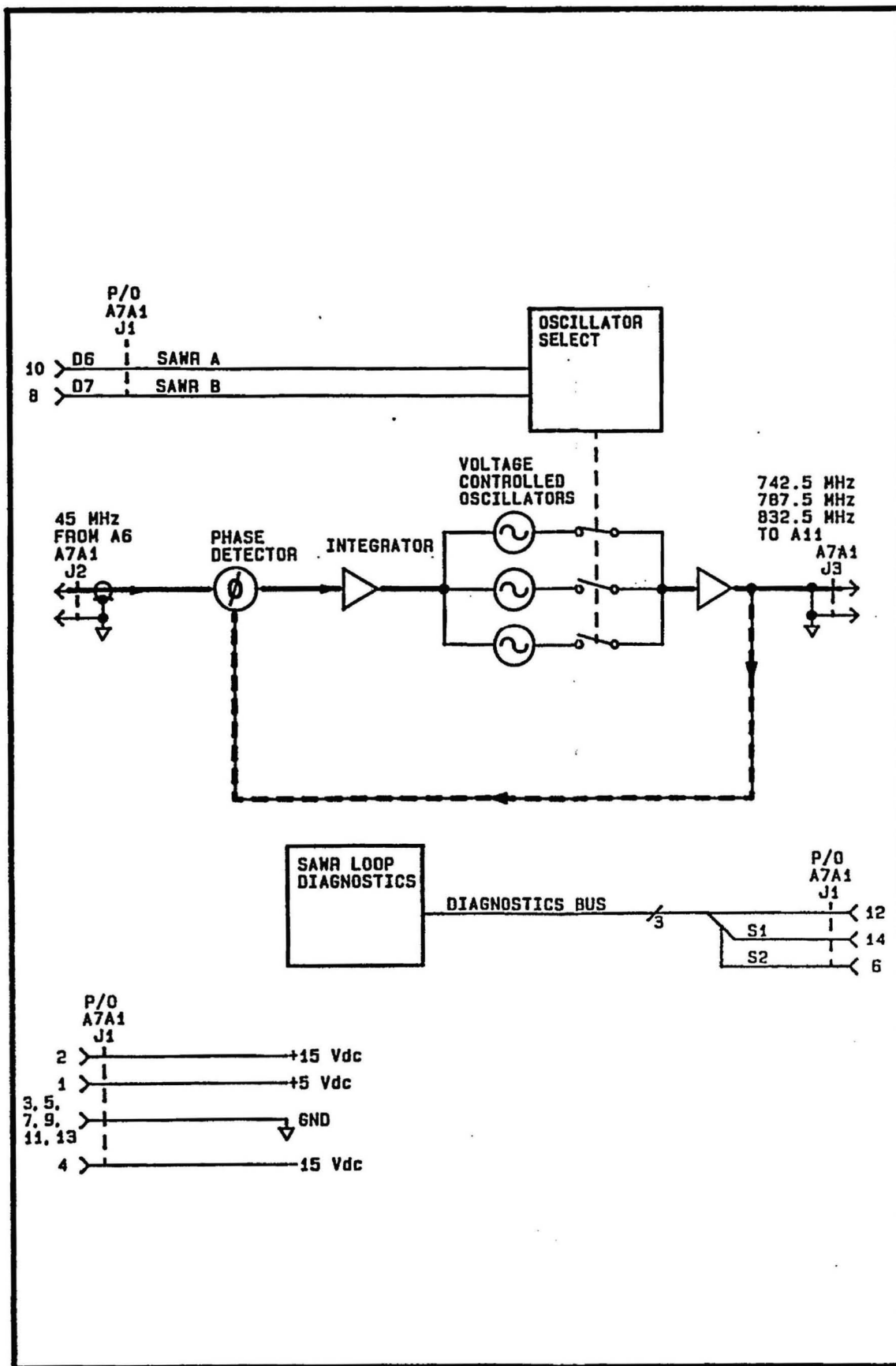
A7 MODULE SIMPLIFIED BLOCK DIAGRAM
