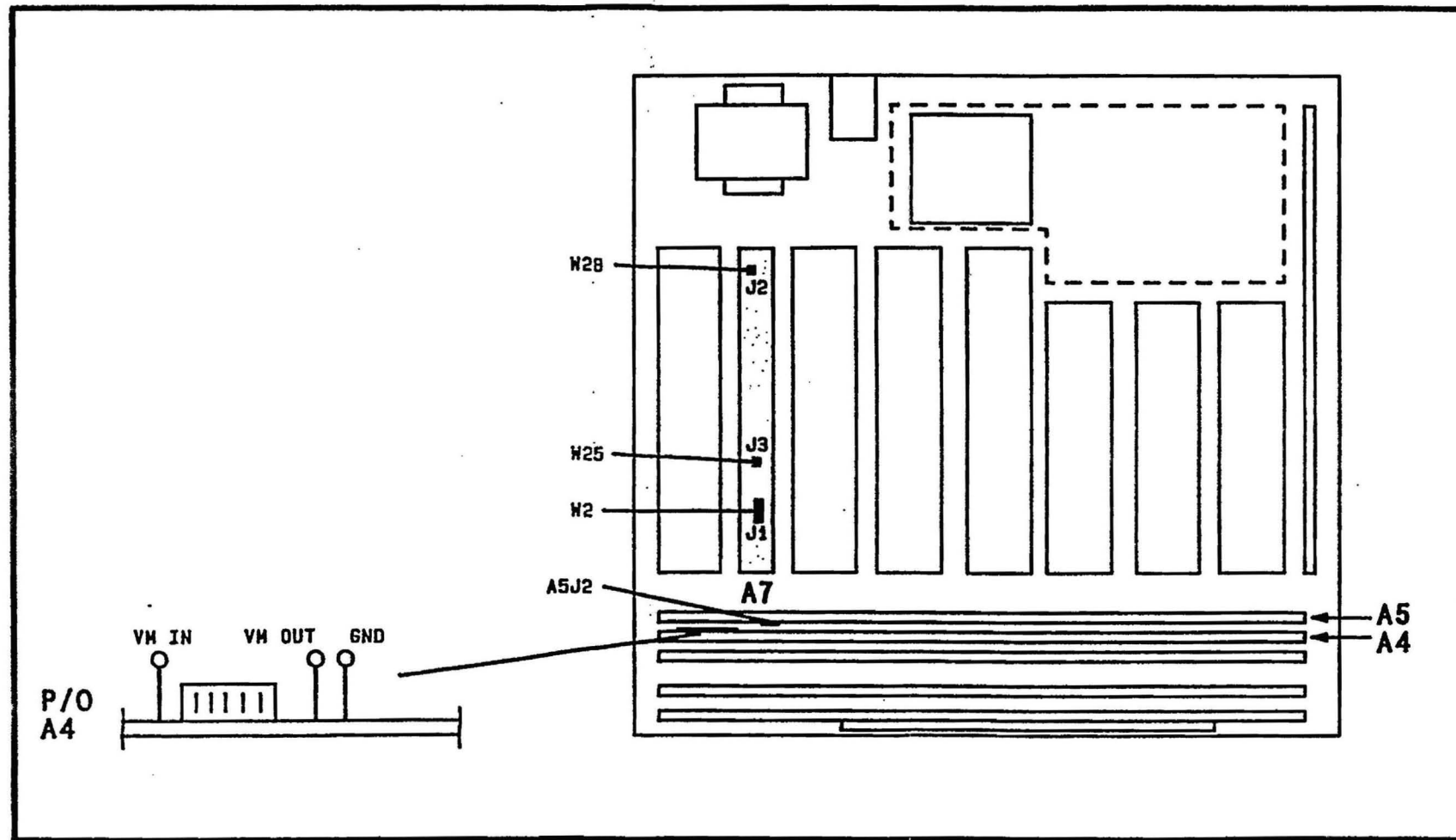
A7 MODULE CABLE CONNECTION LOCATOR
