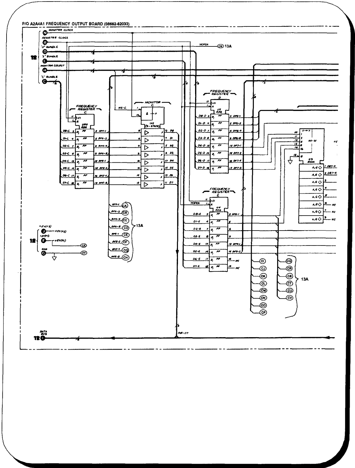
P/O Figure 8-339. P/O A2A4A1 Frequency Output Board Schematic
