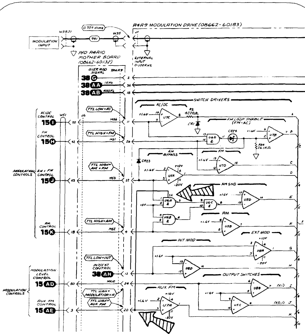
P/O SERVICE SHEET 40 P/O Figure 8-539. A4A9 Modulation Drive Schematic "AUX FM" Configured in the ON Position
