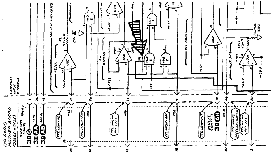
P/O Service Sheet 40, showing "AUX FM" configured in the ON position.
