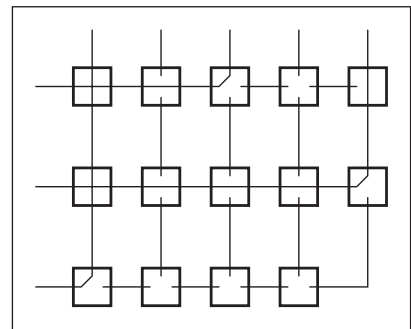
Figure 5. Cross-point matrix
