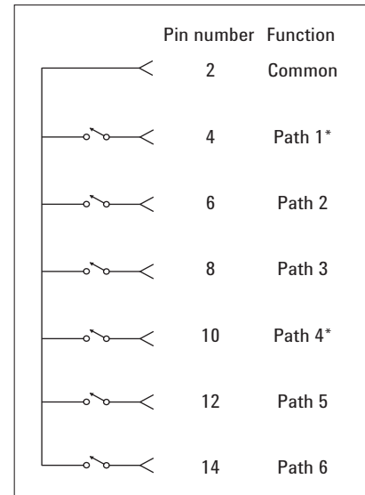
Figure 7. Pin function diagram
