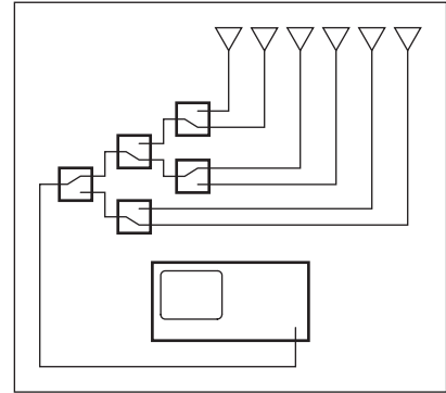
Figure 3. Tree matrix
