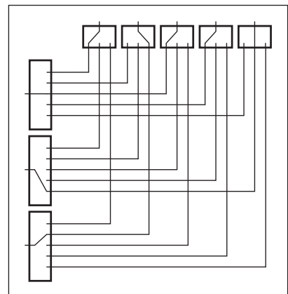
Figure 6. Full access matrix
