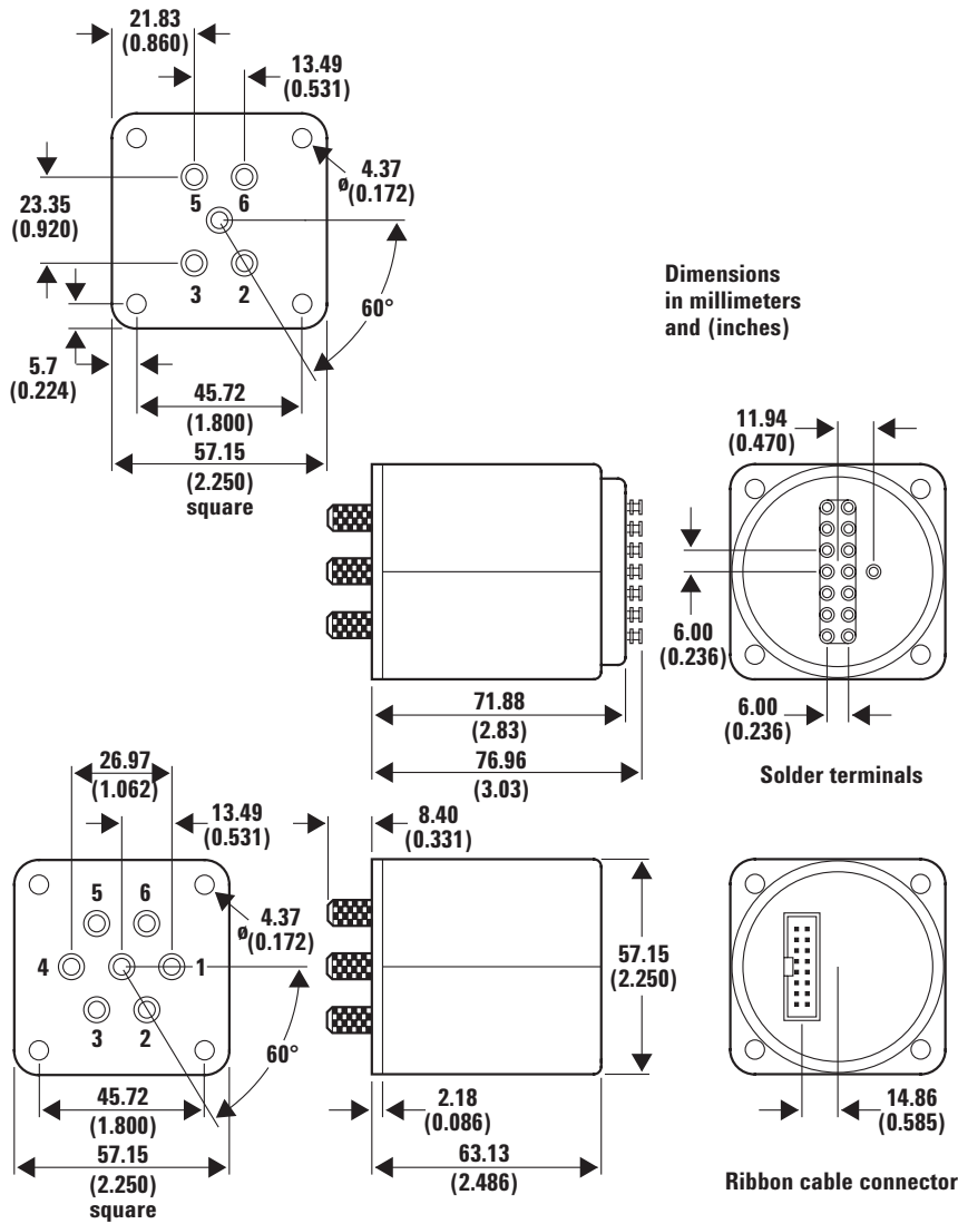
Figure 13. Mechanical dimensions
