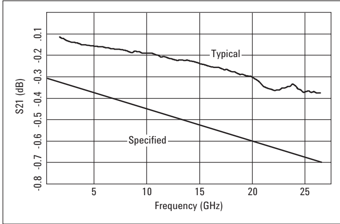
Figure 6. Insertion loss
