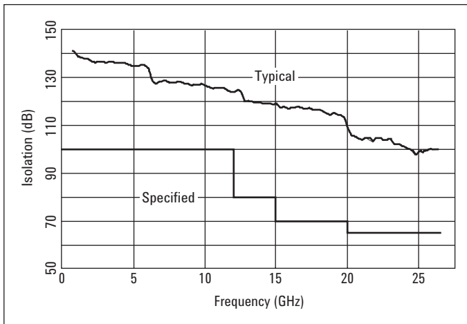
Figure 7. Isolation
