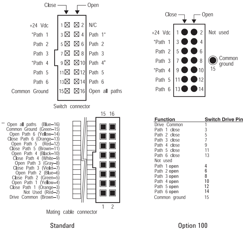
Figure 8. Drive connection diagrams
