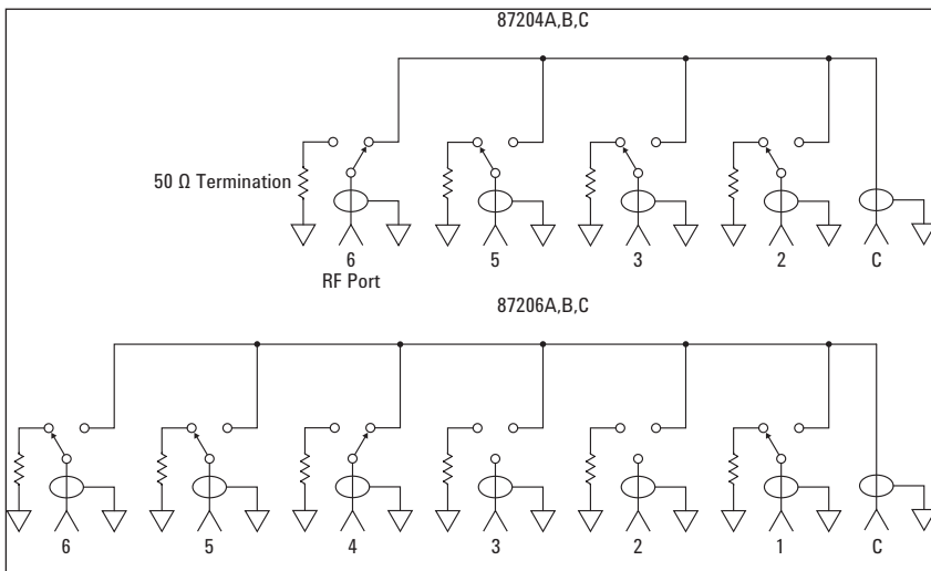
Figure 1. Keysight 87204A/B/C and 87206A/B/C simplified schematics
