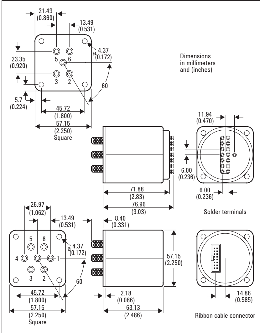
Figure 9. Product outlines
