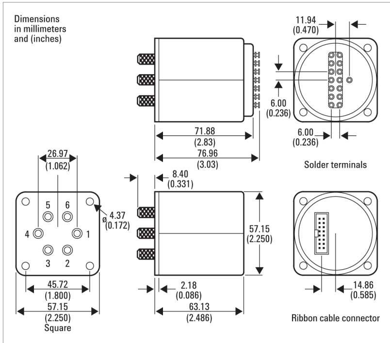
Figure 7. Product outline
