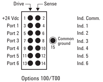
Figure 8. Drive connection diagrams
