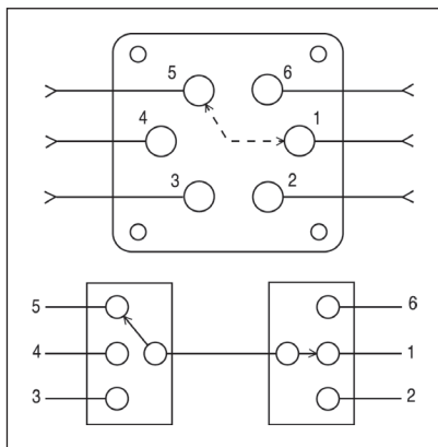
Figure 3. Matrix switch configured for a 3 x 3 blocking application (RF Path 5 to 1 shown)
