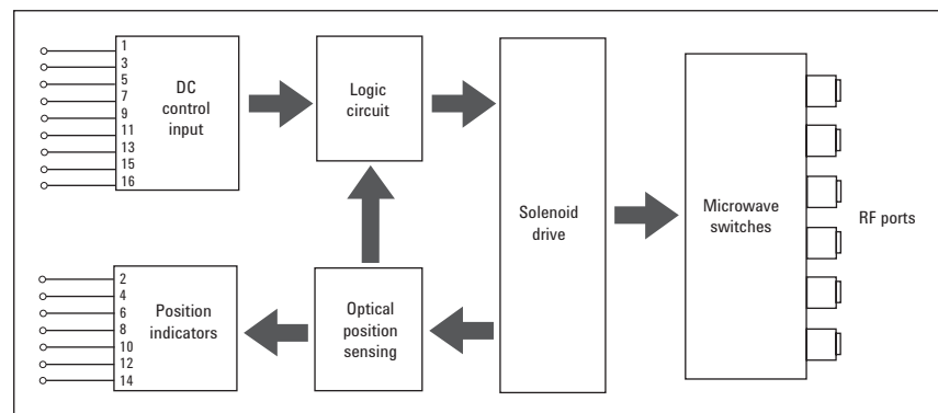
Figure 4. Keysight 87406B block diagram
