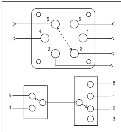
Figure 2. Matrix switch configured for a 2 x 4 blocking application (RF Path 5 to 2 shown)
