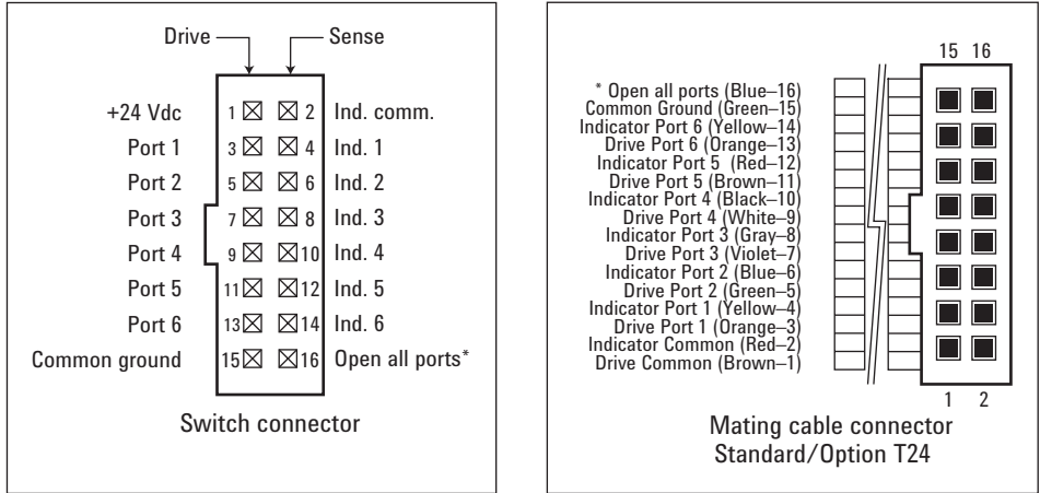
Figure 6. J1 connector configuration
