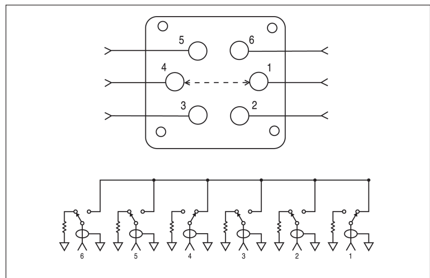
Figure 1. Keysight 87406B connection diagram and simplified schematic (RF path 4 to 1 shown)
