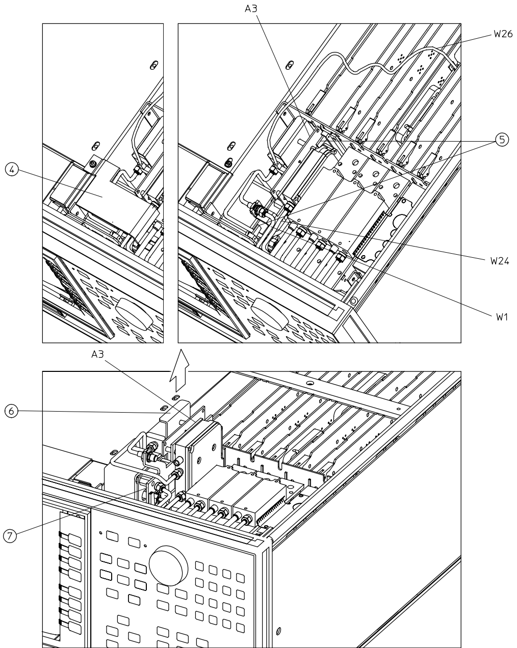
Figure 2 A3 Source Assembly Removal
