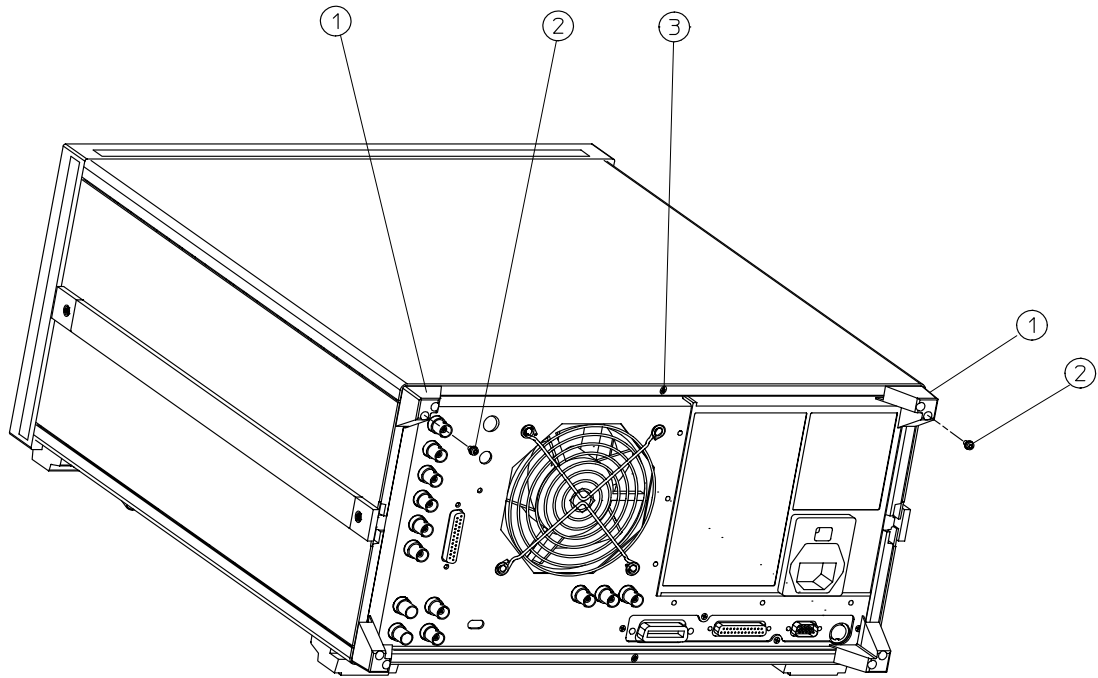
Figure 1 Cover and Feet Removal
