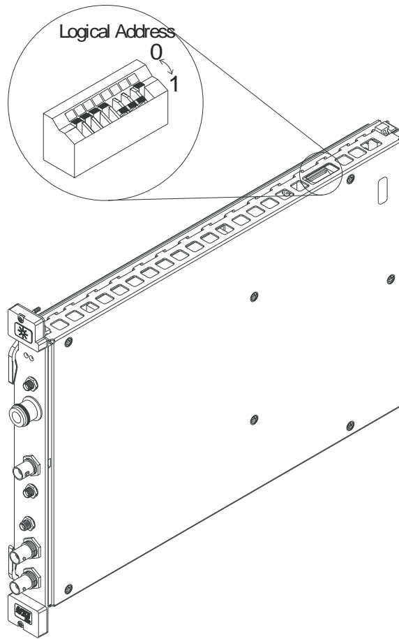
Figure 1-1 89605 Input module -- address 14 (000 1110)
