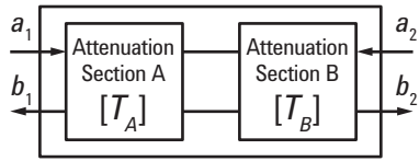
Figure 6. two individual pads connection
