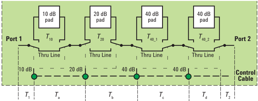
Figure 5. 8496B individual pads connection
