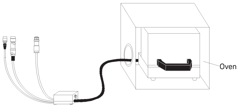
Figure 1-2 N1424A/B/C in an Environmental Test Oven
