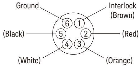
Wire Side of Interlock Cable
