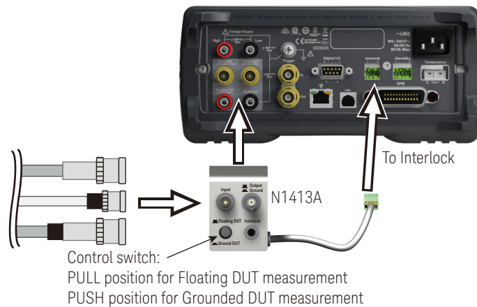
Figure 3-5 Connecting the Product
