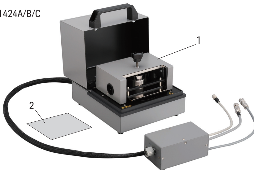
Figure 1-1 Product Overview
