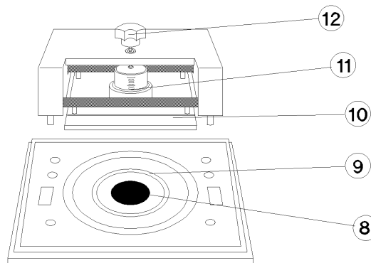
Figure 1-5 Main/Guard/Upper Electrode
