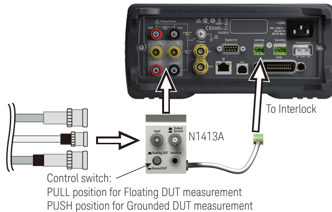
Figure 2-2 Connecting the Product
