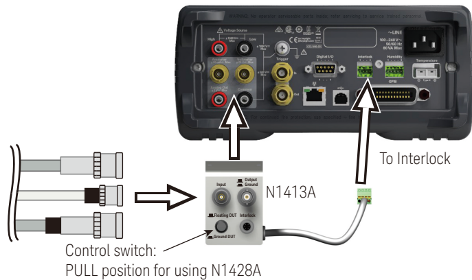
Figure 4-2 Connecting the Product
