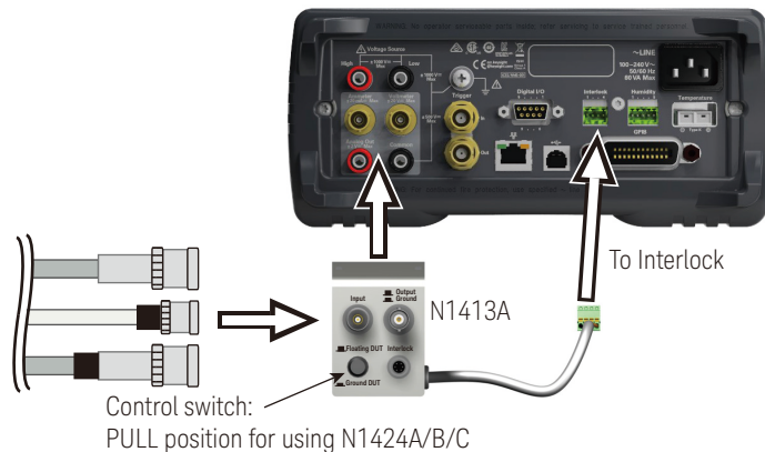
Figure 1-4 Connecting the Product
