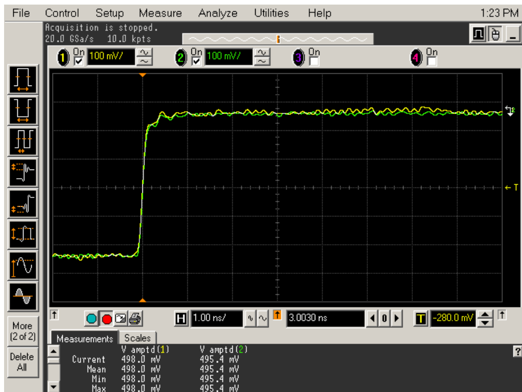
Figure 6 Overlapping Waveforms
