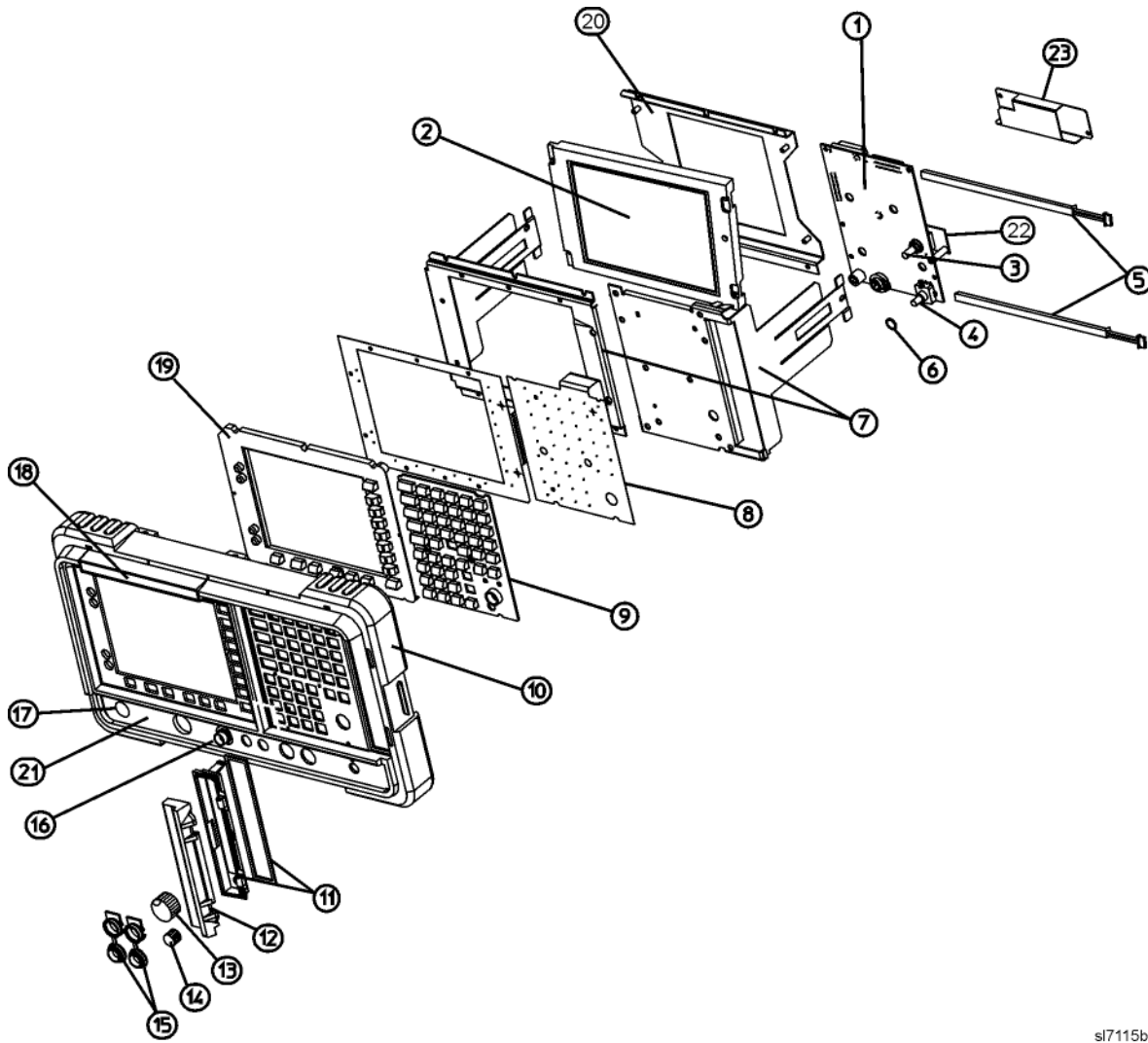
Figure 5-3 Front Panel Parts
