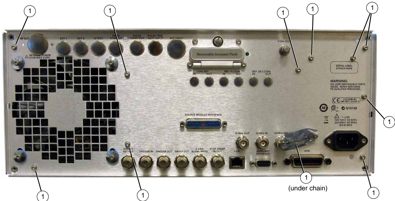
Figure 3-57 Rear Panel Removal
