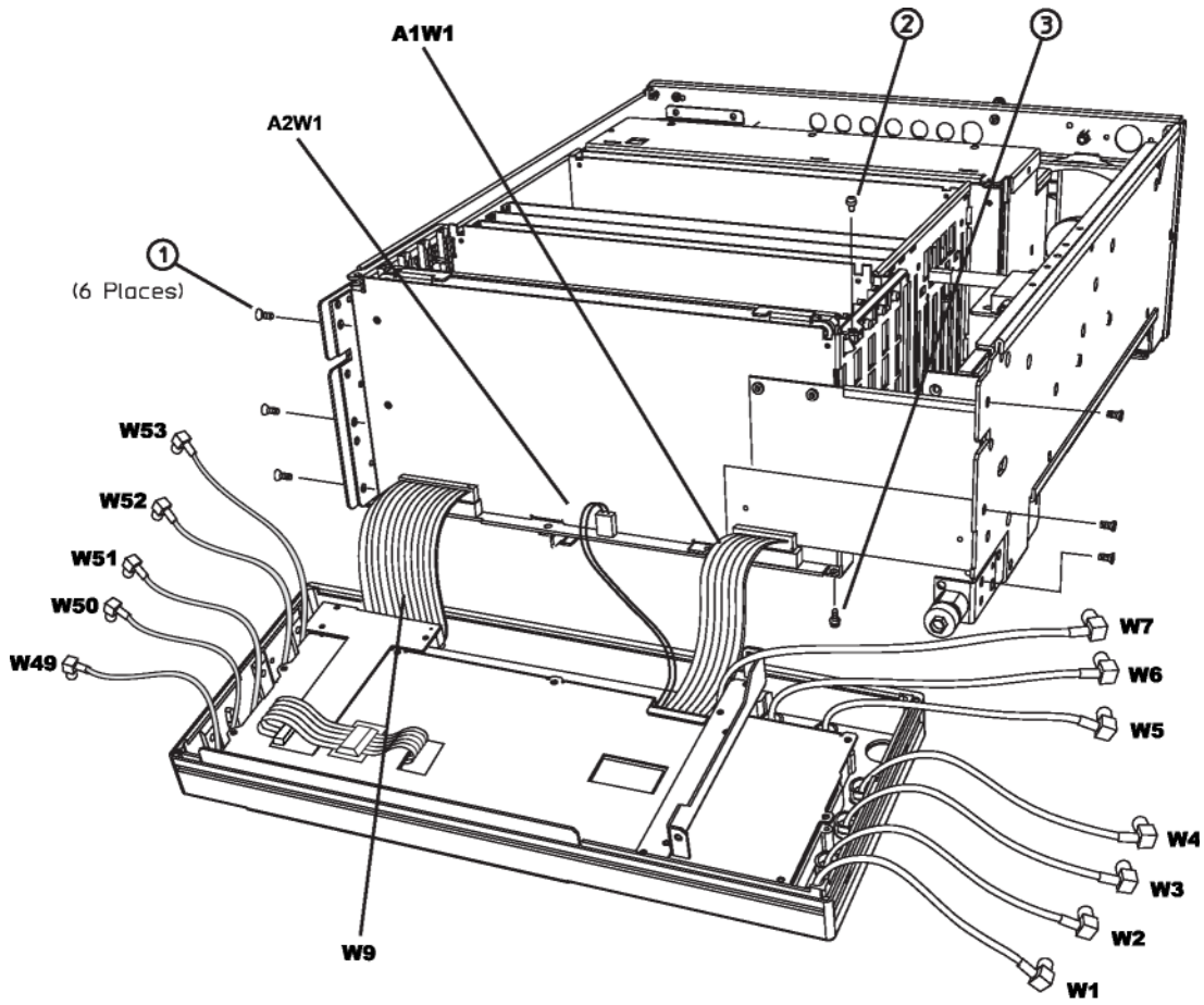
Figure 3-4 Front Panel Removal with serial prefixes > US/MY5XXX3XXX
