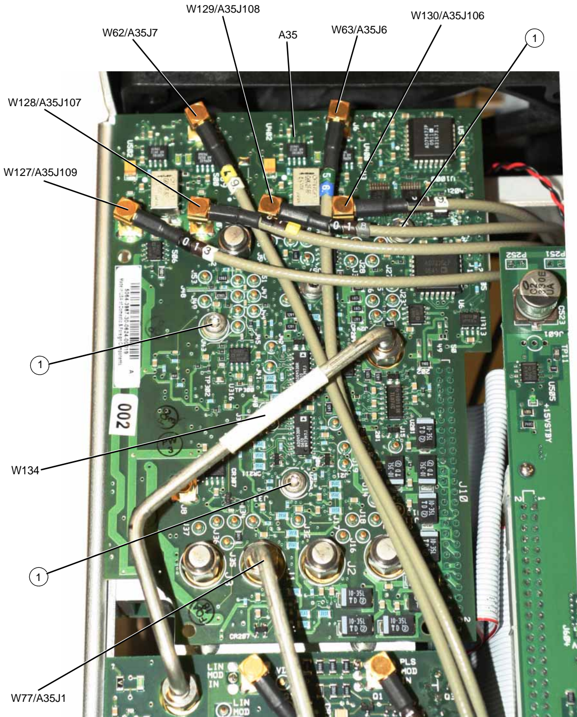
Figure 3-61 A35 3–20 GHz I/Q MOD (E8267D only - Standard or with Option 016) (Serial Prefixes \geq US4722/MY4722)
