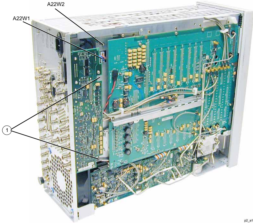
Figure 3-58 Rear Panel Removal (Option 1EM)
