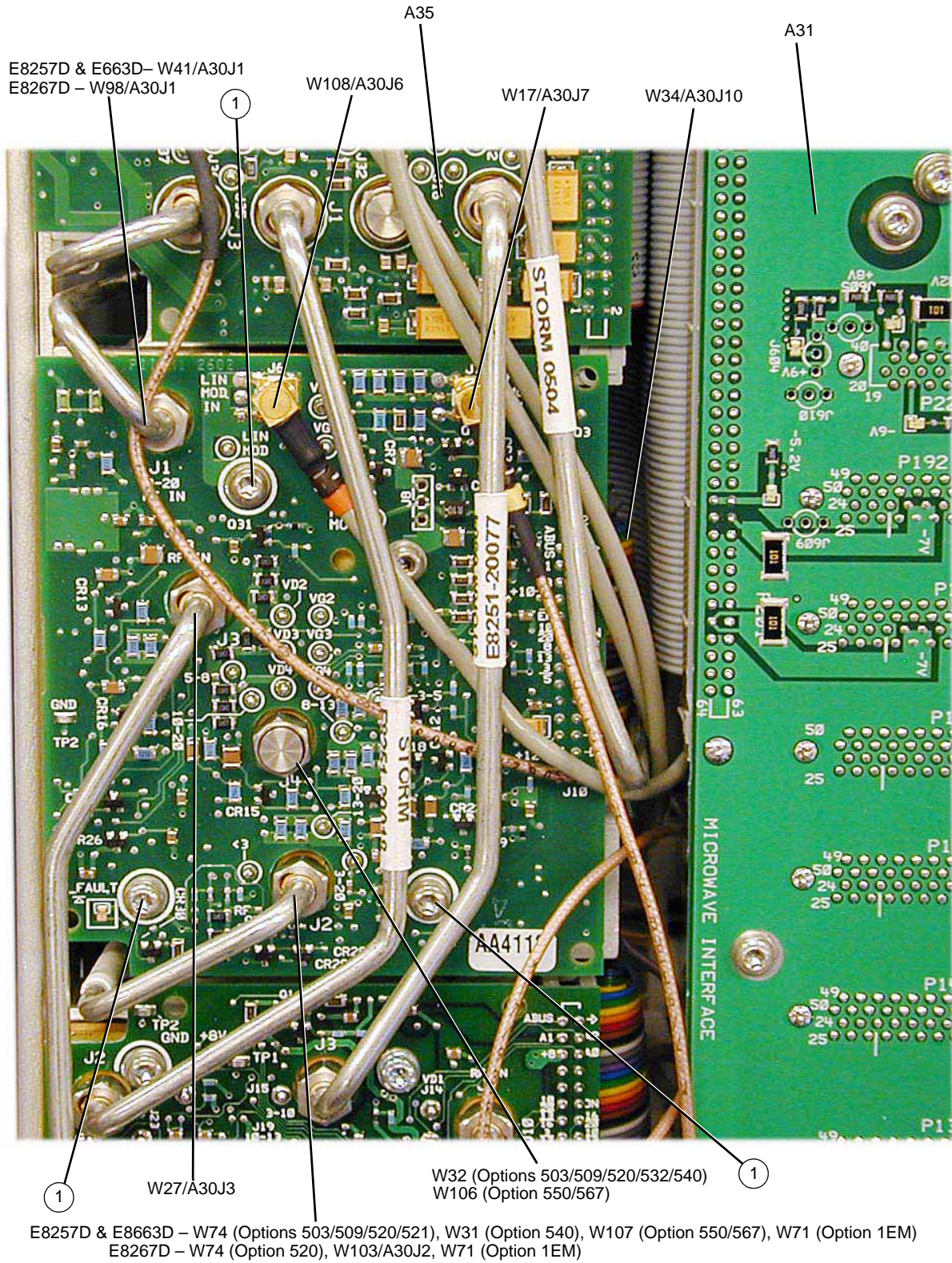
Figure 3-51 A30 Modulator Filter
