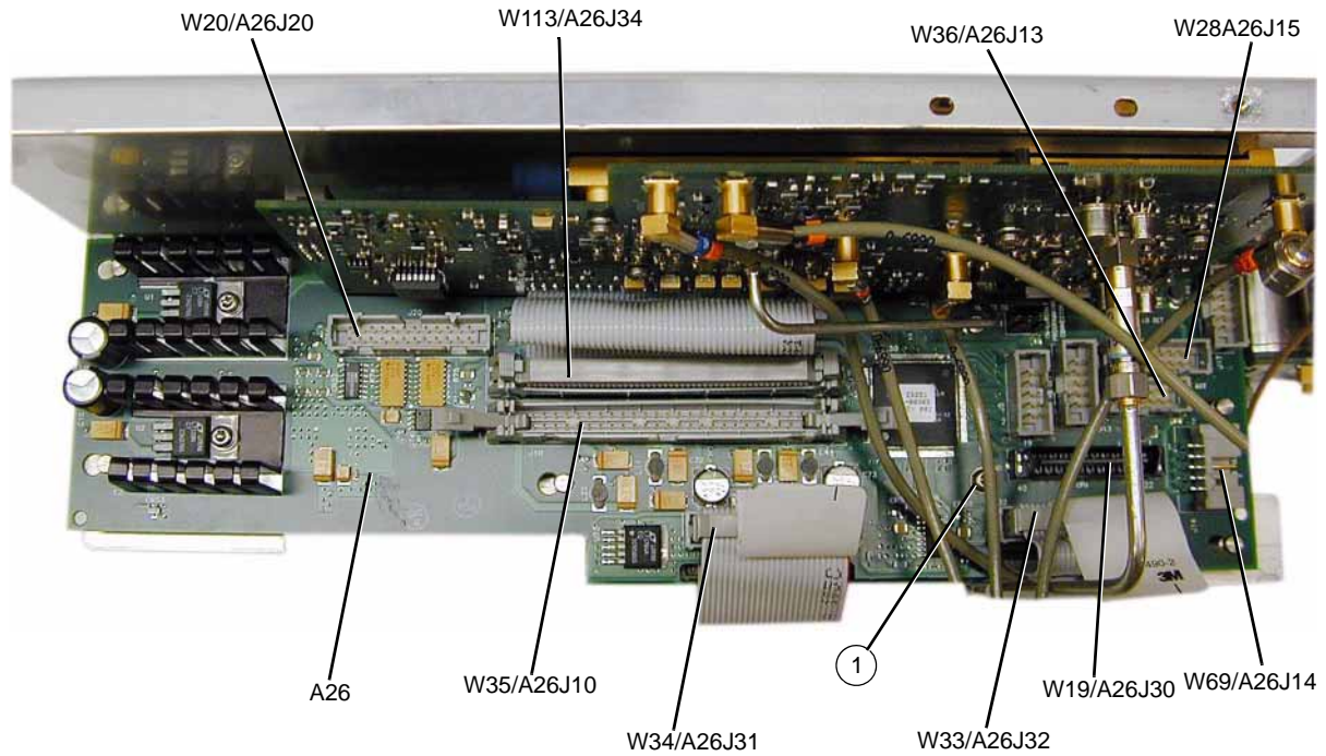
Figure 3-46 A26 MID (E8267D)
