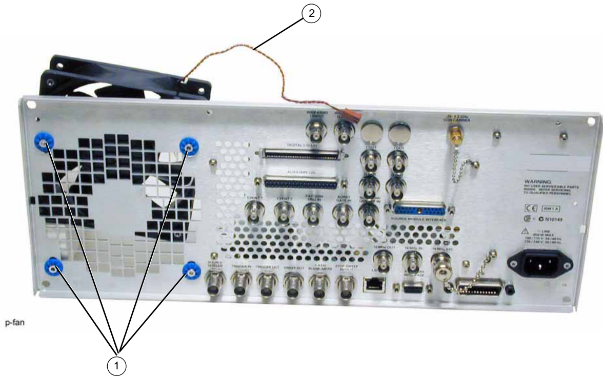
Figure 3-76 B1 Fan
