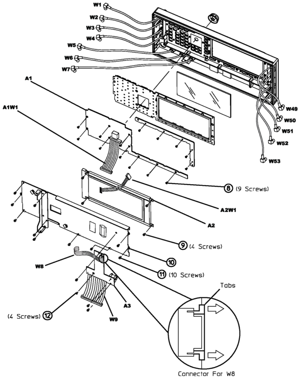
Figure 3-6 A1 Keyboard Removal with serial prefixes > US/MY5XXX3XXX
