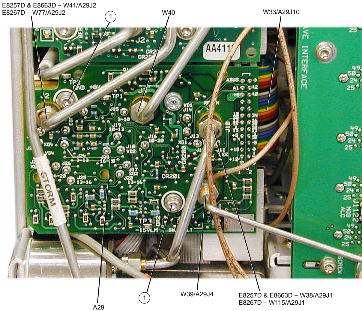
Figure 3-50 A29 20 GHz Doubler
