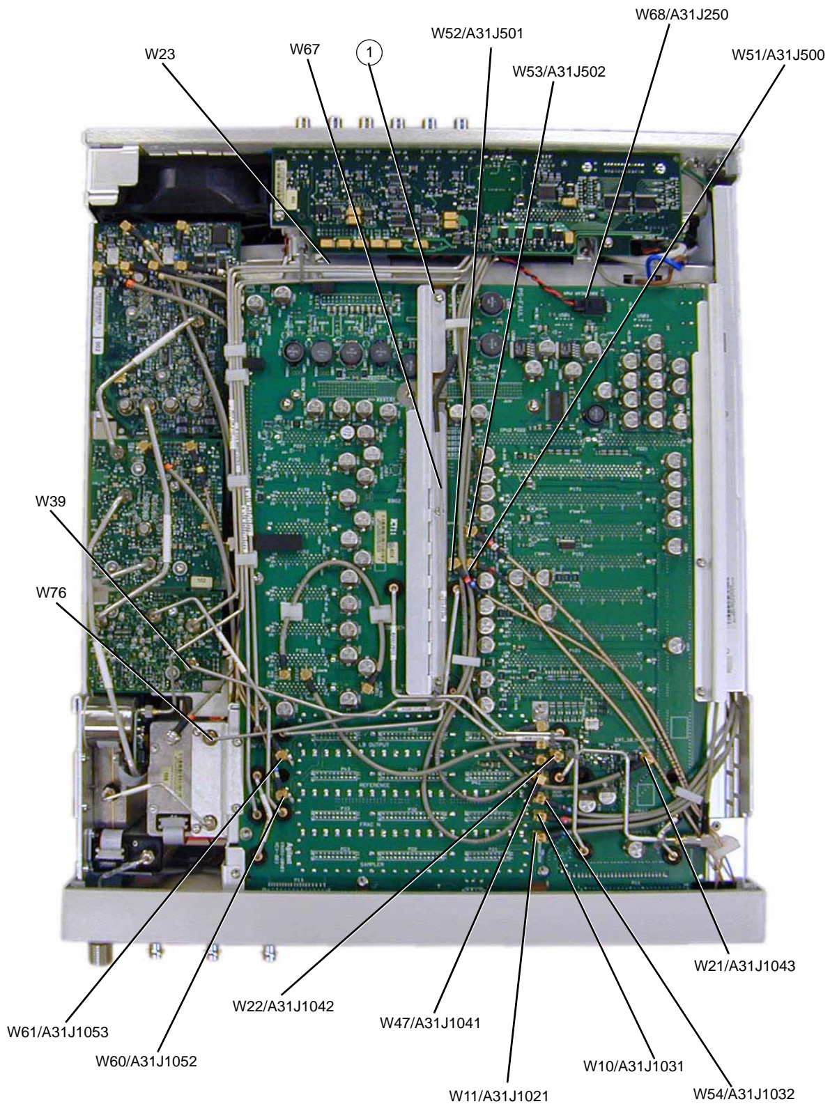
Figure 3-53 A31 Motherboard (E8267D)
