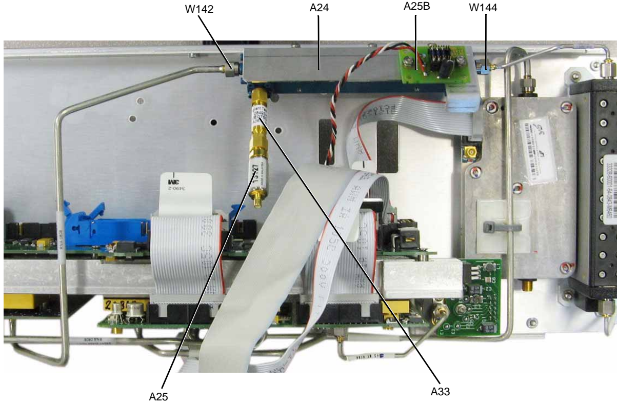
Figure 3-32 A24 20 GHz Highband Coupler (Option 521 - Option 1EM)
