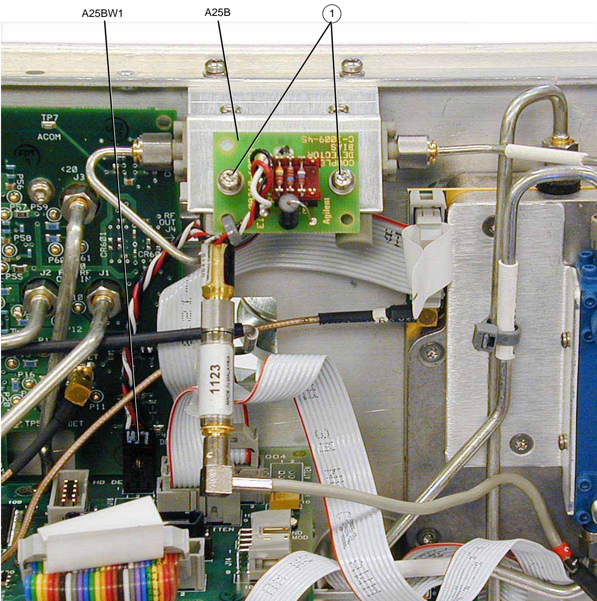
Figure 3-44 A25B Highband Detector Bias Board
