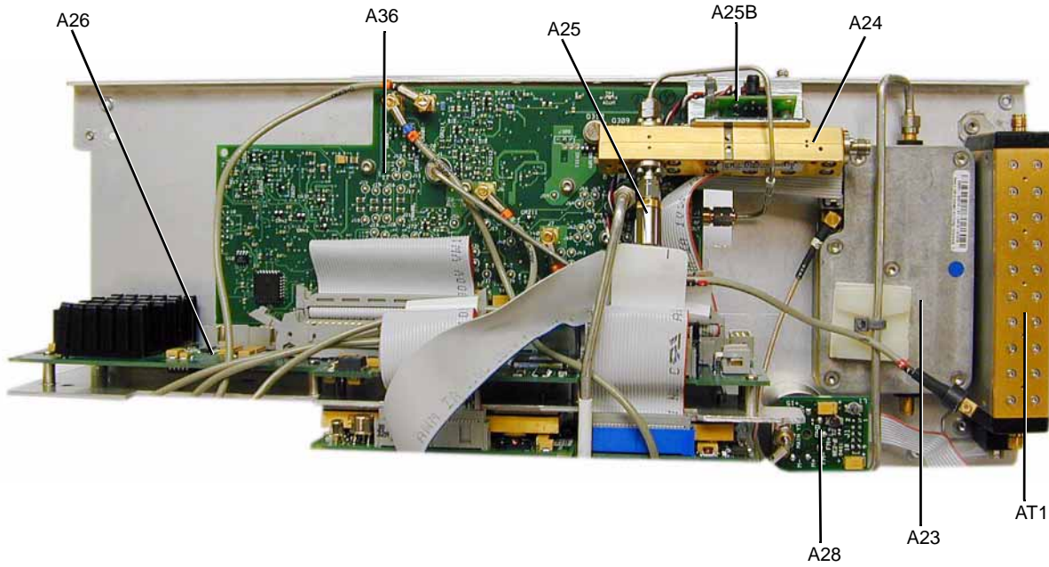
Figure 2-11 Assemblies from a Microcircuit Deck View (E8267D Option 520)
