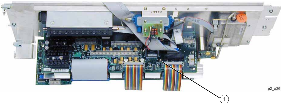
Figure 2-27 E8267D Microcircuit Interface Deck Top View
