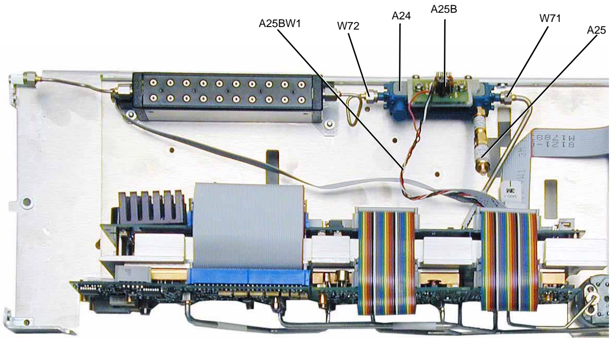
Figure 3-34 A24 40 GHz Highband Coupler (Option 540 – Option 1EM)
