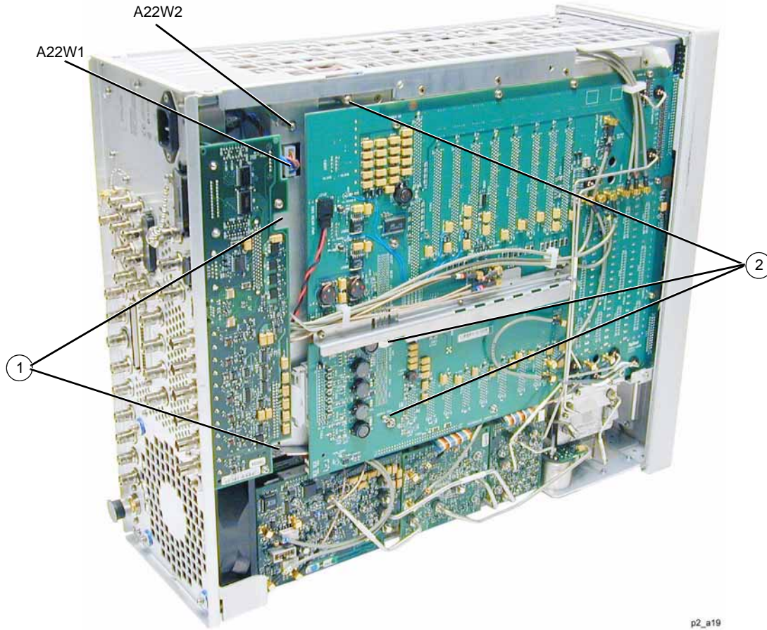
Figure 3-24 A19 Power Supply Removal
