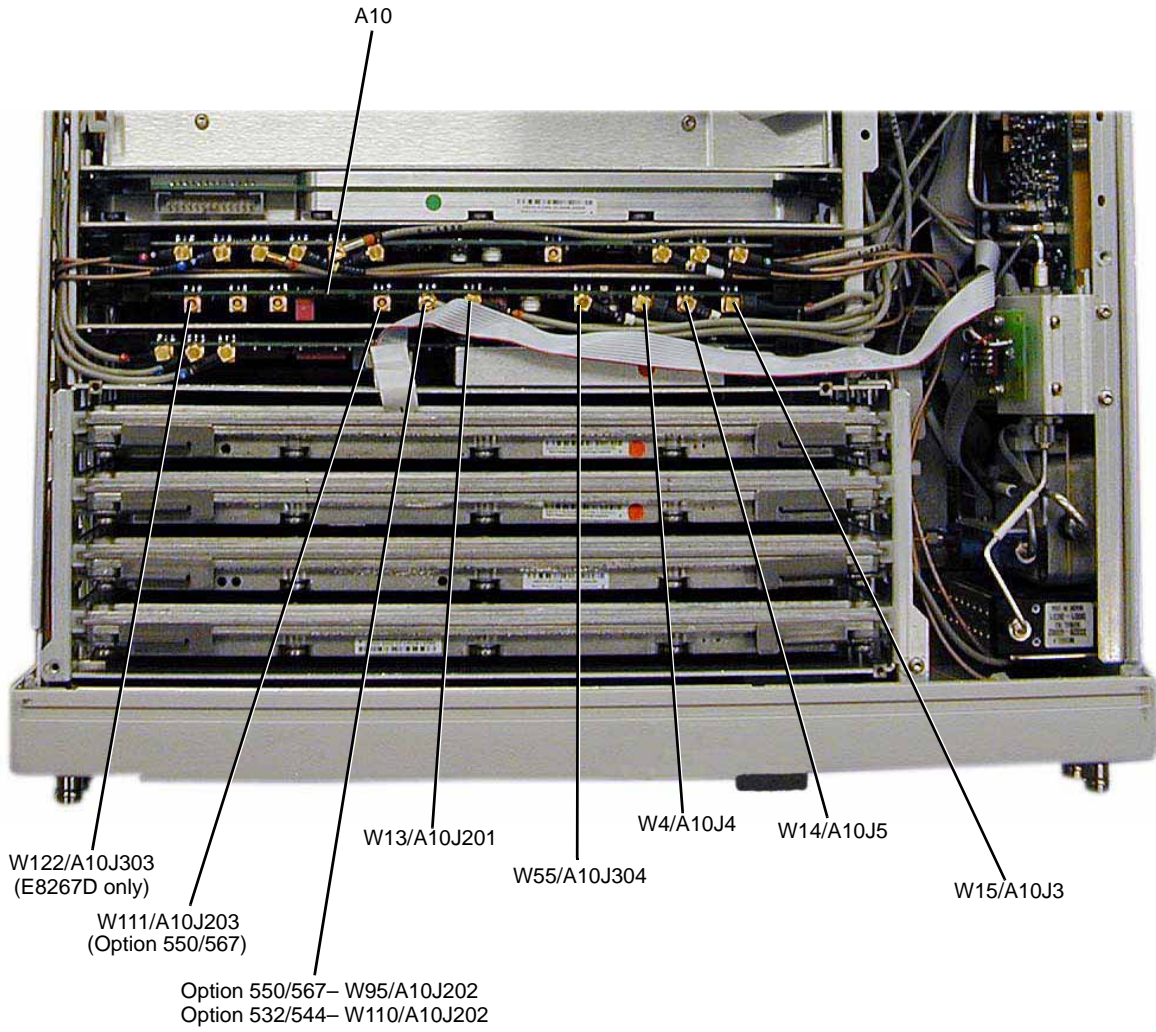
Figure 3-15 A10 ALC
