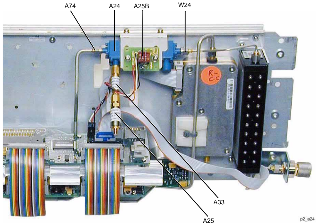
Figure 3-30 A24 20 GHz Highband Coupler (Options 503, 509 and 520 – Option 1EM)
