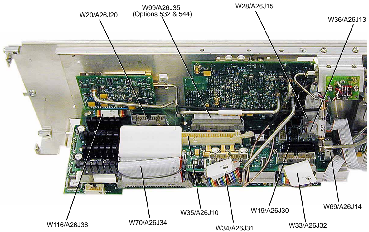
Figure 3-46 A26 MID (E8267D)
