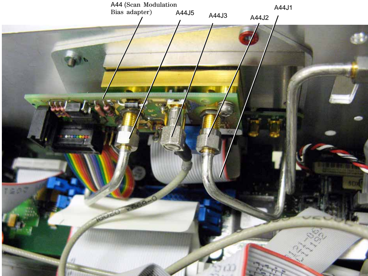
Figure 3-71 A44 Scan Modulation Bias Adapter
