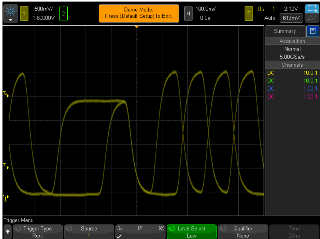
Figure 37 Triggering on positive runts.
