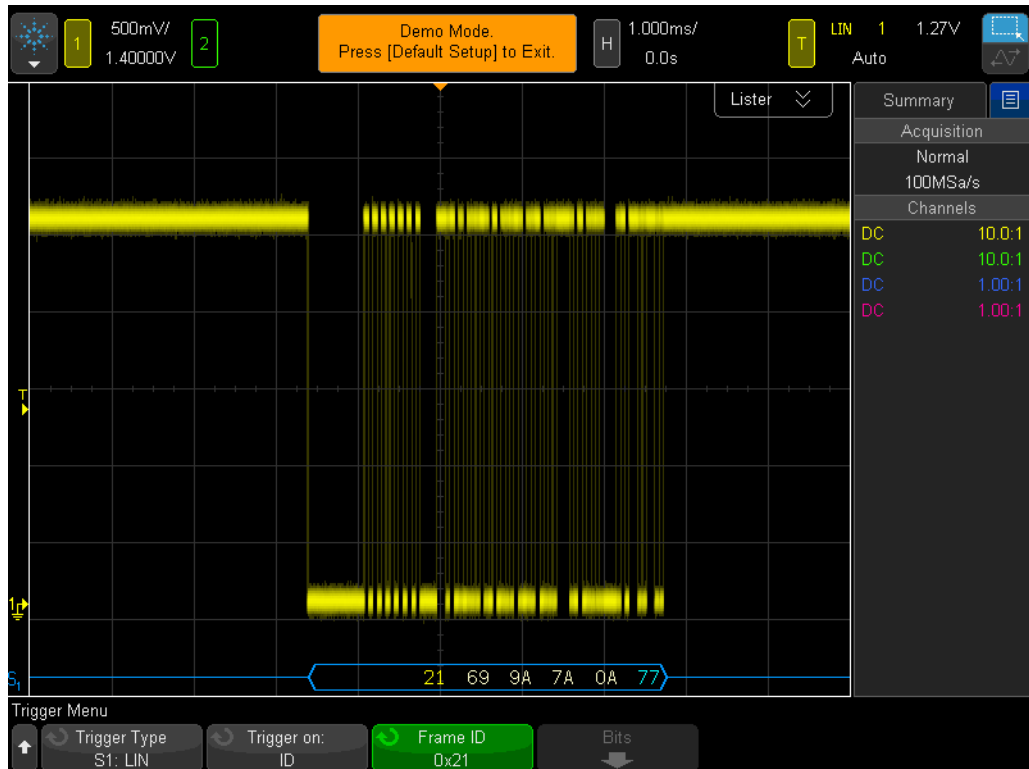
Figure 75 While triggering on LIN frame = 21_{\text{HEX}} , the scope's hardware-based decoding reveals parity bit errors in the frame ID field.
