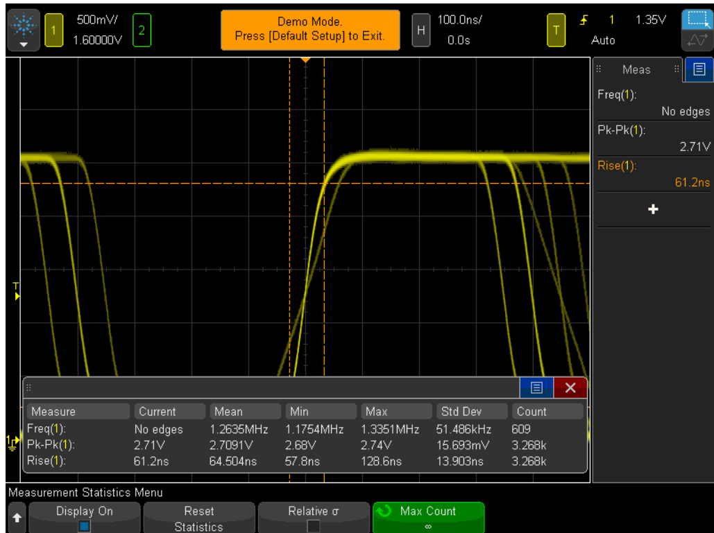
Figure 32 The scope's measurement statistics shows the range of rising edge speeds on this signal.
