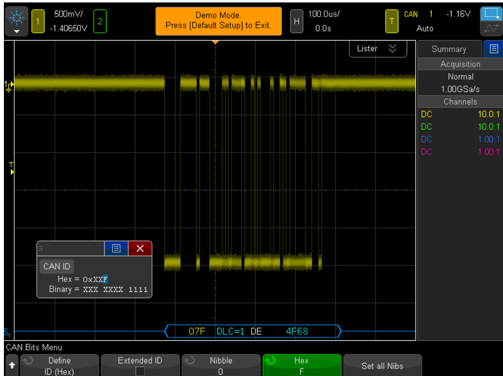
Figure 69 While triggering on CAN data frame = 07F_{\text{HEX}} , the scope’s hardware-based decoding reveals infrequent error conditions.
