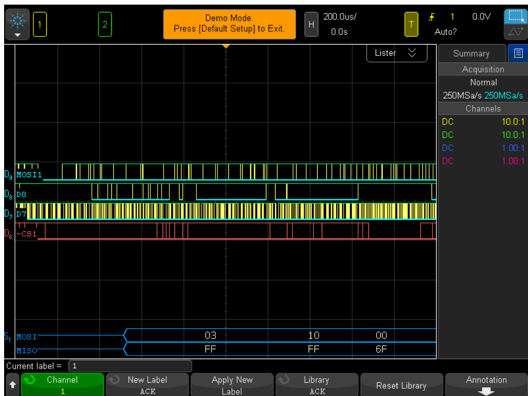
Figure 56 Decoding a 4-wire SPI serial bus.
