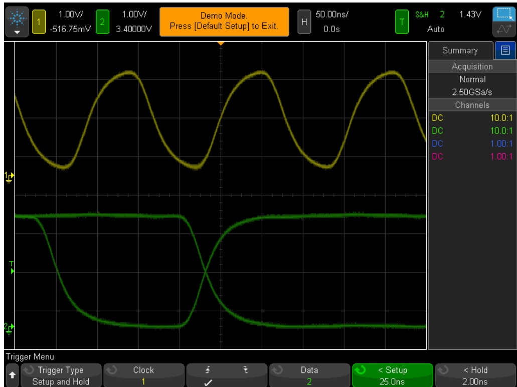
Figure 42 Triggering the scope on just setup time violations of less than 25 ns.
