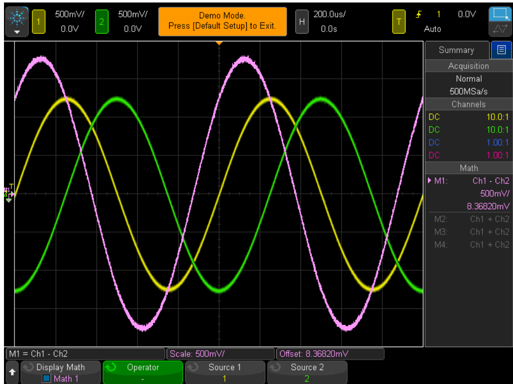
Figure 11 Using waveform math to subtract channel-2 from channel-1.
