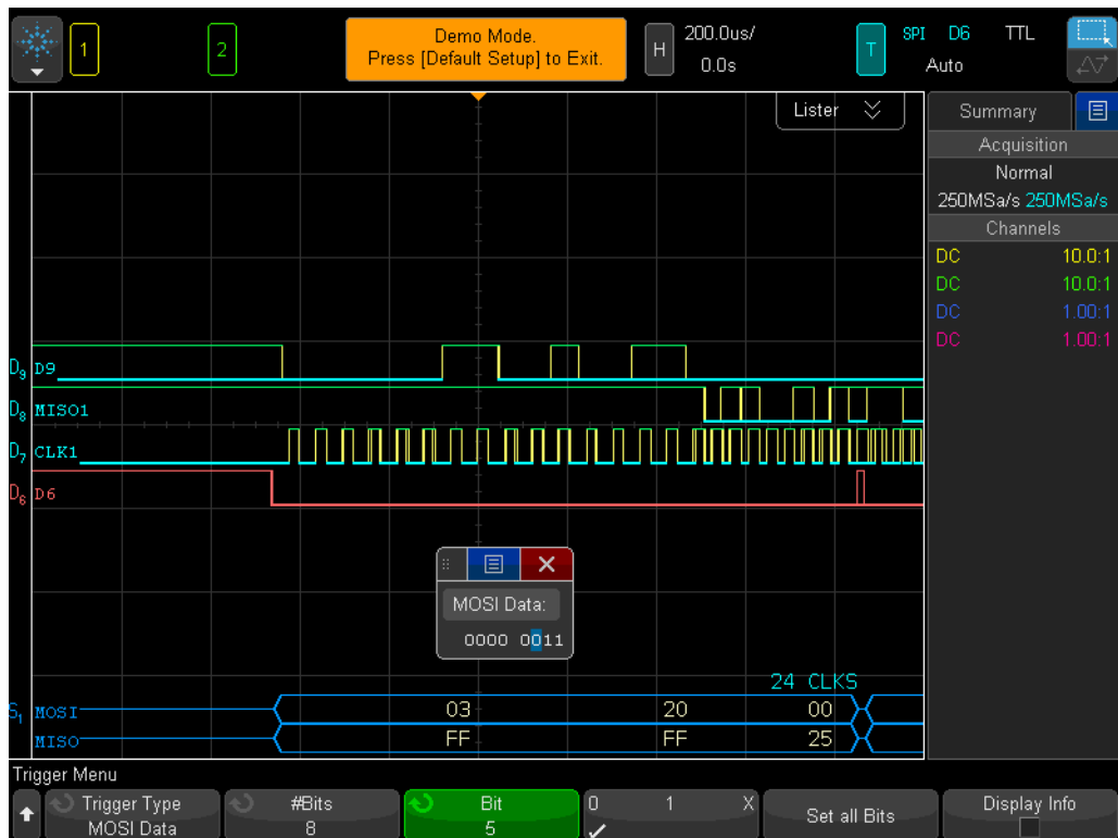
Figure 57 Triggering on MOSI data = 03 HEX .
