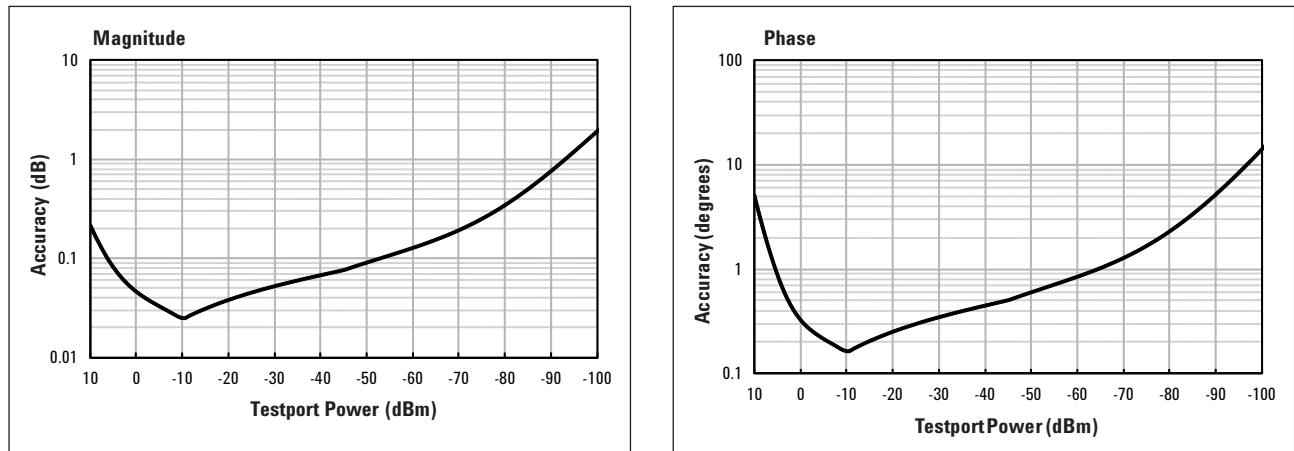
Figure 10. Dynamic Accuracy
