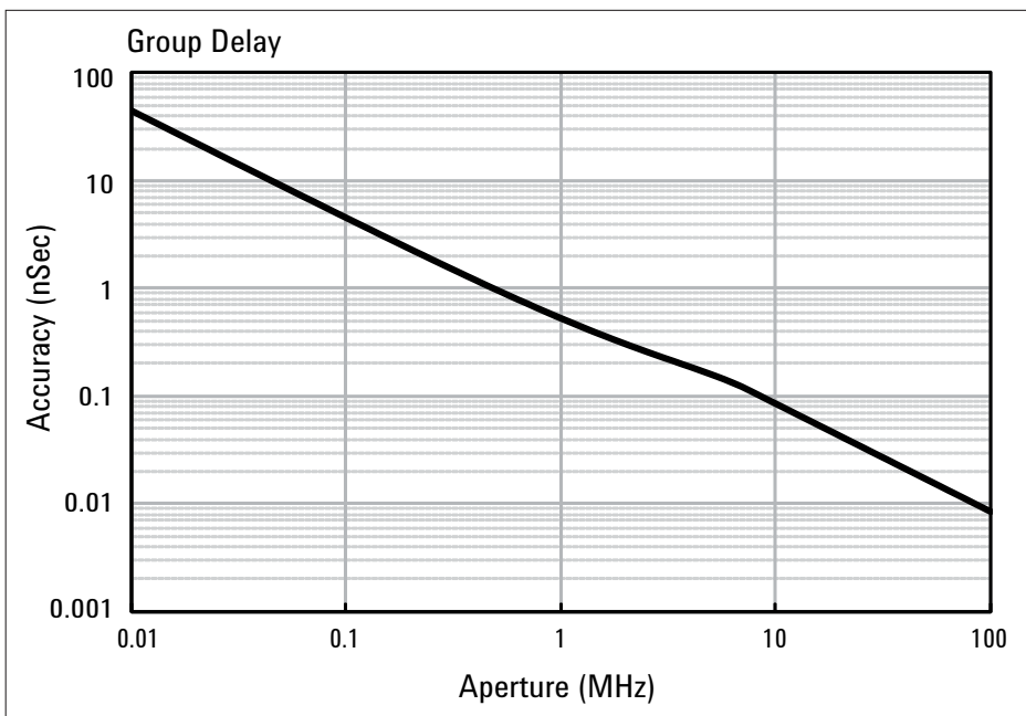
Figure 11. Group delay
