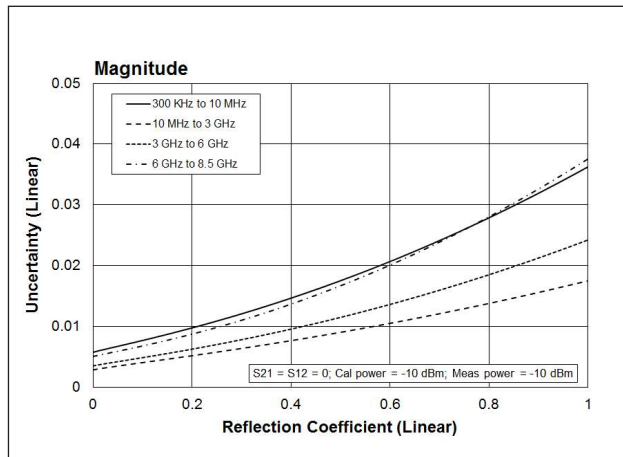
Figure 9. Reflection uncertainty (Specification)
