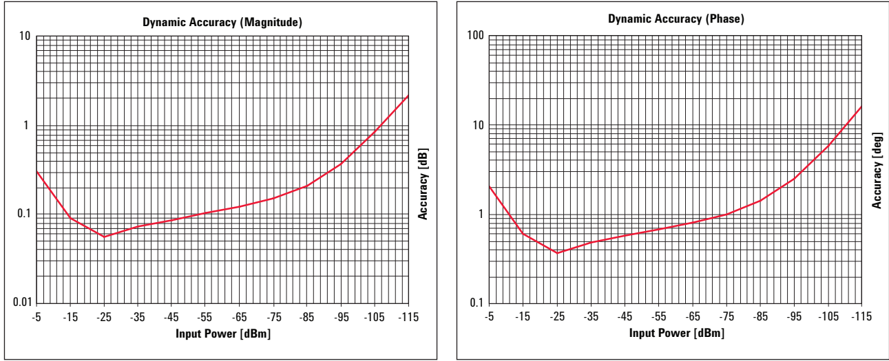
Figure 20. Dynamic Accuracy
