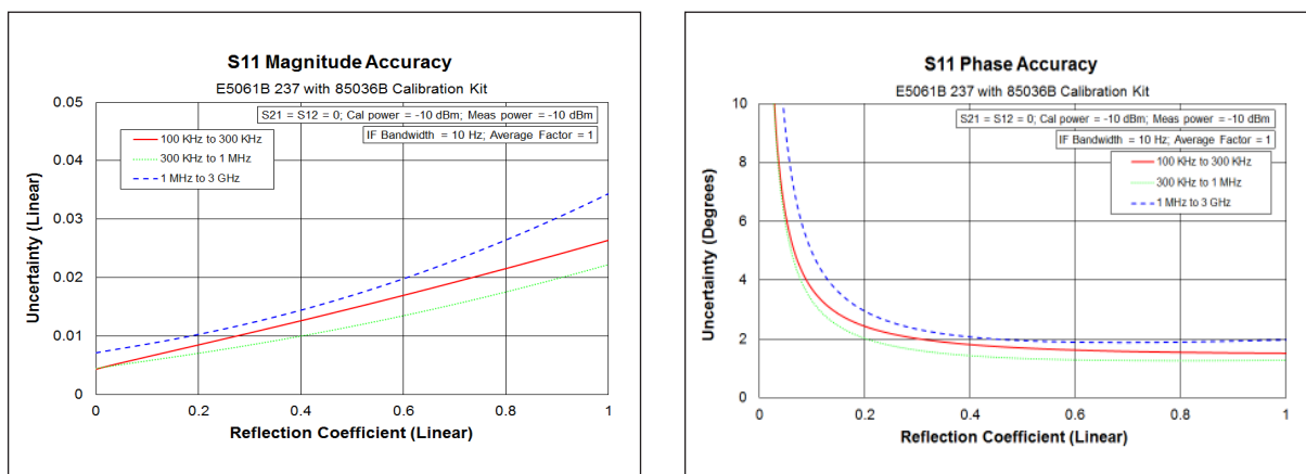
Figure 14. Reflection uncertainty (specification)
