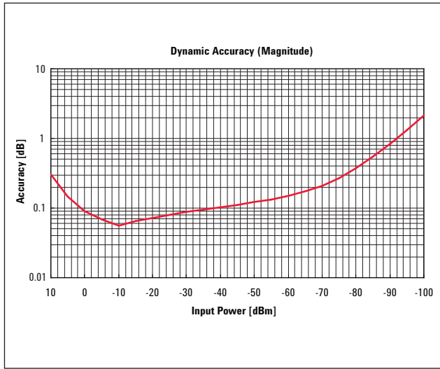
Figure 17. Dynamic Accuracy Option 3L5
