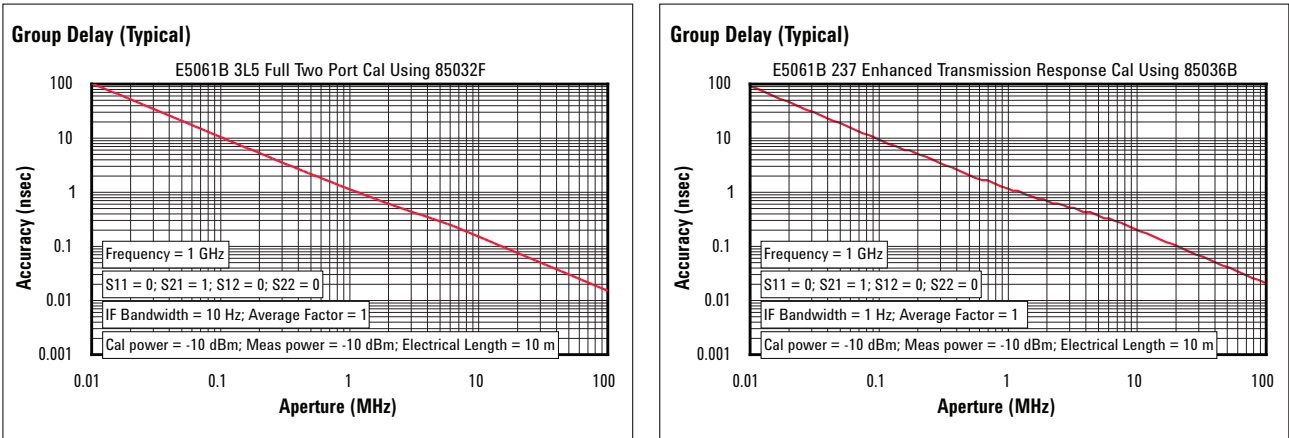
Figure 19. Group delay (typical)
