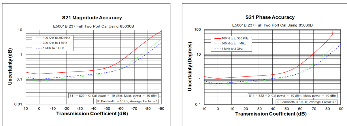
Figure 13. Transmission uncertainty (specification)
