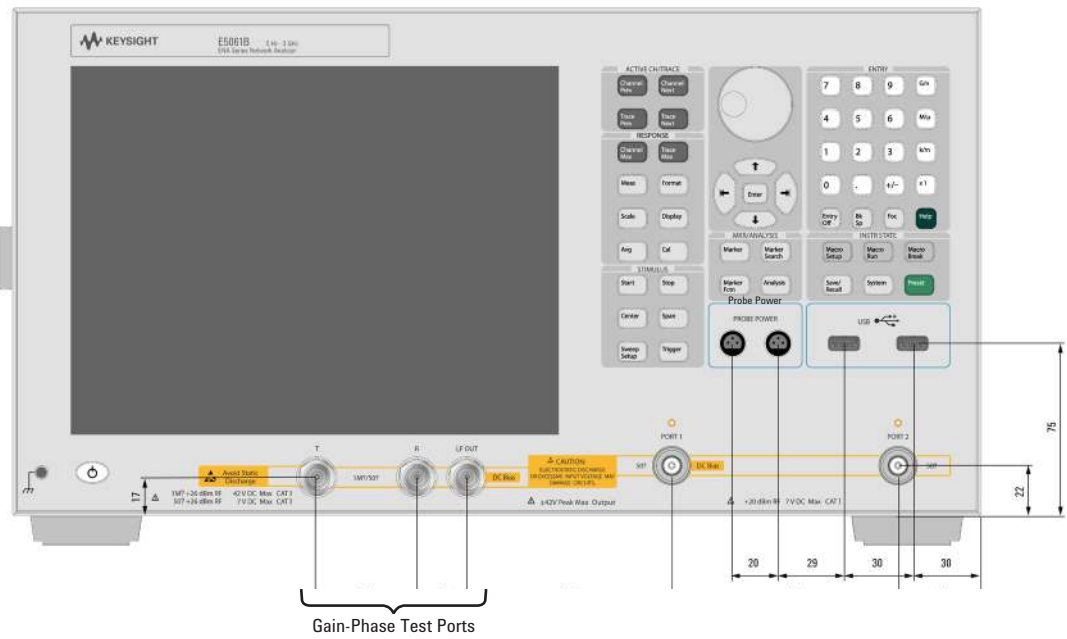
Figure 21. Dimensions (front view, in millimeters) 1
