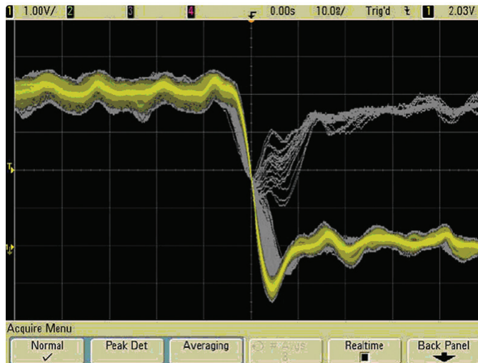
Figure 19. An infrequent glitch caught on a Keysight InfiniVision 6000 Series oscilloscope
