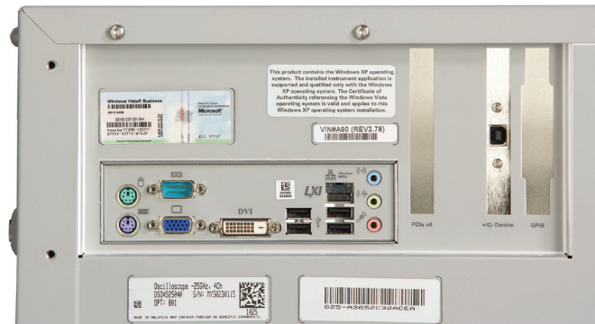
Figure 9. Rear panel on the Keysight Infinium 9000 Series oscilloscope
