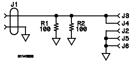
01148800 Test Board Schematic
