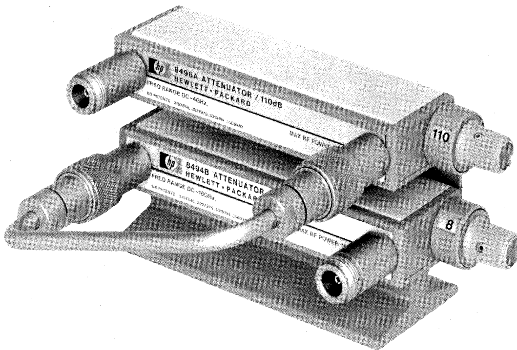
Figure 1 Typical Installation
