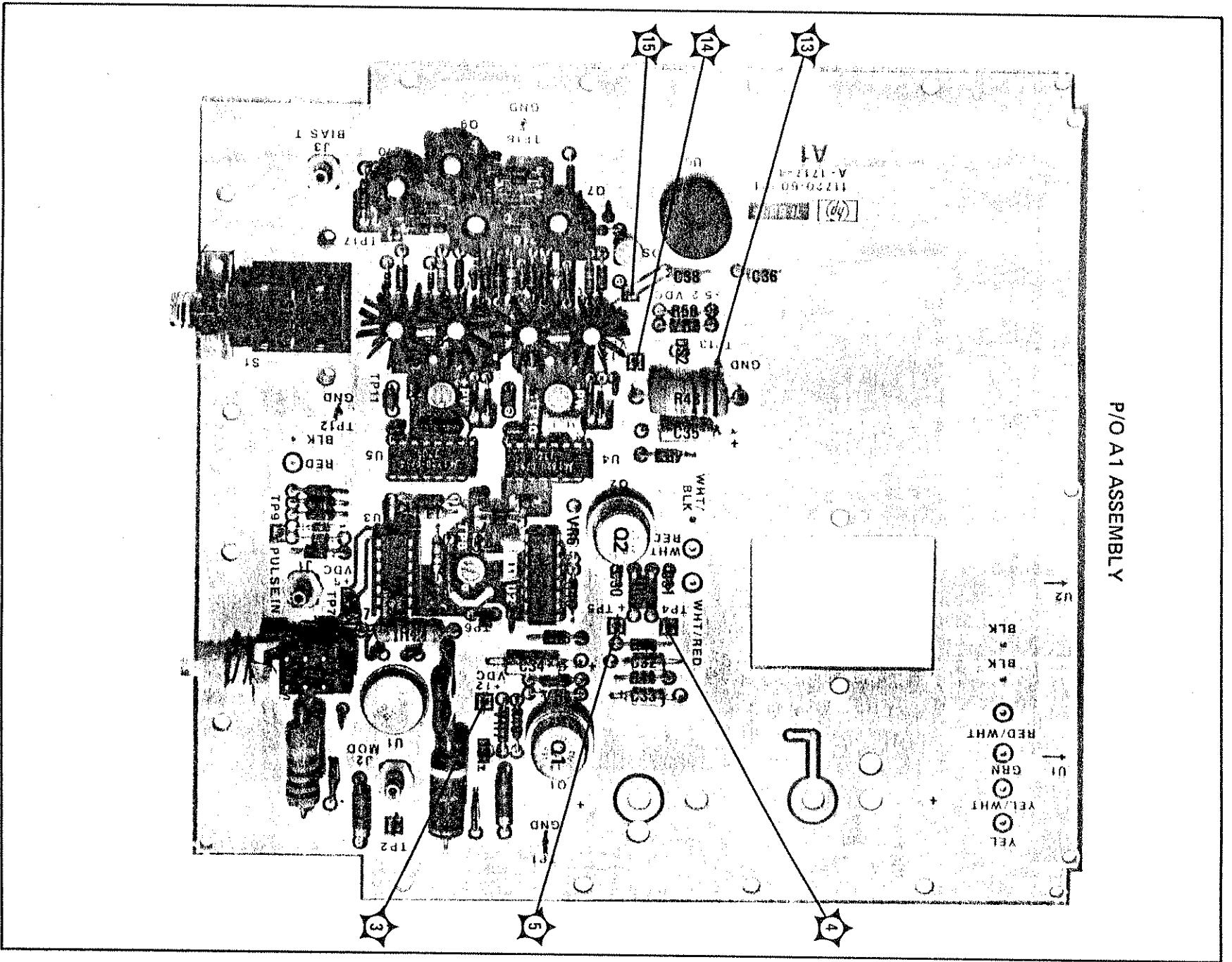
Figure 20. P/O A1 Pulse Driver Board Assembly Component Locations
