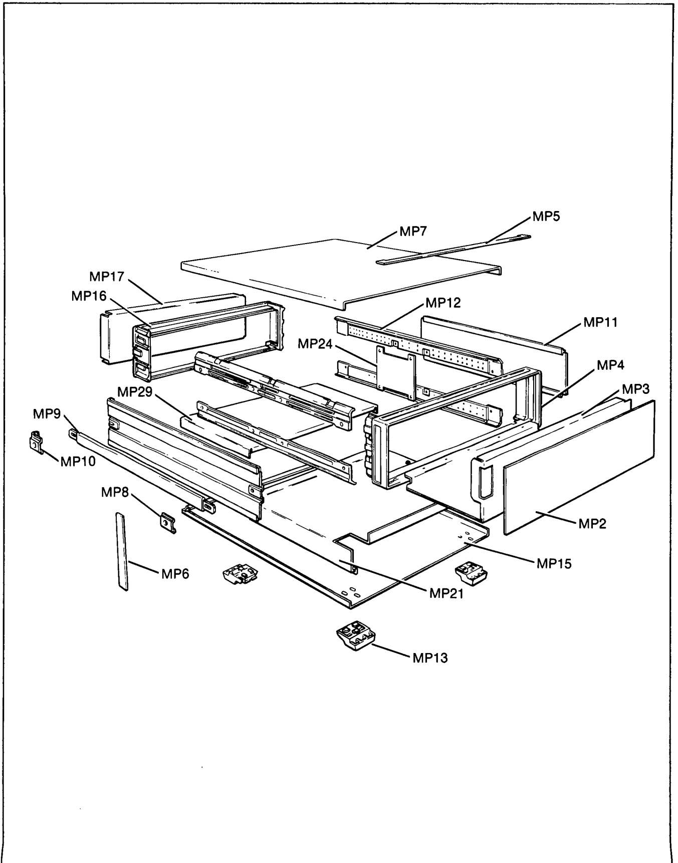
Figure 6. Cabinet Parts
