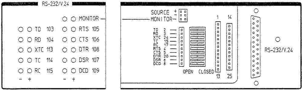
V.24 Front Panel Layout
