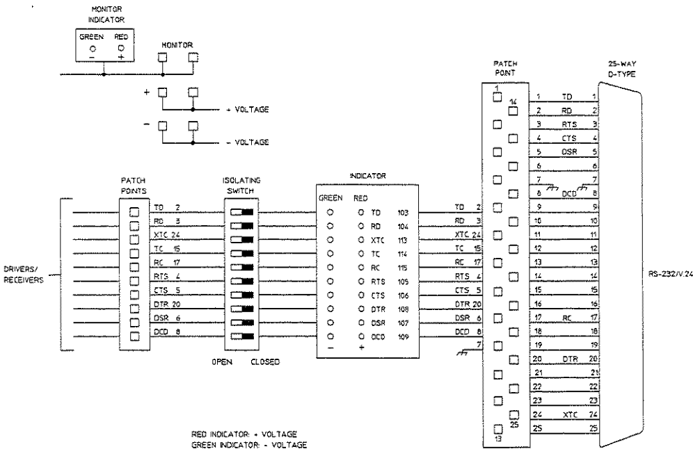
V.24 Functional Layout
