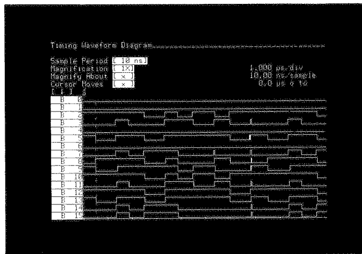
Figure 5-6. Triggering on a Timing Event
