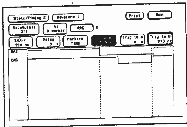
Figure 7-11. Time X to O
