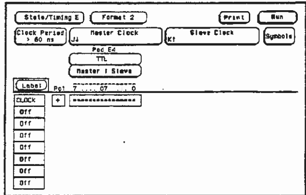
Figure 5-27. Master Clock and Slave Clock
