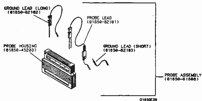
Figure 2-3. Probe Assembly
