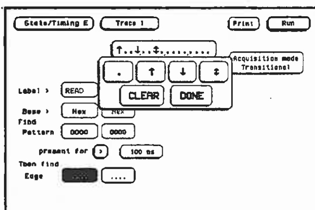
Figure 5-44. Combination of Edges Specified
