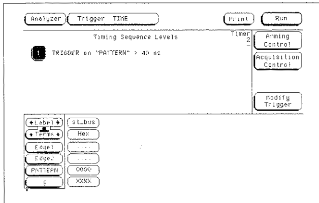
Triggering after lines have finished transitioning
