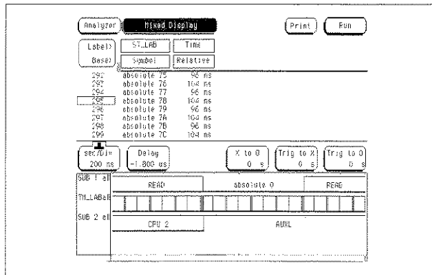
Mixed display using timing and state in the HP 1661C
