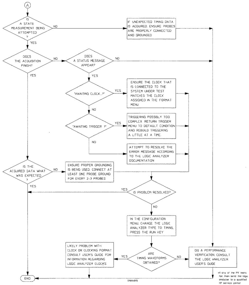
Troubleshooting Flowchart 2
