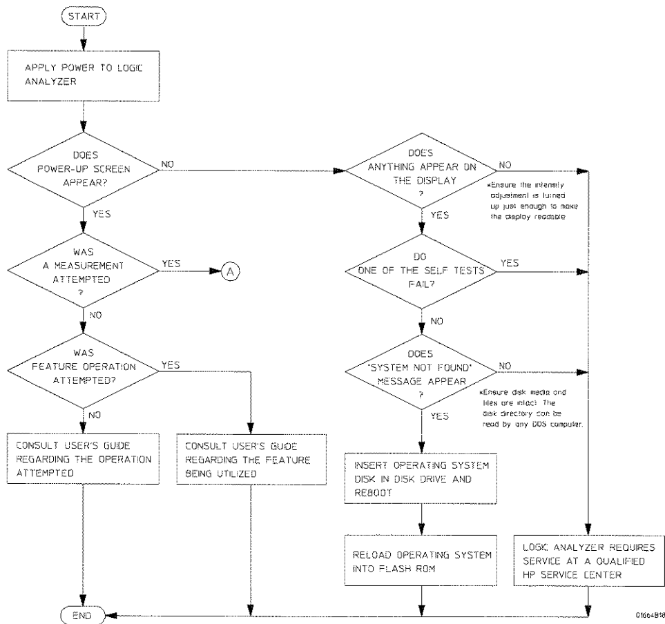
Troubleshooting Flowchart 1
