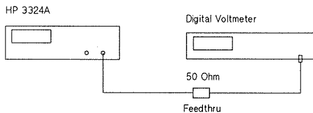
Figure 12-8. DC Offset Test Set-Up
