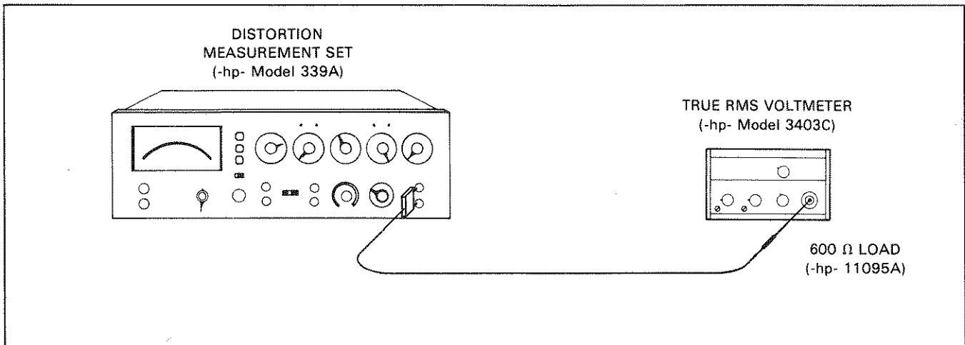
Figure 4-5. Oscillator Output Level and Flatness Test.
