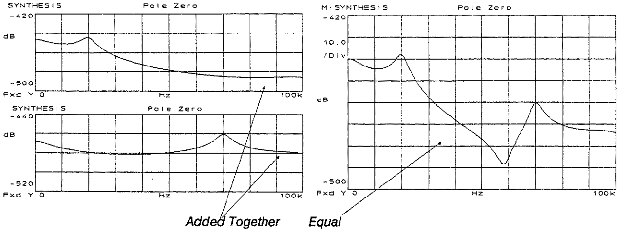
Figure 15-2. Addition
