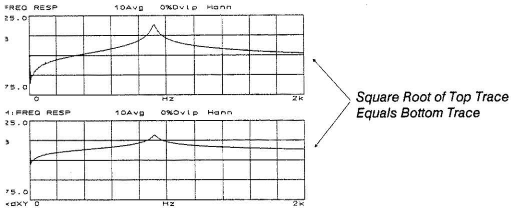
Figure 15-3. Square Root
