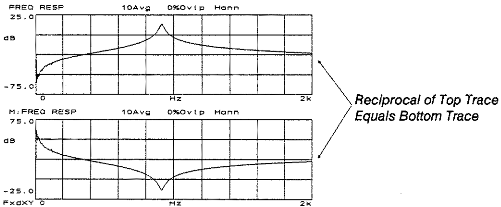
Figure 15-4. Reciprocation
