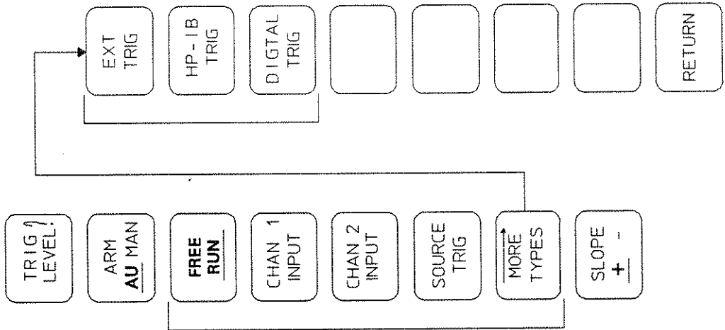
Select Trigger Menu Diagram
