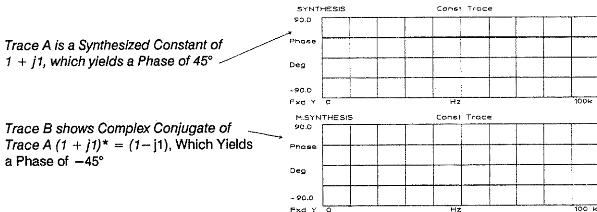
Figure 15-13. Complex Conjugation
