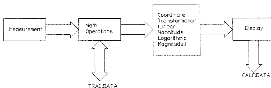
Figure 29-1. Flow of Measurement Data in the HP 35665A
