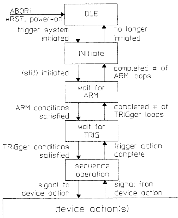
Figure 30-1. The HP 35665A's ARM-INITiate-TRIGger Functions
