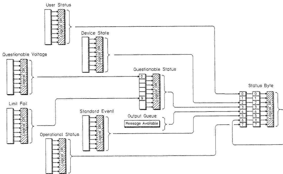
Figure 6-4. HP 35665A Register Sets
