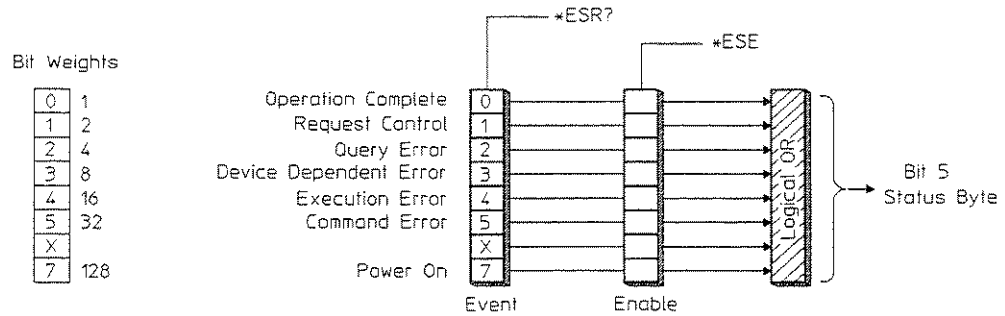
Figure 6-10. The Standard Event Register Set
