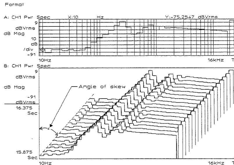
Figure 14-2. Waterfall traces displayed at 45° angle of skew
