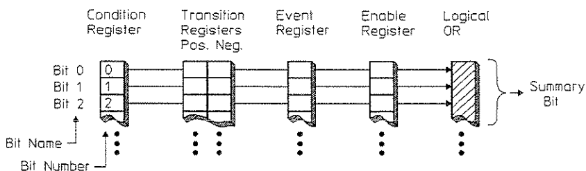
Figure 6-1. General Status Register Model
