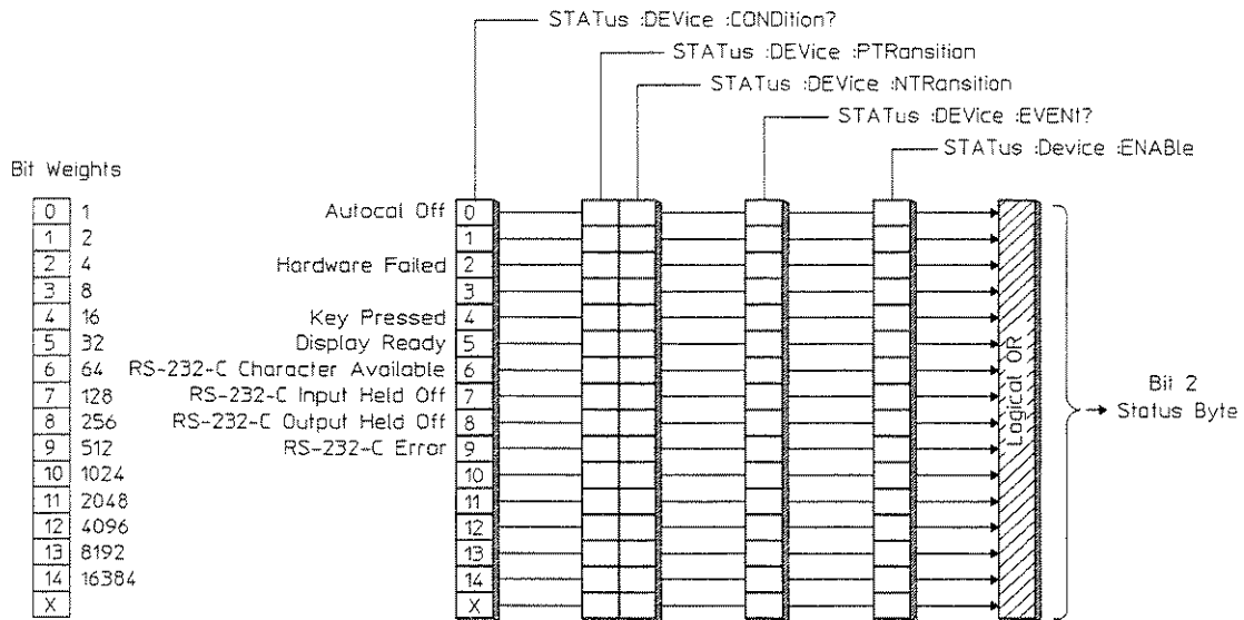
Figure 6-6. The Device State Register Set
