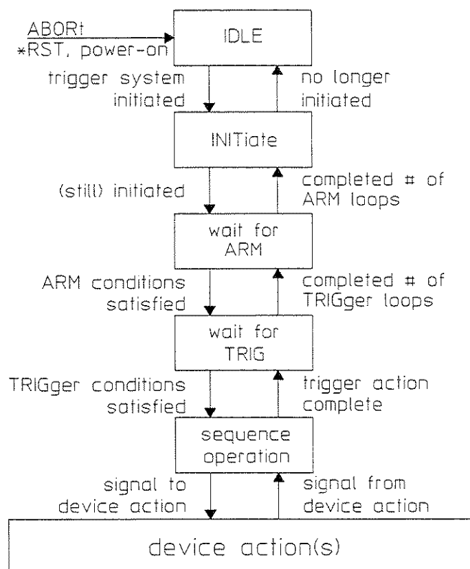
Figure 17-1. The HP 35665A's ARM-INITiate-TRIGger Functions
