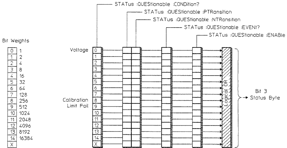
Figure 6-8. The Questionable Status Register Set
