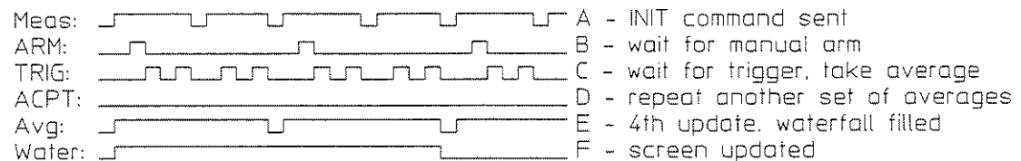
Figure 24-1. Transition of Operational Status Condition Register When AVERAge[:STATE] ON
