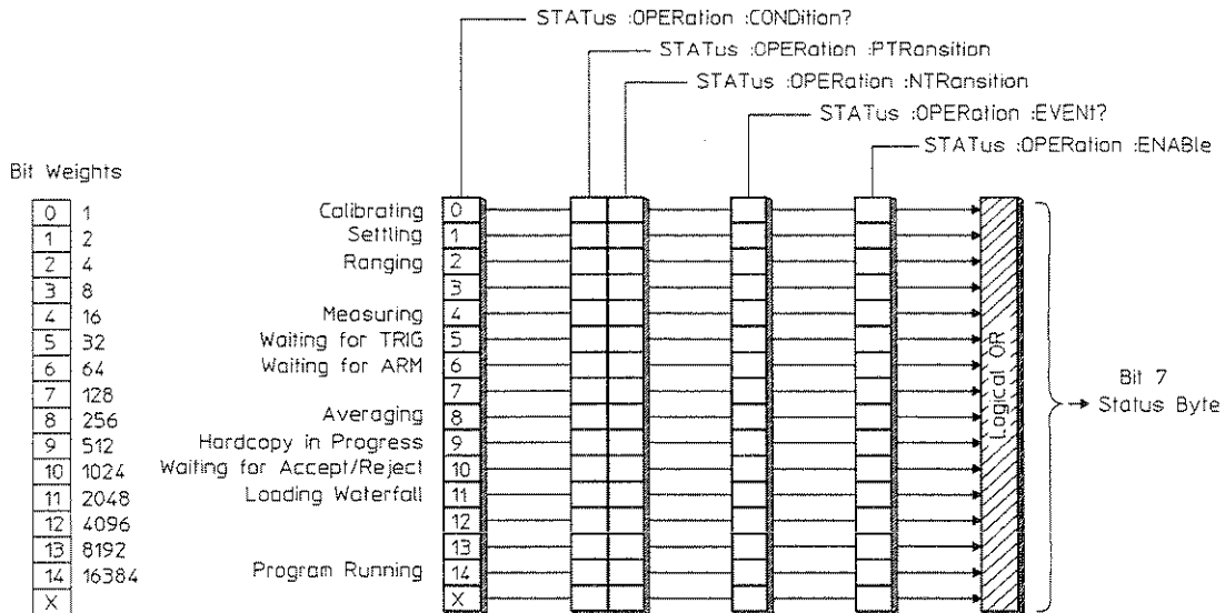
Figure 6-11. The Operational Status Register Set
