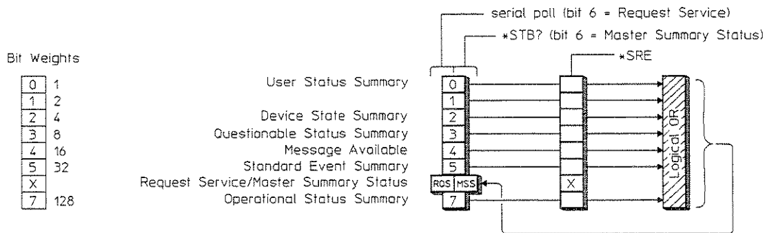
Figure 6-5. The Status Byte Register Set
