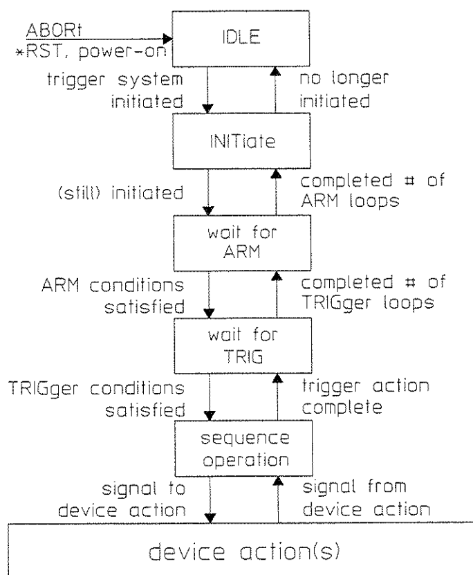
Figure 11-1. The ARM-INITiate-TRIGger Functions
