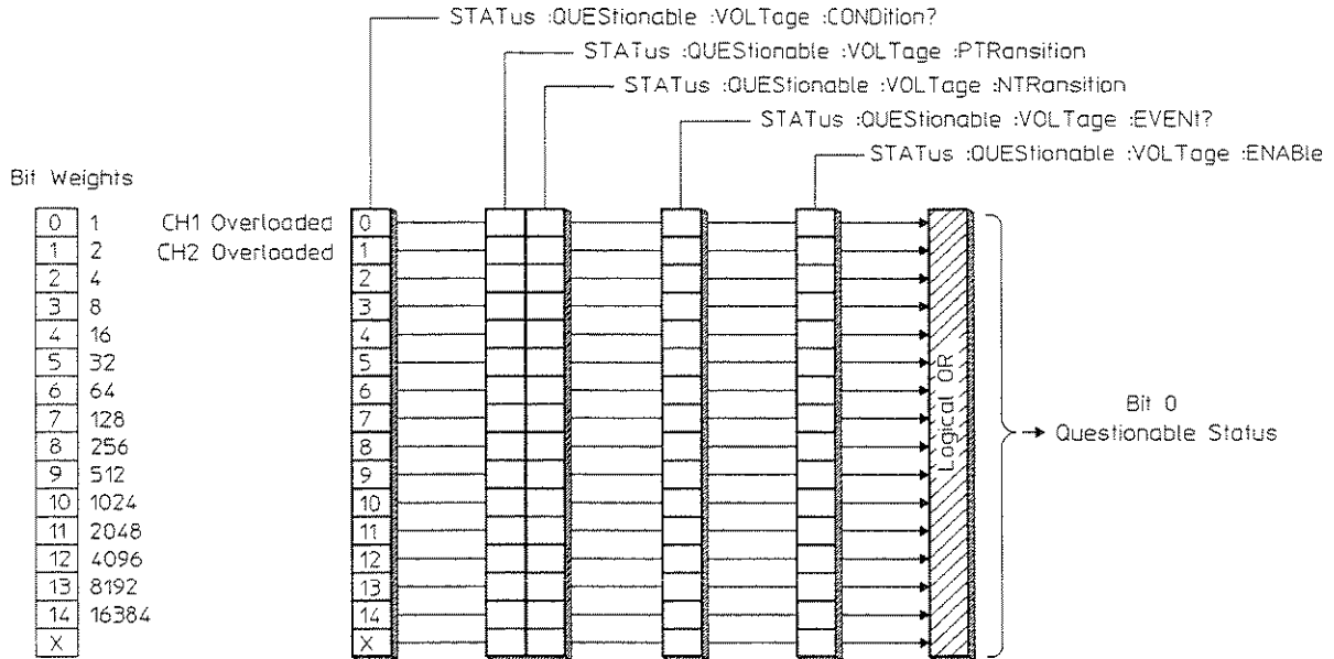
Figure 6-9. The Questionable Voltage Register Set
