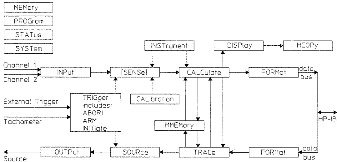
8-2. HP 35665A Measurement and Signal Flow
