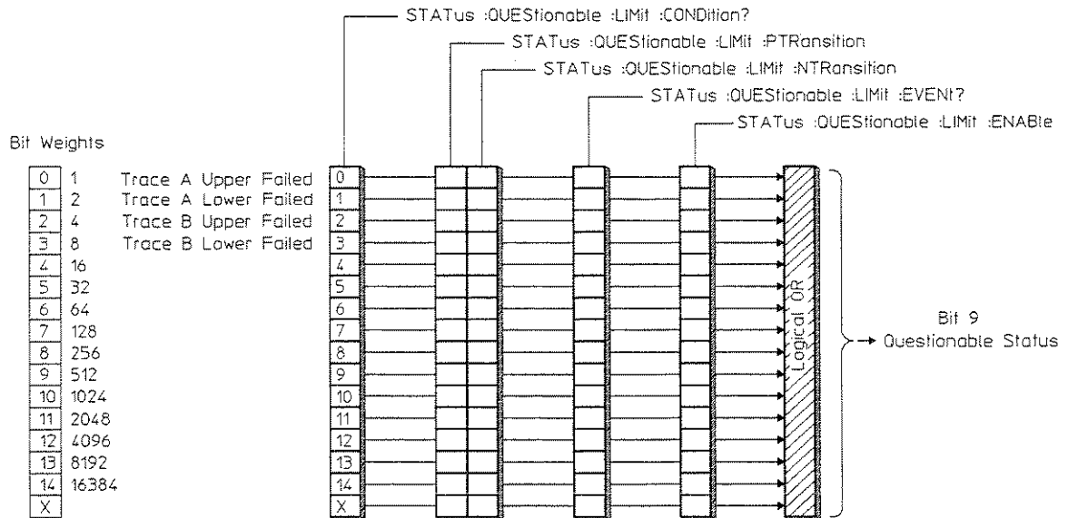
Figure 6-7. The Limit Fail Register Set
