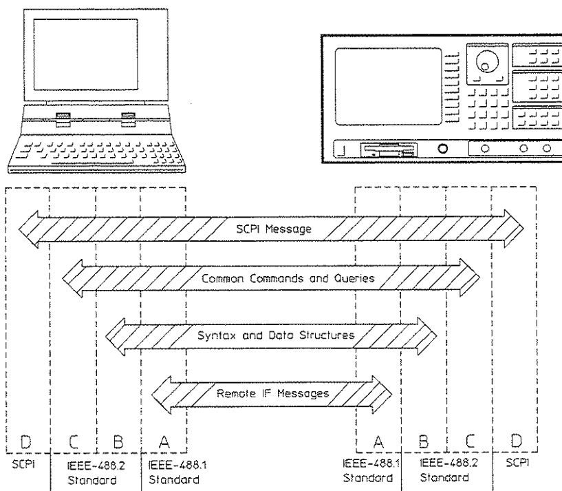
Figure 2-1. SCPI and Related Standards
