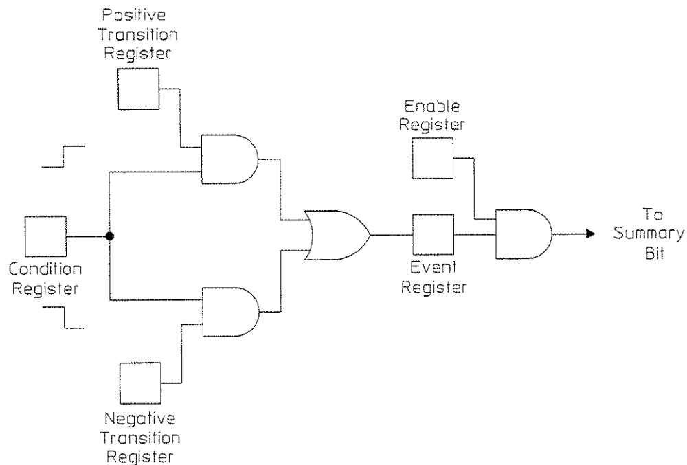
Figure 6-2. Flow of Information Within a Register Set
