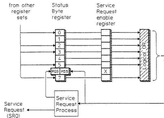
Figure 6-3. Generating a Service Request
