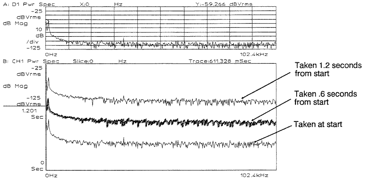
Figure 11-2. Recorded Time of Triggered Event Referenced to Start Time
