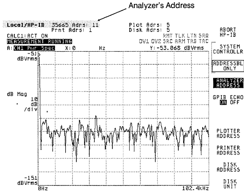
Figure 1-3. HP 35665A Screen After Pressing Local/HP-IB
