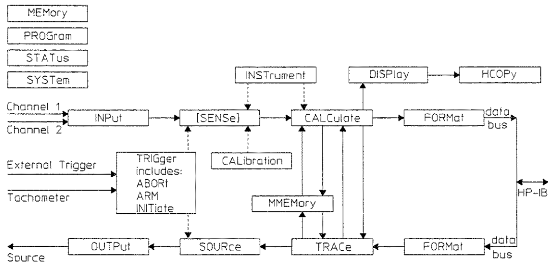
Figure 4-1. Measurement and Data Flow of the HP 35665A
