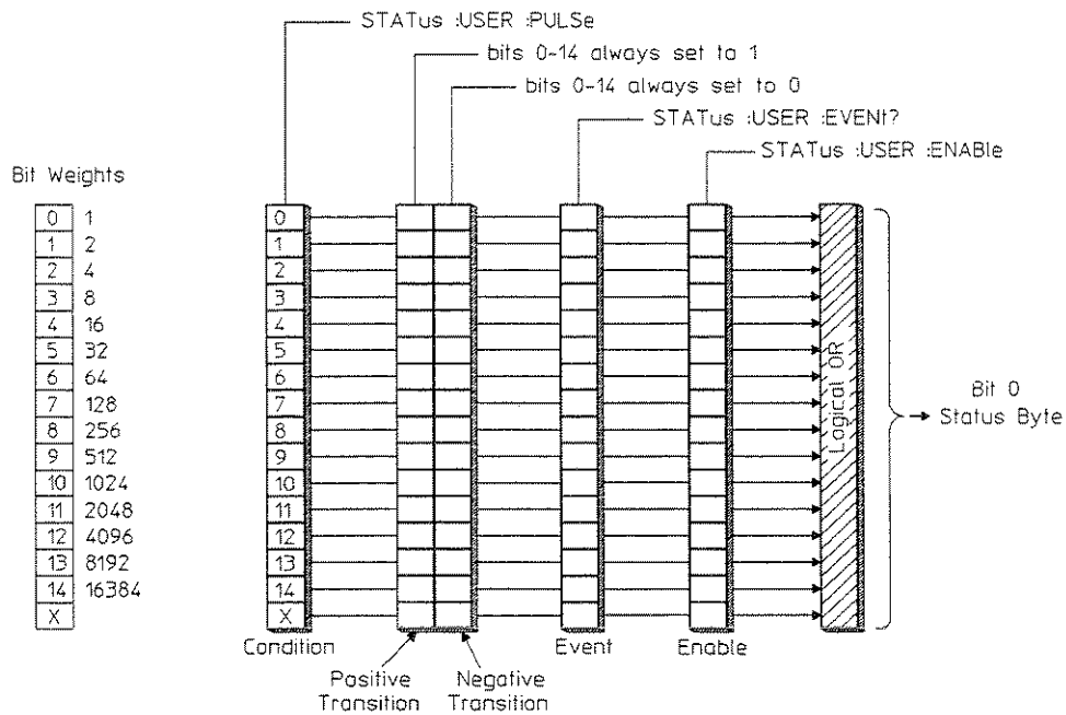
Figure 6-12. The User Status Register Set
