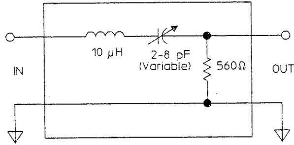
20 MHz Bandpass Filter
