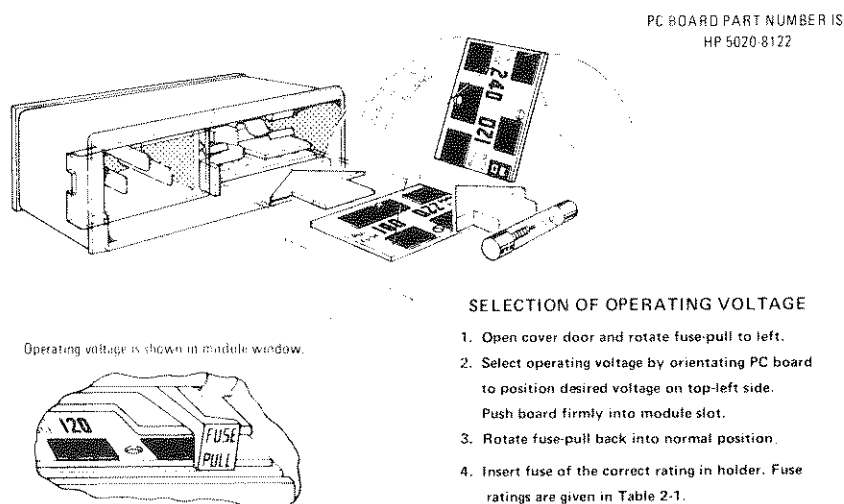
Figure 2-1 Line Selector
