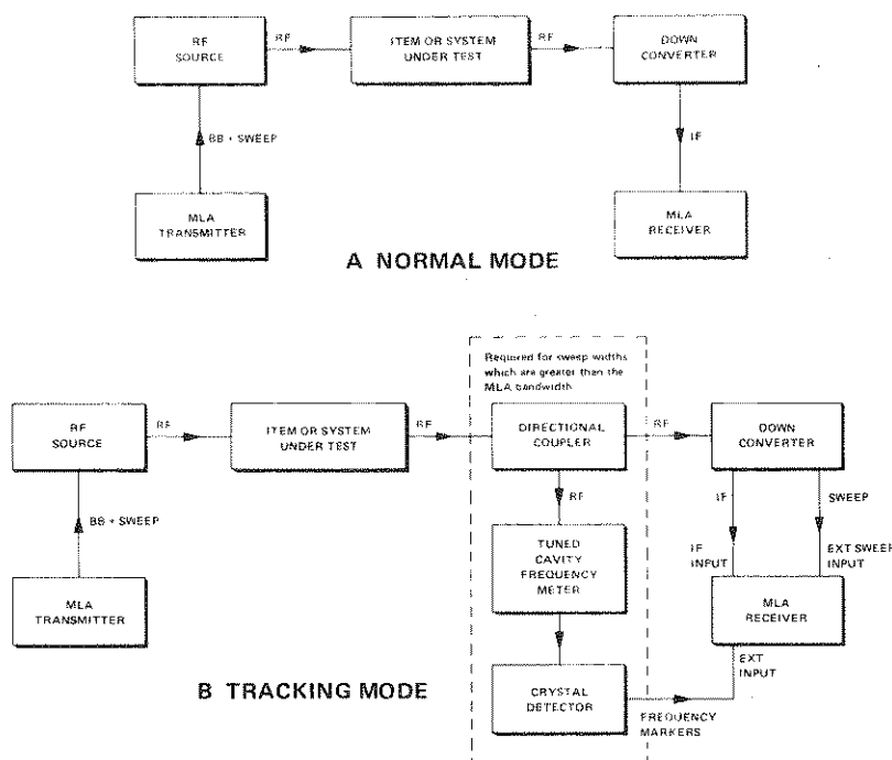
Figure 3-2 Typical Test Systems
