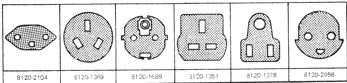
Figure 2-2 Power Cable Part Numbers/Power Receptacles
