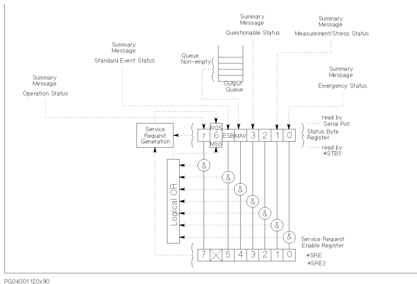
Figure 3-1 Status Reporting Structure
