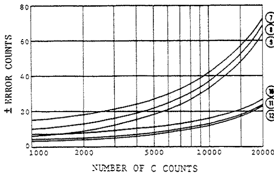
Figure 3-15. Measurement Accuracies (sheet 1 of 9).
