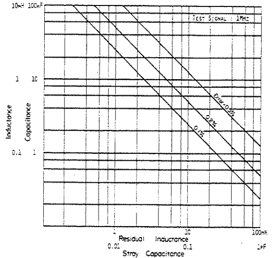
Figure 3-9. Relationships of Residual Parameters on Additional Errors.
