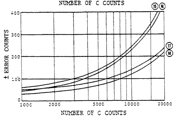
Figure 3-15. Measurement Accuracies (sheet 1 of 9).
