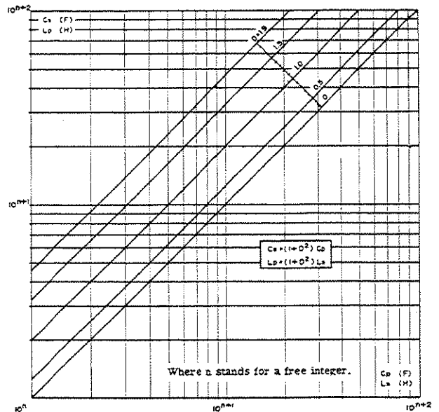
Figure 3-3. Parallel and Series Parameter Relationships.
