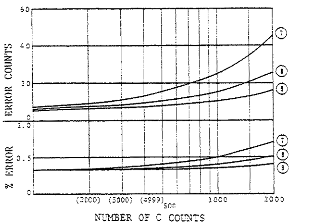
Figure 3-15. Measurement Accuracies (sheet 2 of 9).
