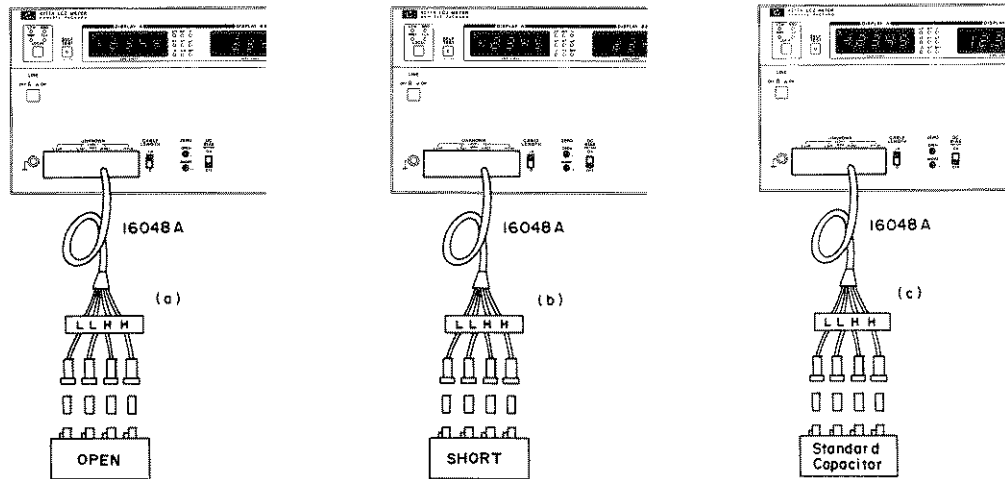
Figure 4-5. Capacitance Accuracy Test Setups (CABLE LENGTH: 1m).
