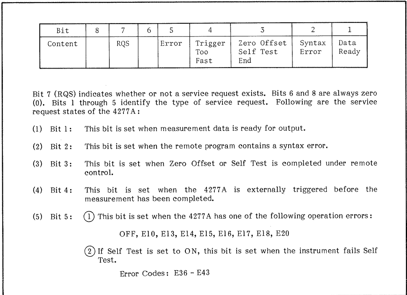
Figure 3-26. Status Byte for the 4277A.
