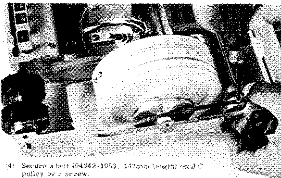
Figure 5-10. AC Dial Restringing.
