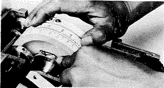
(1) Hook one end of the string (04342-8541, 620mm length) to the free end of the spring on Main Capacitor Drum Scale Pulley.
