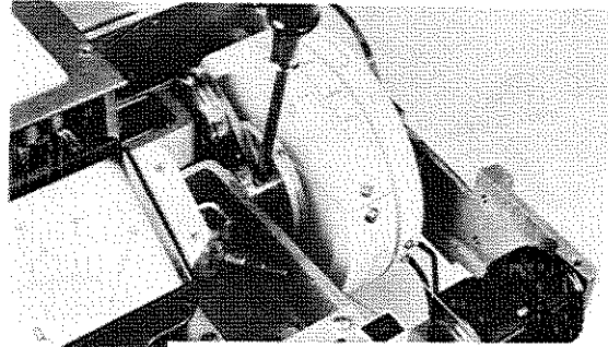
(5) Secure the other end of the belt to the Drum Scale Pulley by a screw, which should not be tightened.
