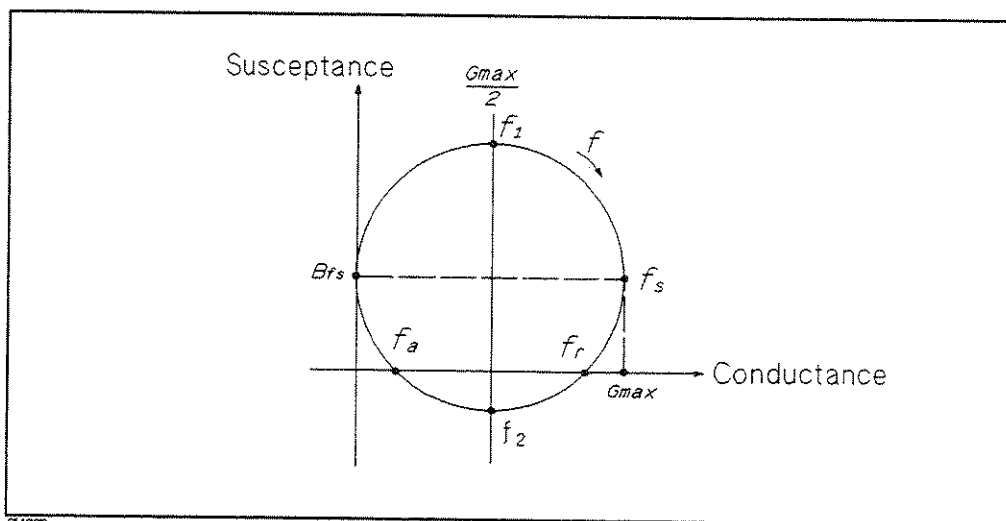
Figure I-19. Admittance Characteristic Circle Diagram
