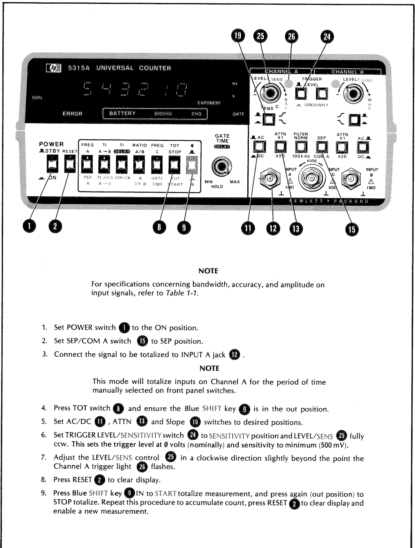
Figure 3-20. Totalize Measurement
