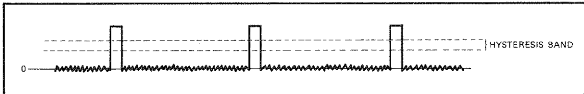
Figure 3-11. DC Coupled Measurements
