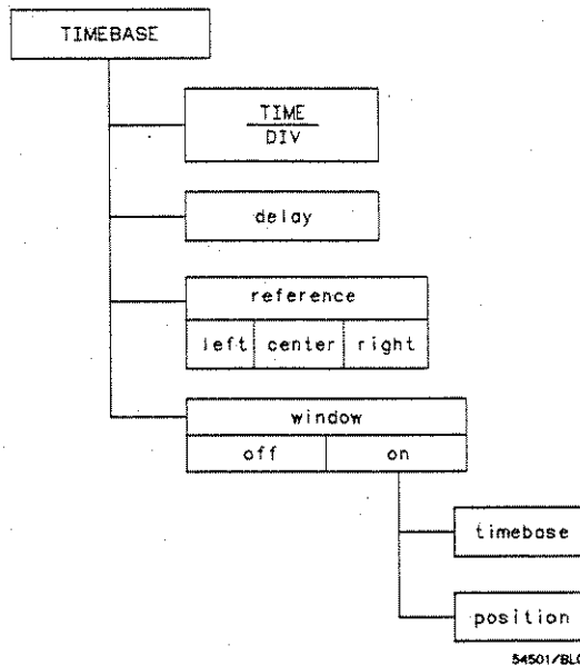
Figure 4-1. Timebase Menu.
