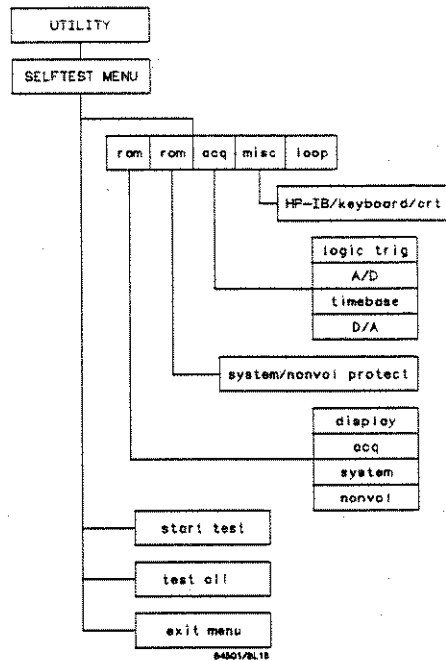
Figure 12-3. Self-Test Menu
