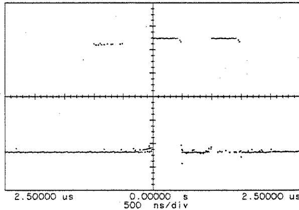
Figure 6-3. Two-Burst Pulse
