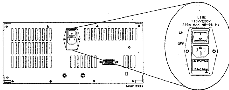
Figure 2-5. Line Switch
