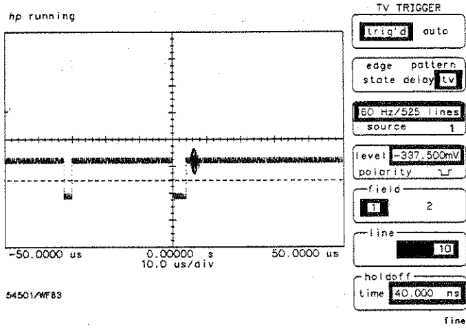
Figure 6-18. Trigger on Field 1, Line 10
