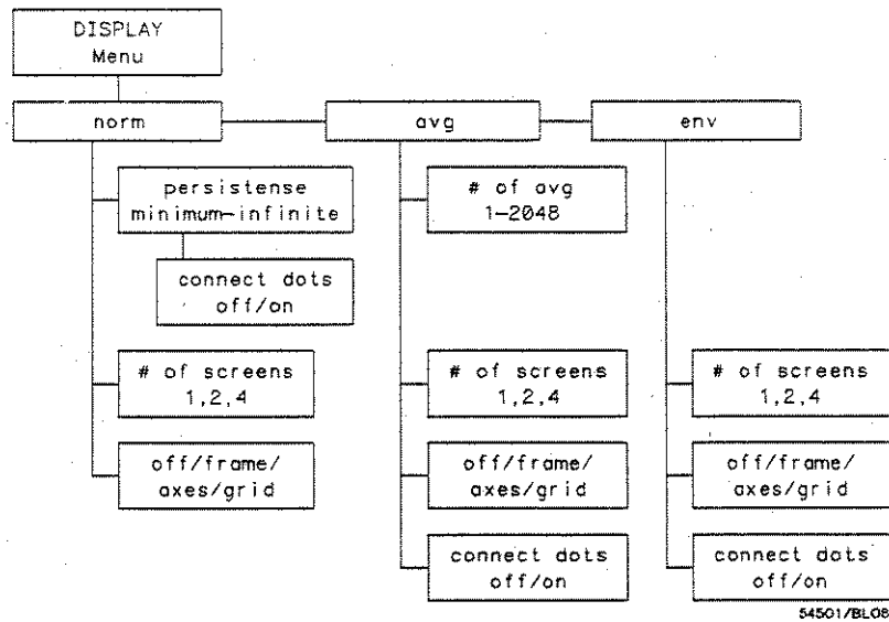
Figure 7-1. Display Menu
