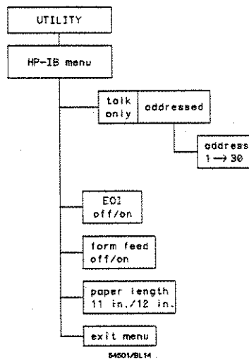
Figure 12-2. HP-IB Menu
