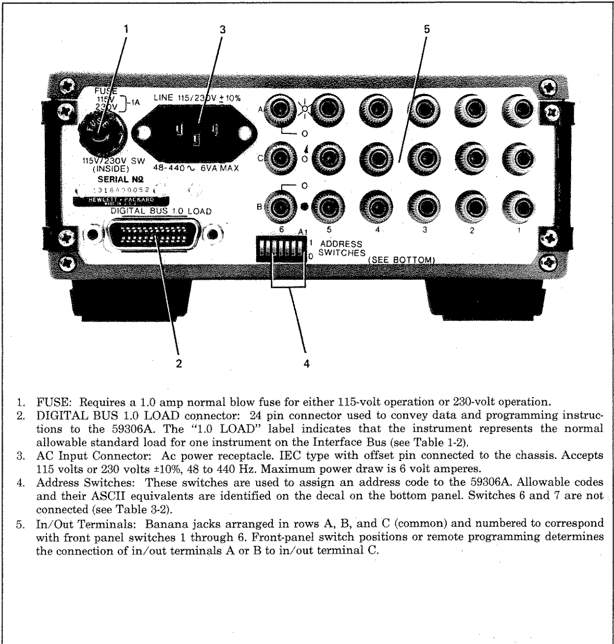
Figure 3-2. 59306A Relay Actuator Rear Panel
