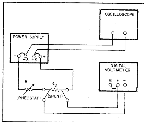
Figure 5-6. Current Limit Adjustment Setup
